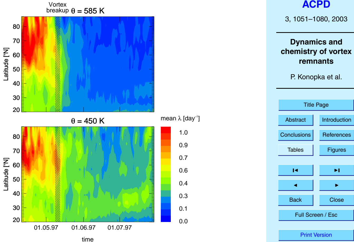
Fig. 6. Zonally averaged Lyapunov exponent \lambda during the 1997 period calculated over a time step \Delta t = 12 h at \theta = 450 and 585 K. Note that the summer circulation at 585 K is characterized by very low values of \lambda .
