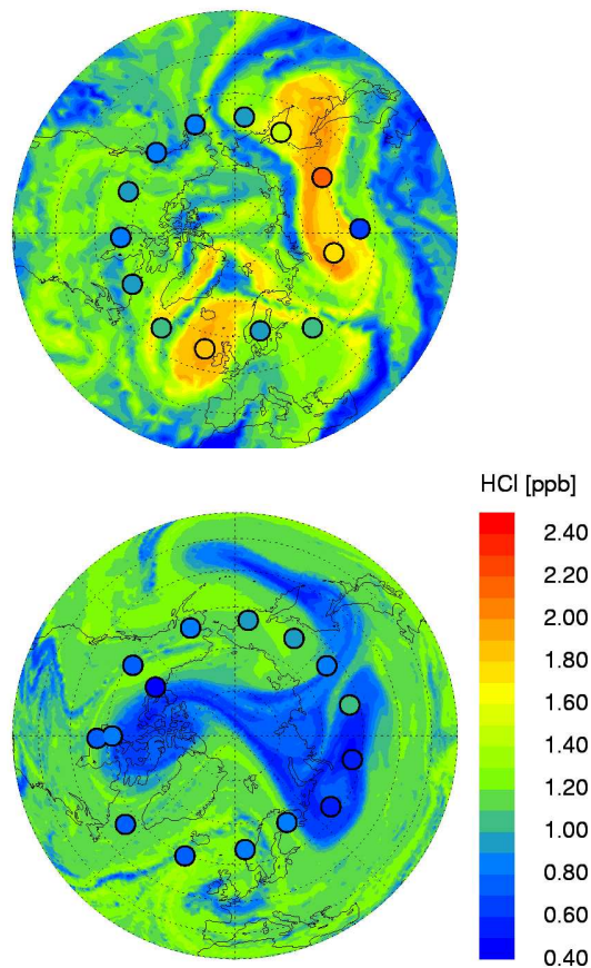
Fig. 8. HCl simulated with CLaMS at \theta = 450\text{K} 2 days after the vortex breakup at 12 May 1997 (top) and 17 March 2000 (bottom). High values of HCl indicate a completed chlorine deactivation. The circles denote the HALOE observations.
