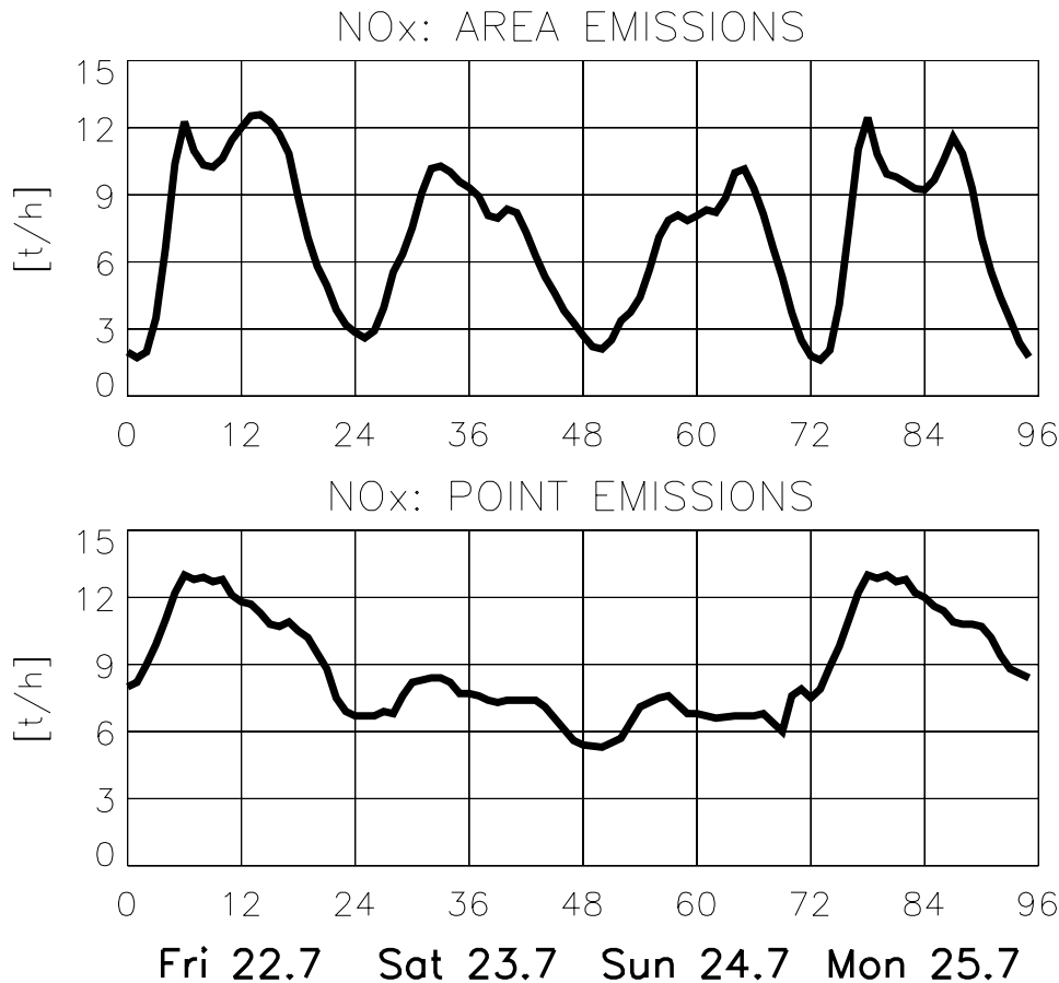
Fig. 4. Time series of NO x emission as sum of all area emission sources (upper panel) and point sources (lower panel) released into the domain between 22 and 25 July. The emissions are in units of [t/h].
