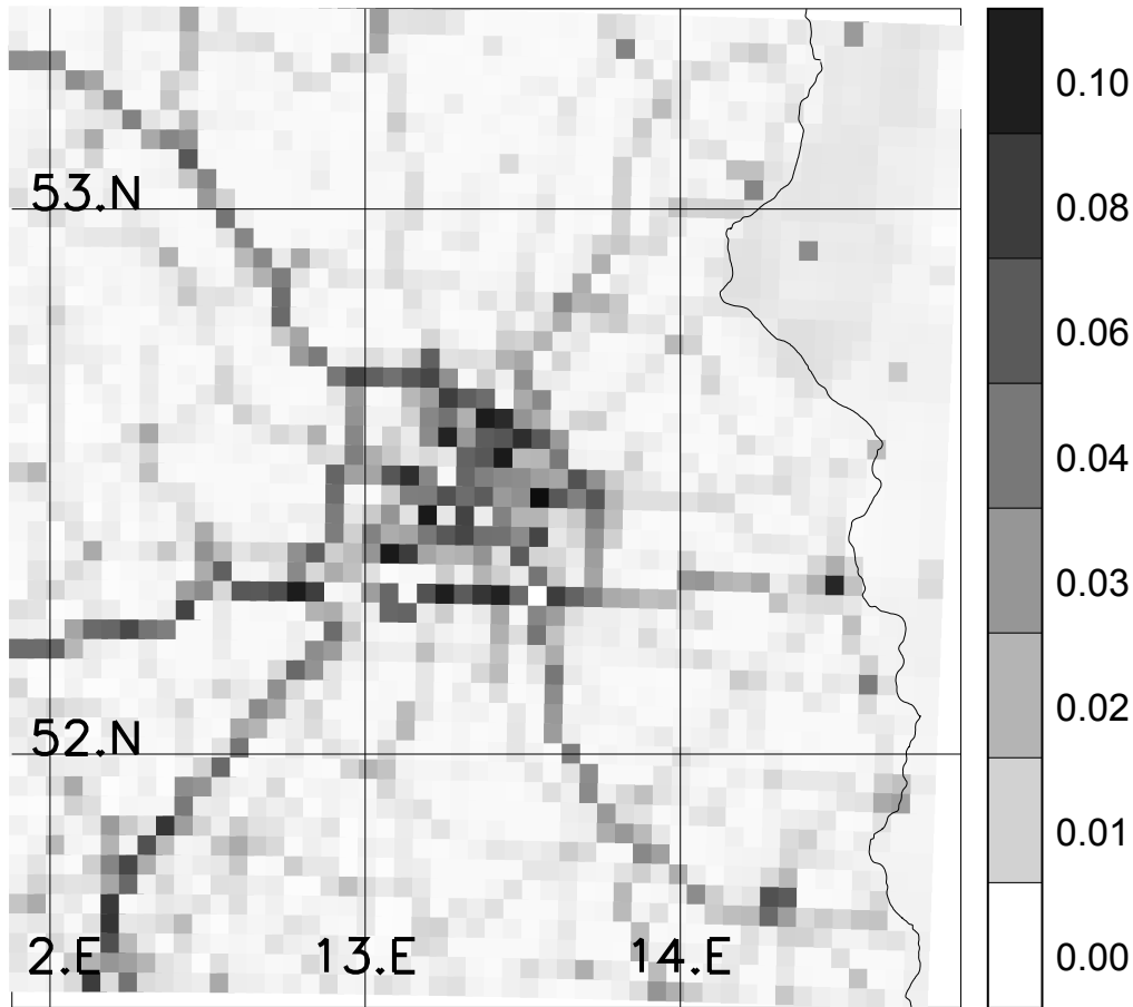
Fig. 3. \text{NO}_x emission on 25 July 1994 at 6:00 UTC. The emissions are in units of [t/h].
