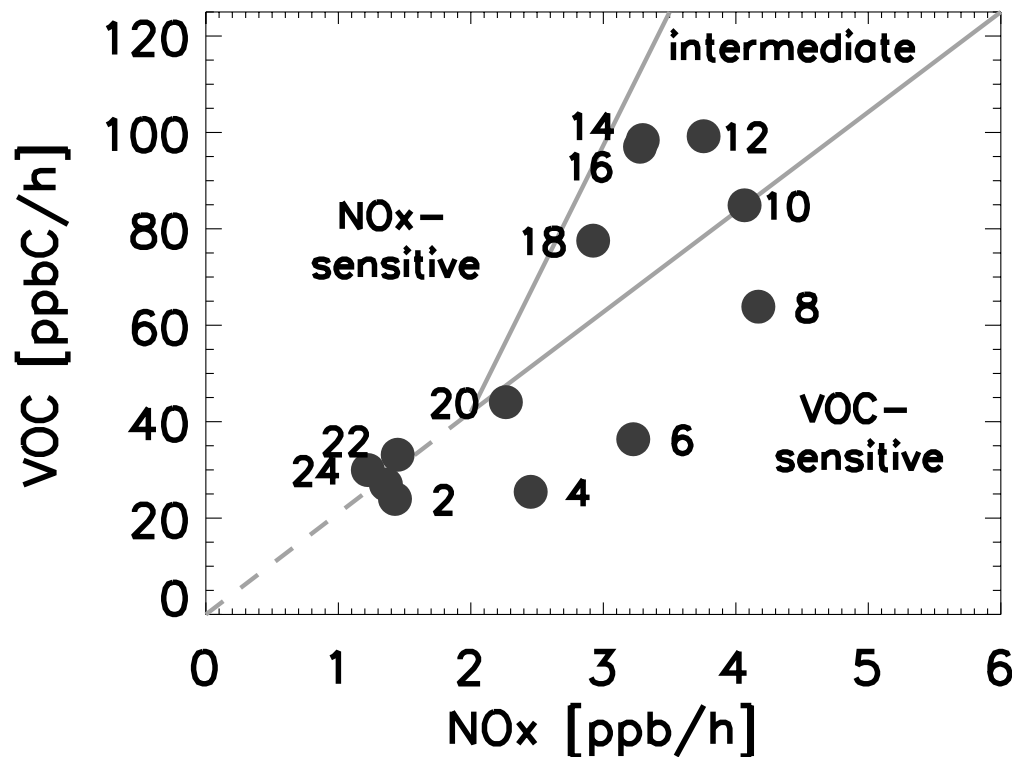
Fig. 10. Total emissions of VOC versus NO x . Emissions of the total domain are shown. The numbers mark the time of the day. The lines separate the VOC- and NO x -sensitive areas for ozone production.
