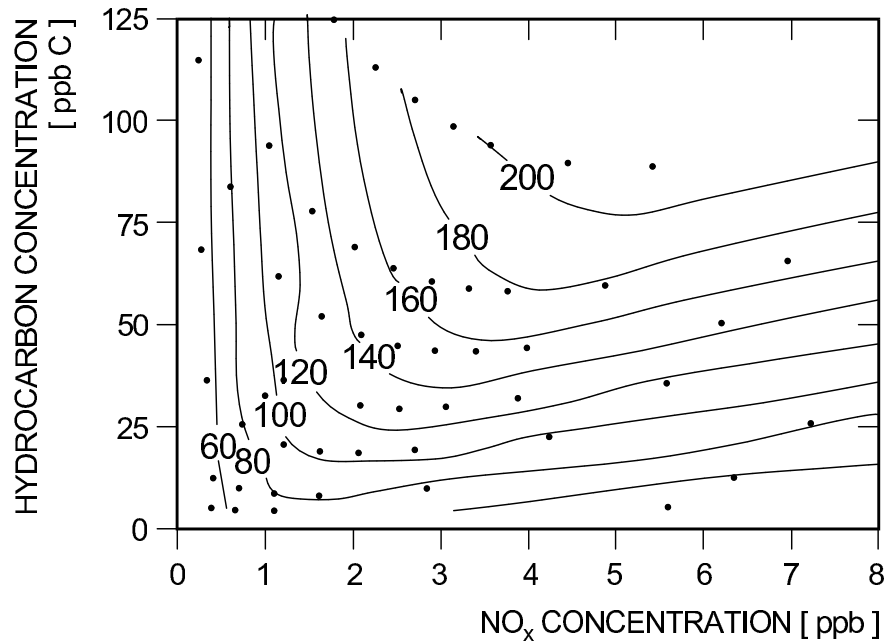
Fig. 9. Ozone in ppb v as function of the concentrations of NO x and VOC after Sillman et al. (1990). The dots refer to the simulations Sillman has done to calculate this figure.
