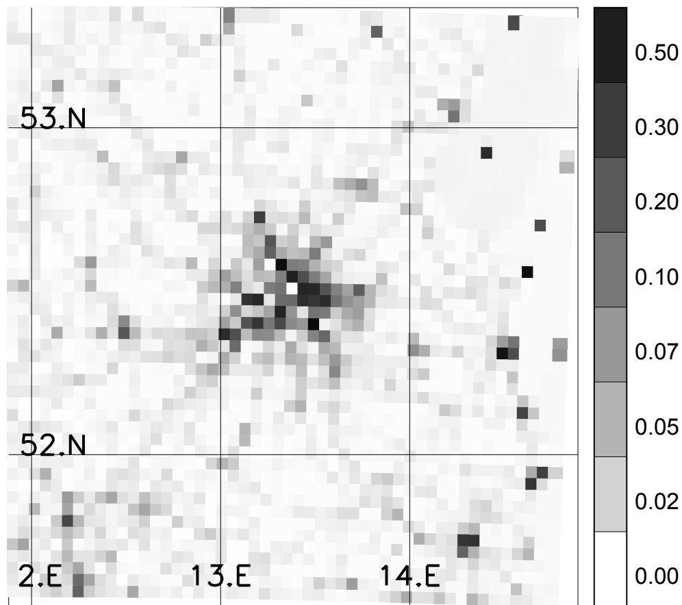
Fig. 5. Anthropogenic VOC emissions on 25 July at 6:00 UTC. The emissions are in units of [t/h].
