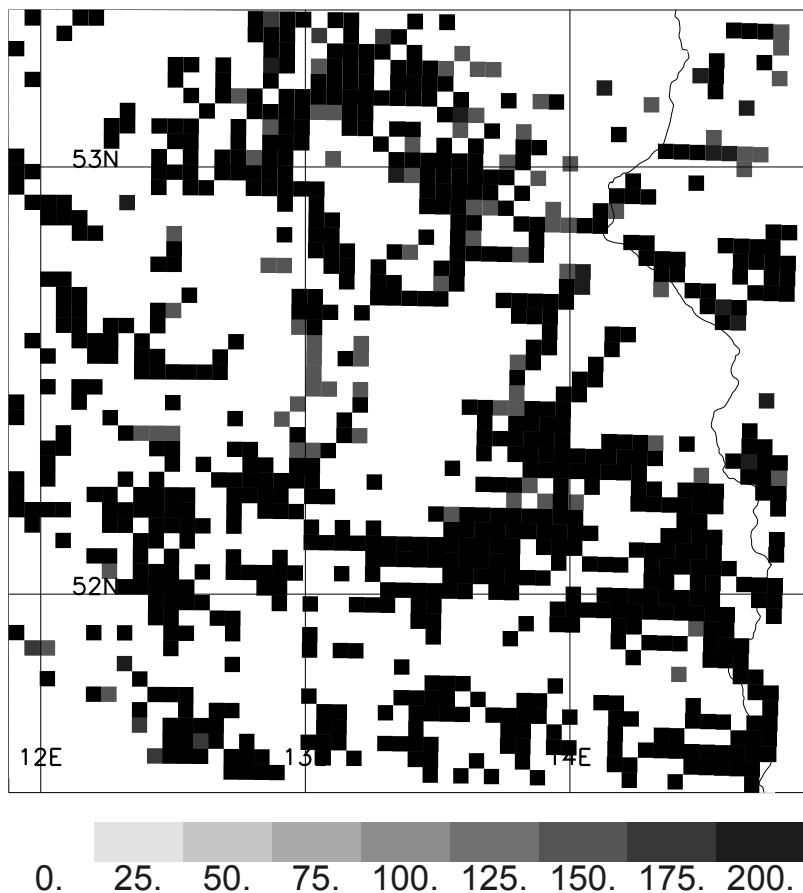
Fig. 7. Biogenic VOC emissions at 14:00 UTC on 23 July in \text{ppb}_v\text{C} per hour.
