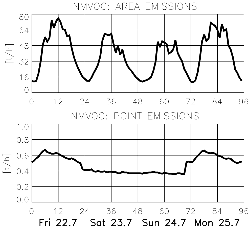
Fig. 6. Time series of VOC emission as sum of all area emission sources (upper panel) and point sources (lower panel) released into the domain between 22 and 25 July. The emissions are in units of [t/h].
