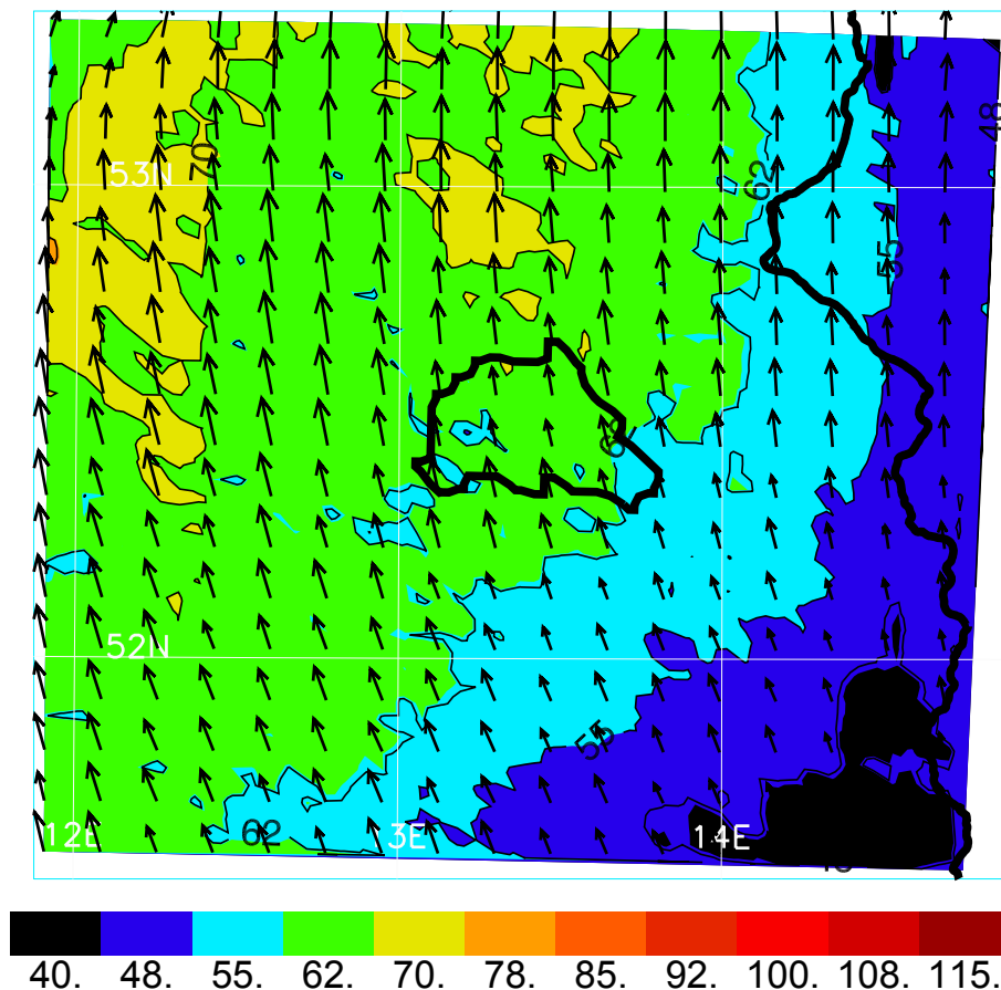
Fig. 1. Near surface ozone concentrations (ppb v ) and wind directions on July 23 at 14 UTC in Berlin-Brandenburg. Berlin and the border to Poland are marked in black, latitudes and longitudes in white. The model results are projected to this map.
