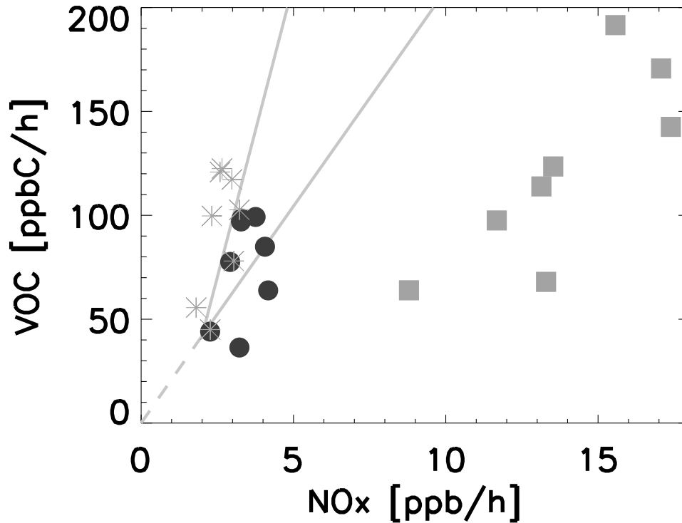
Fig. 12. Total emissions of VOC versus NO x in ppb v per hour and grid box area. Emissions representing the total domain (filled circles) and for rural (grey stars) and urban (grey squares) conditions are shown. The lines separate the VOC- and NO x -sensitive areas.
