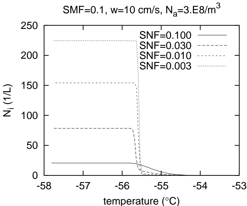
Fig. 1. Number density of ice crystals forming from internally mixed aerosol of sulfuric acid solution with soot inclusions in a uplifting and adiabatically cooling air mass as function of temperature (which may be considered a reverse time axis) as simulated in a box-model. Ice crystals form by heterogeneous and homogeneous nucleation. The simulations were performed with 10 cm/s uplift, with soot mass fraction SMF = 0.1 (of those aerosol droplets that bear an inclusion), total aerosol number density N_a = 3 \times 10^8 \text{ m}^{-3} , and with fraction of aerosol particles bearing an inclusion, SNF , as indicated on the figure. Homogeneous nucleation is signalled by the steep increase of N_i with decreasing temperature.
