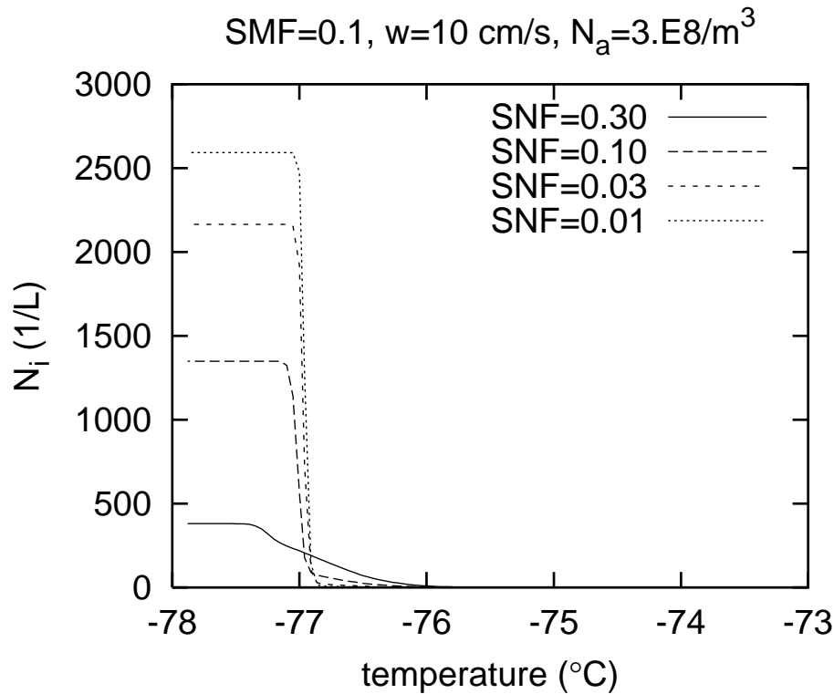
Fig. 2. As Fig. 1, but computed with initial temperature of -73^{\circ} C and initial relative humidity RH = 50\% .
