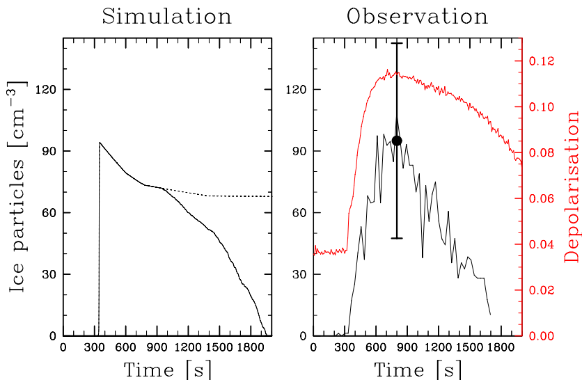
Fig. 7. Total ice particle number densities versus time (modeled values on the left panel, measured values on the right panel). The simulation shows two results with and without loss of ice water caused by sedimentation, wall impaction, or undersampling of large ice particles (solid and dashed curve, respectively). The vertical bar depicts the experimental uncertainty in measuring ice number densities. The red curve depicts the measured depolarisation signal detected with an Argon laser, ascribed to the formation and growth of ice particles.
