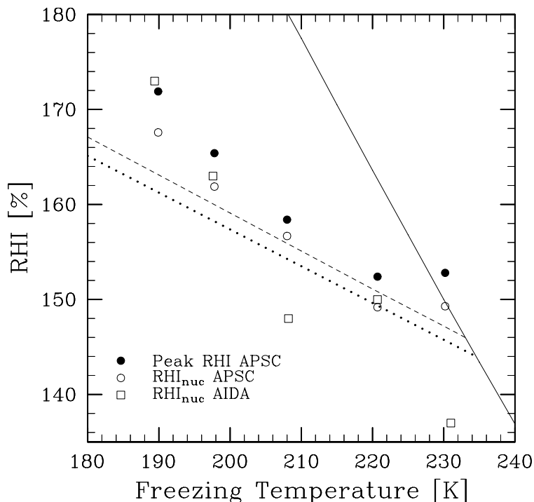
Fig. 11. Modeled baseline values of peak RHI and \text{RH}_{\text{nuc}} (closed and open circles) and measured threshold values for homogeneous ice nucleation inside the AIDA chamber (squares). The solid line indicates RHI when liquid water is saturated. The dashed (dotted) line depicts \text{RH}_{\text{nuc}} for which a particle with radius 0.25 (1) \mu\text{m} freezes homogeneously in one second (minute) (Koop et al., 2000). The experimental uncertainty of \text{RH}_{\text{nuc}} ranges from \pm 5\% at 230 K to \pm 12\% at 190 K (Möhler et al., 2002).
