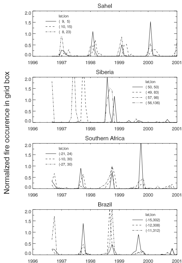
Fig. 2. Time series of the normalised monthly fire occurrence in selected grid boxes. The fire frequency has been derived by sampling ATSR nighttime active fire observations into 1^{\circ} \times 1^{\circ} grid boxes.
