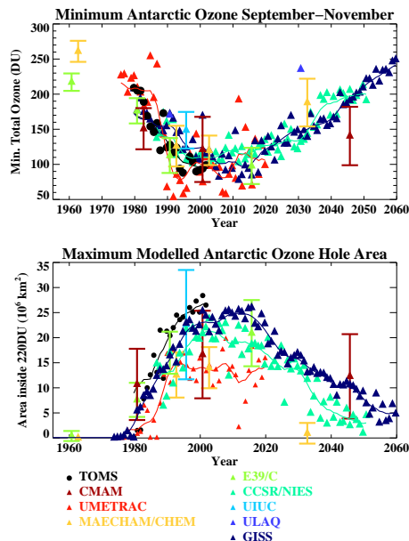
Fig. 10. Upper Panel: Minimum antarctic total ozone for September to November, computed by the participating models. For the transient models, the solid lines show the results of a gaussian smoother applied to the individual year's results (also plotted). For the timeslice experiments the mean and twice the standard deviation of the values within each sample are recorded by the error bars. For MAECHAM/CHEM only: (i) the values have been plotted two years late for clarity, (ii) a standard tropospheric column of 40 DU has been added to the computed stratospheric columns. Lower panel: The maximum area of the ozone hole during the period September to November, as given by the 220 DU contour, for TOMS observations and participating models. The TOMS data and transient model results are plotted for each year and with a gaussian filter applied (solid lines). For the timeslice experiments the means and twice the standard deviations of the model samples are included. The MAECHAM/CHEM results for 1960 indicated no ozone values below 220 DU and are not included in the figure.
