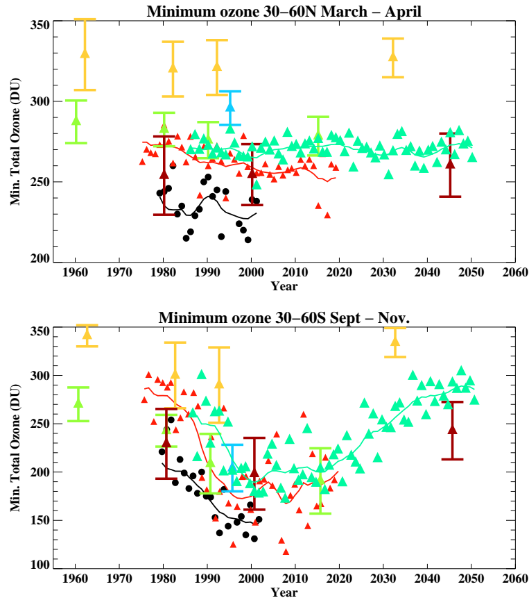
Fig. 11. Minimum total column ozone in the latitude range 30^{\circ} to 60^{\circ} in the Northern (upper) and Southern (lower) Hemispheres for participating models. See Fig. 10 for line styles and symbols.
