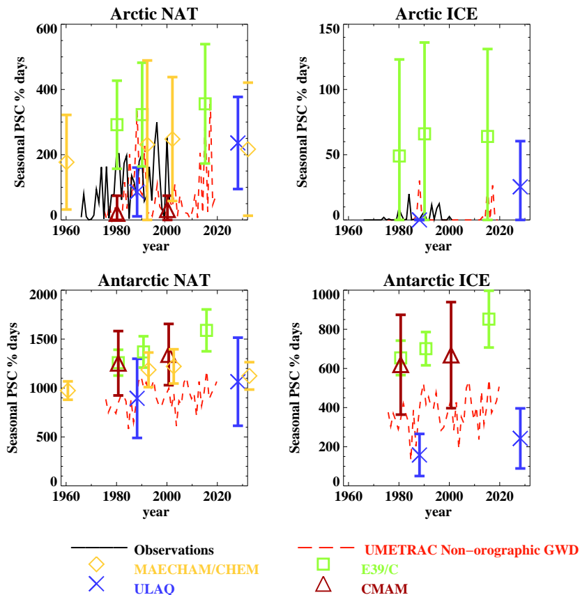
Fig. 6. Seasonal integration of the hemispheric area at 50 hPa, corresponding to the temperatures below 195 K (approximate NAT temperature) and below 188 K (approximate ICE temperature) for participating models. The error bars for the timeslice runs indicate 95% confidence intervals. For clarity, ULAQ data are plotted two years early, and for 1990 and 2030 MAECHAM CHEM data are plotted two years late.
