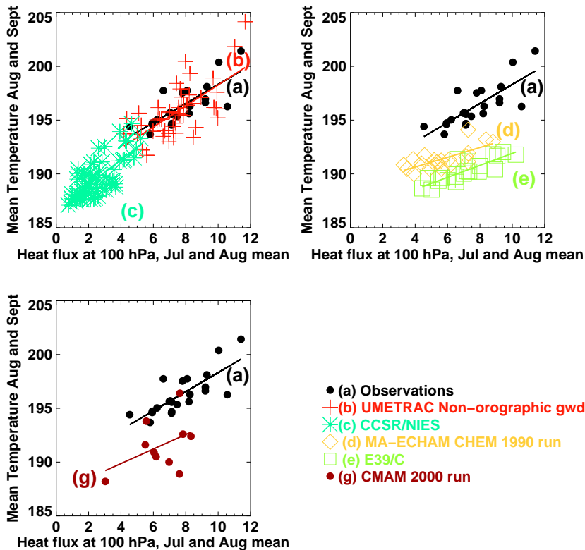
Fig. 5. As in Fig. 4, but for the Southern Hemisphere for the months July and August, and August and September, respectively. For convenience, the usual convention for \nu has been used (i.e. negative values indicate toward the South Pole) but the values have been multiplied by -1 .
