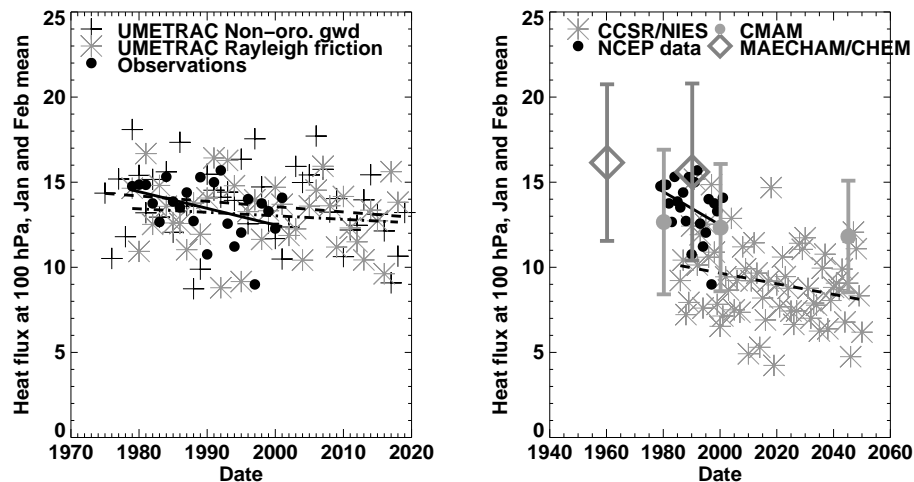
Fig. 8. Scatter diagrams of heat flux \overline{v'T'} (averaged 40^{\circ} – 80^{\circ} N, at 100 hPa for January and February) against year for participating models. In both panels, the linear regression line between the NCEP derived heat flux and time is drawn as a solid line. Left panel: the dashed line is the linear regression for the non-orographic gwd run of UMETRAC, and the dot-dash line is the linear regression for the Rayleigh friction run of UMETRAC. Right panel: the dashed line is the linear regression for the CCSR/NIES results and the CMAM and MAECHAM/CHEM results are indicated by dots and diamonds. Two standard deviations of the annual values are indicated by the error bars for the timeslice experiments.
