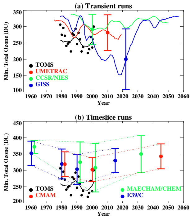
Fig. 9. Minimum Arctic (March/April) total ozone for the main experiments of this assessment. (a) Transient runs in comparison with TOMS data. The solid lines show the results of a gaussian smoother applied to the individual year's results. The error bars denote twice the standard deviation of the individual years from the smoothed curve. (b) Timeslice runs in comparison with TOMS data. The error bars denote the mean and twice the standard deviation of the individual years within each model sample (10 years for CMAM, 20 years for MAECHAM/CHEM and E39/C). Dotted lines are drawn between the end points of the error bars to assist in estimating trends by eye. For MAECHAM/CHEM only: (i) the values have been plotted two years late for clarity, (ii) a standard tropospheric column of 100 DU has been added to the computed stratospheric columns. Note that the MAECHAM/CHEM results are not symmetric about the mean, but have a long tail towards low values.
