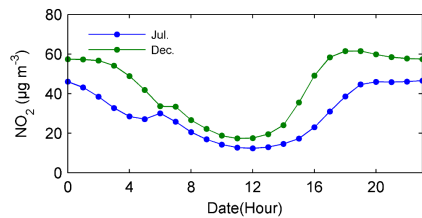
Fig. 2. The diurnal variation of NO 2 concentration from CUACE.
