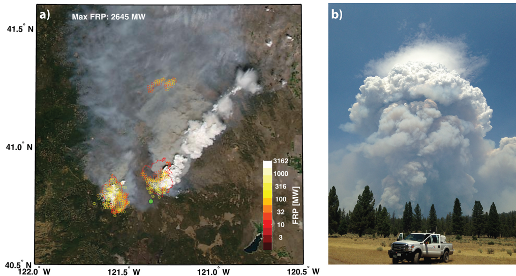
Figure 1. Overview of the Bald Fire. On 2 August 2014. (a) MODIS true color image at ~ 14:30 PDT overlaid with MODIS Fire Radiative Power (colored circles), and fire perimeters (dashed red lines). The maximum FRP is annotated and the truck location is shown as a green dot. (b) Photograph of the Bald Fire pyrocumulus at ~ 14:20 PDT showing the lidar vantage of the windward plume edge.
