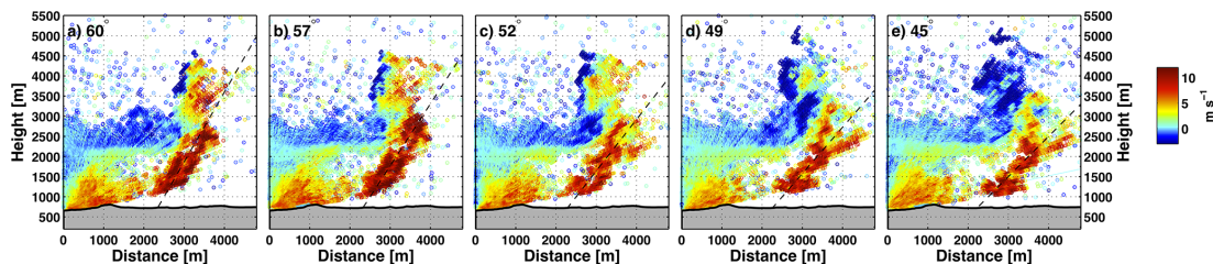
Figure 9. Lidar radial velocity during the second Rocky Fire plume rise sequence. Times are as in Fig. 7. Warm (cool) colors correspond to outbound (inbound) flow. The plume tilt angle is displayed adjacent to the panel label and the plume center line indicated as a black dashed line.
