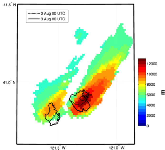
Figure 4. Radar derived echo tops for the Bald and Eiler Fires along with the evening fire perimeters.
