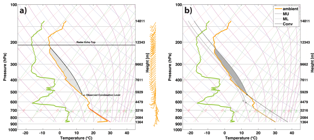
Figure 5. Skew-T Log-P diagrams showing radiosonde and parcel data during the Bald Fire Pyrocumulus event. (a) Observed temperature (orange) and dewpoint (green), modified CBL profile (dashed red), and observed condensation level, assumed moist adiabatic ascent (black dashed) with CAPE (grey shading). Also noted is the radar estimated echo tops. (b) Lifted parcel trajectories including the most unstable (MU), mixed-layer (ML), and convective parcels. The CAPE for each parcel is shaded and the condensation level for each parcel is denoted with a circle.
