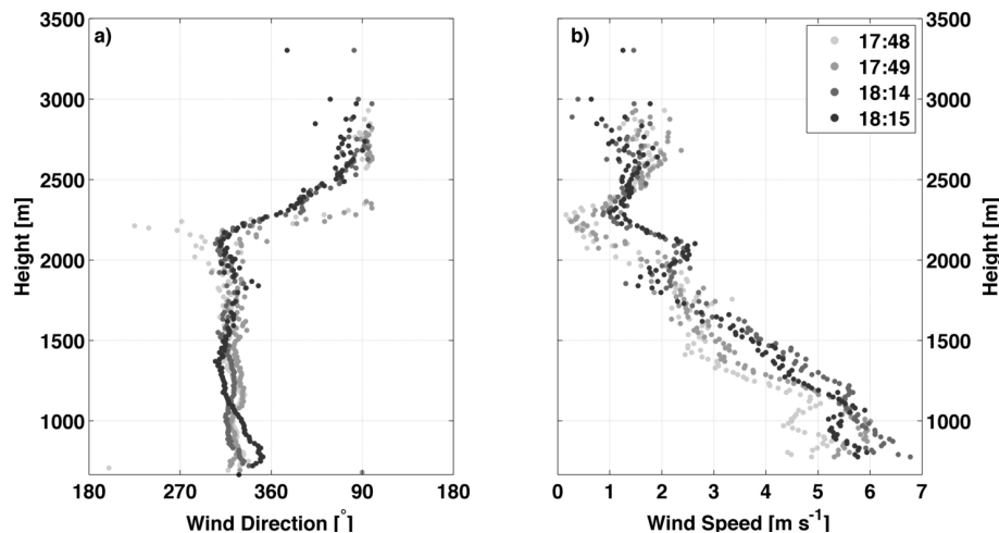
Figure 8. Lidar derived wind profiles during the second Rocky Fire pyrocumulus event. (a) Wind direction profiles, and (b) wind speed profiles. Gray shading corresponds to the time of the wind profile, which is shown in PDT in the legend.
