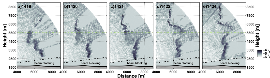
Figure 2. Lidar attenuated backscatter ( \text{m}^{-1} \text{sr}^{-1} ) sequence of the plume rise during the onset of a pyrocumulus on 2 August 2014. Flat gray shading shows where the lidar beam is attenuated. Times in PDT are shown next to the panel labels, and the light green line indicates the condensation level at 5500 m a.m.s.l.
