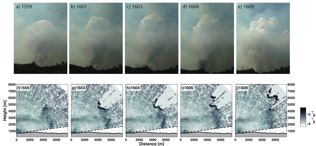
Figure 6. Pyrocumulus development during the Rocky Fire on 30 July 2015. (a–e) Photographs of the plume rise and pyroCu development. (f–j) Lidar backscatter showing the onset of condensation and subsequent cloud growth. All times are PDT.
