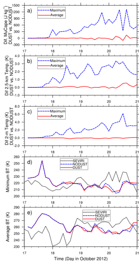
Fig. 10. (a) 3 hourly evolution of the maximum MuCAPE difference (dashed blue line) in the CV domain and MuCAPE difference averaged over the CV domain (solid red line) between the DUST and NODUST from 00:00UTC
