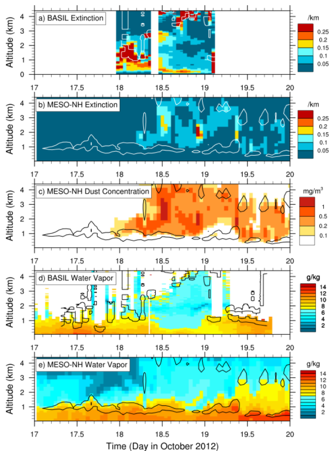
Fig. 6. Time-height series of extinction coefficients derived from (a) BASIL at 355 nm and (b) the Meso-NH DUST simulation - valid for the spectral range 0.25–0.44 \mu\text{m} over Candillargues between 00:00 UTC on 1
