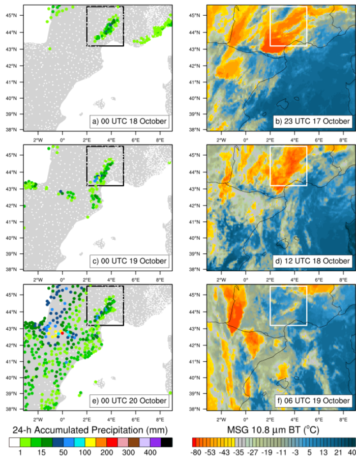
Fig. 2. Left column: 24-h rainfall amounts (from 00 UTC) derived from rain gauge measurements on (a) 17 October, (c) 18 October and (e) 19 October 2012. The thick black line delineates the CV area (2-5°E/43.2°N).
