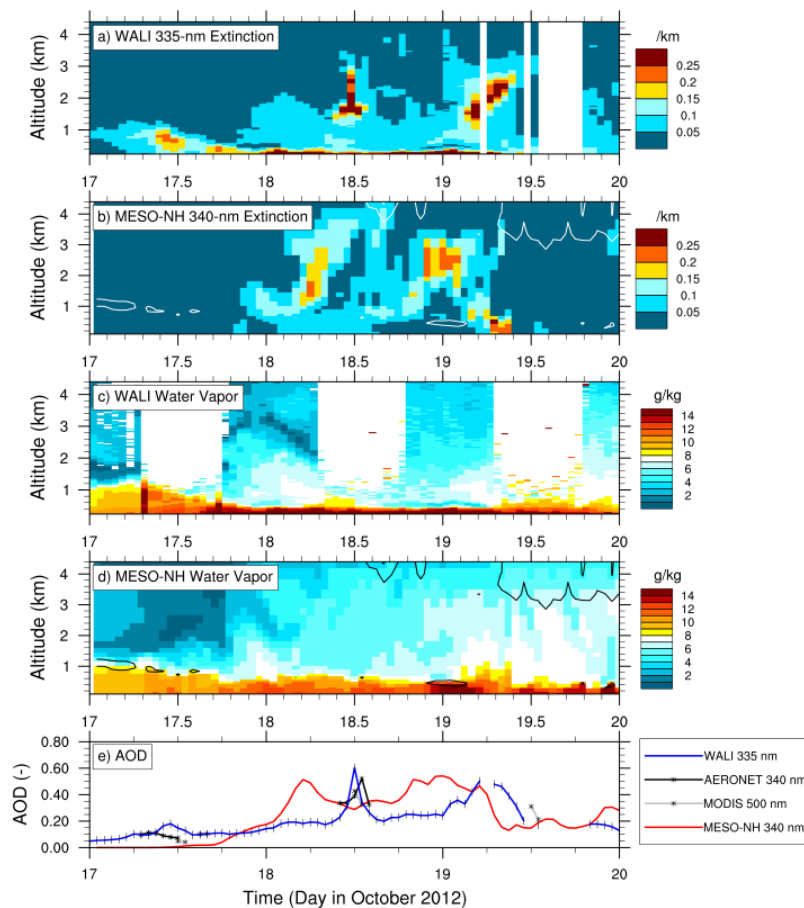
Fig. 5. Time-height series of extinction coefficients derived from (a) WALI at 335 nm and (b) the Meso-NH DUST simulation –valid for the spectral range 0.25–0.44 \mu\text{m} – over Menorca between 0000 UTC on 17 Octob
