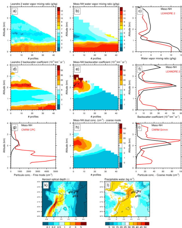
Fig. 7. (a) LEANDRE 2 derived water vapor mixing ratio between 17:16 and 17:23 UTC along the aircraft profile marked as “obs” in (k) , (b) Meso-NH water vapor mixing ratio at 21:00 UTC for the same horizontal
