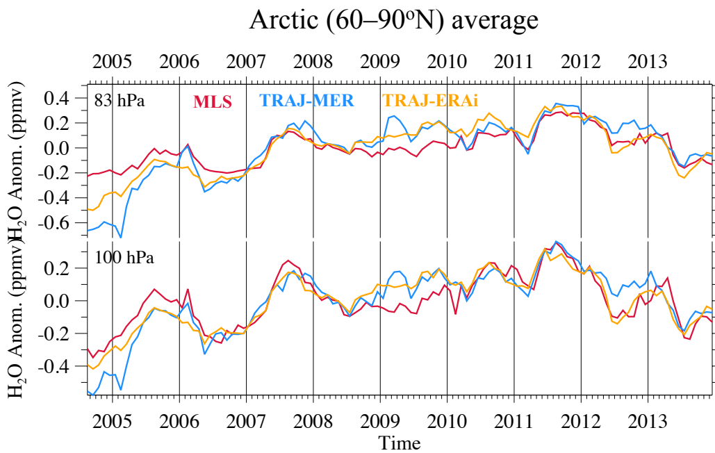
Figure. Arctic water vapor predicted from trajectories driven by MERRA (blue) and ERA interim (orange) circulation and GPS RO temperatures (refer Wang et al., 2015), compared to MLS observations. All trajectory results have been weighted by MLS averaging kernels.
