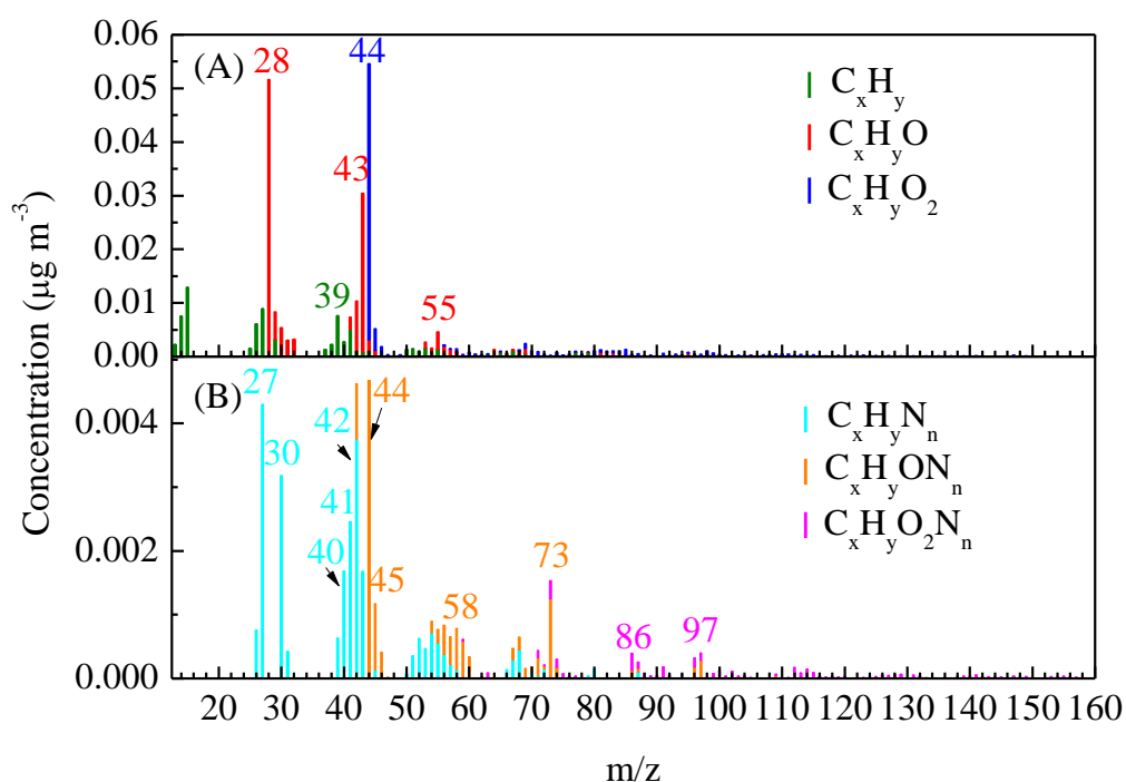
Fig. R2. Mass spectra of (a) non-N-containing species fragments and (b) N-containing species fragments in the SOA formed by OH oxidation of m-xylene in the presence of 66 ppbv NH 3 (Exp. M16).
