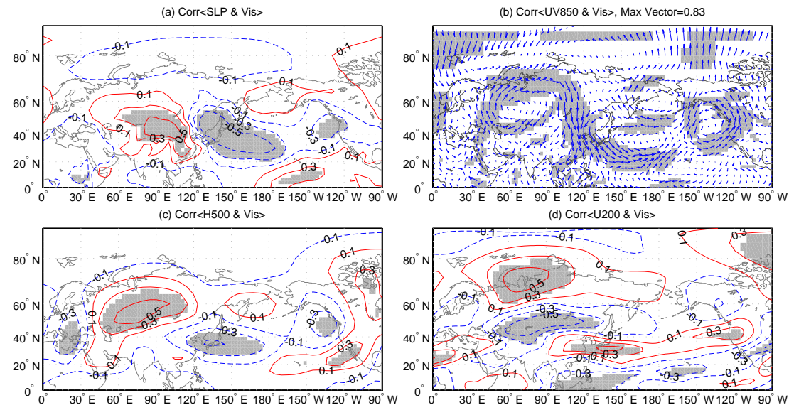
Fig. 3. Figure 3. Spatial distribution of correlation coefficients between visibility and SLP (a), UV850 (b), H500 (c) and U200 (d) (Area significant at the 0.05 level are shaded; either U850 or V850 significant)
