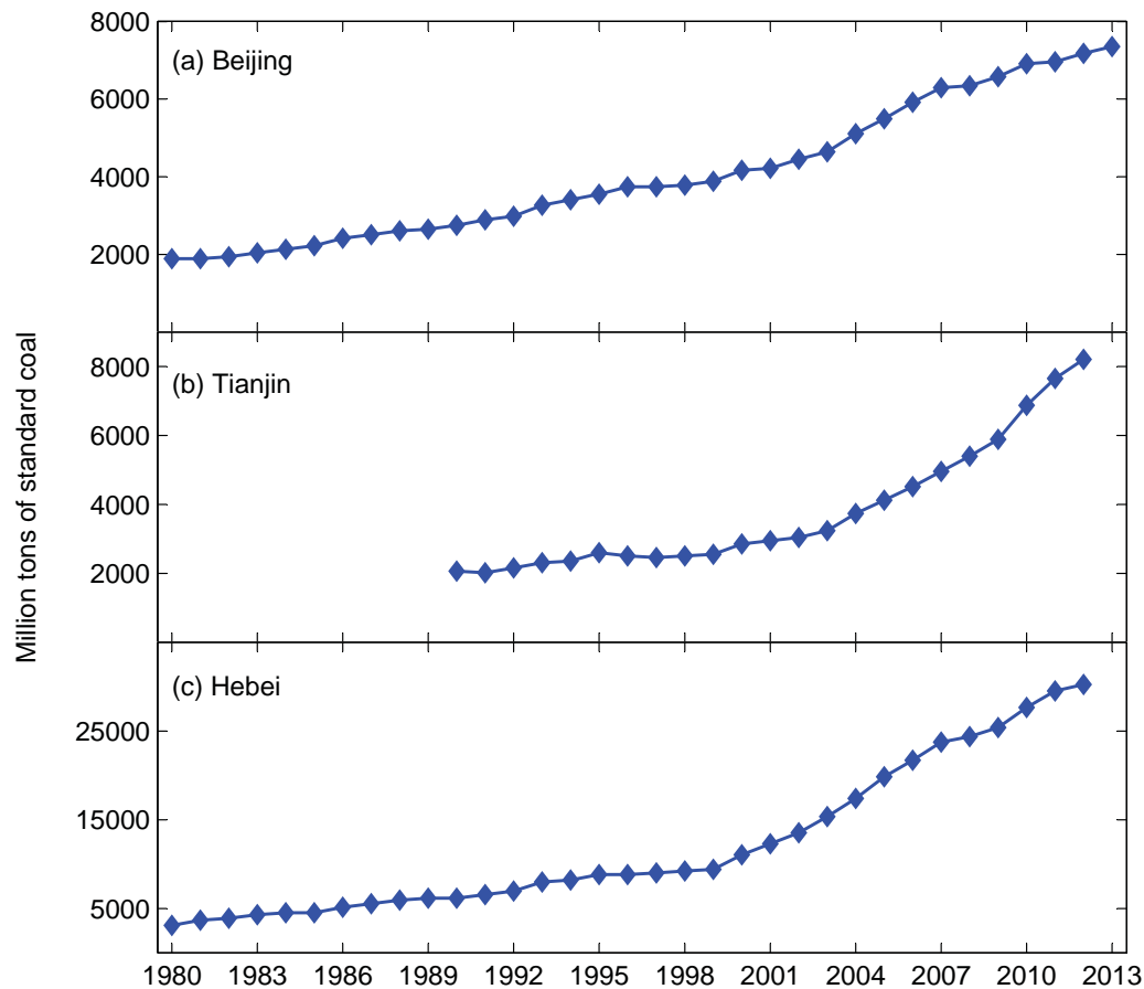
Fig. 1. Figure S1. Curves of the annual total energy consumption (million tons of standard coal) in Beijing (a), Tianjin (b) and Hebei province (c)
