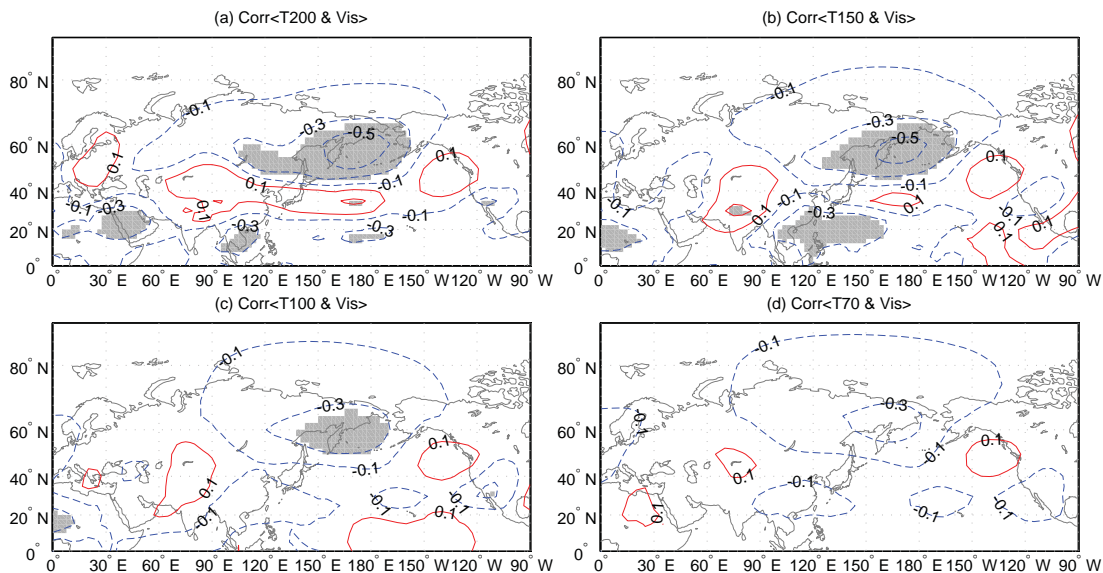
Fig. 4. Figure 4. Spatial distribution of correlation coefficients between visibility and T200 (a), T150 (b), T100 (c) and T70 (d) (Area significant at the 0.05 level are shaded)
