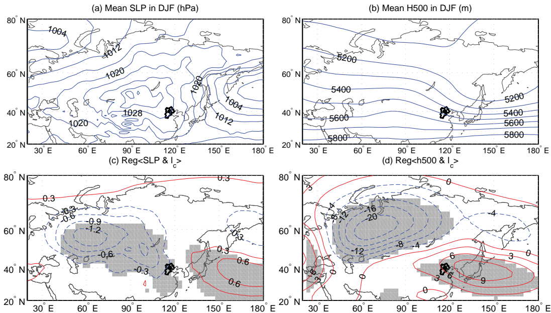
Fig. 5. Figure 6. The climatological mean fields of SLP (a) and H500 (b) averaged in winter 1981 to 2010, and the spatial distribution of the regression coefficients of SLP (c) and H500 (d) upon the I c over t
