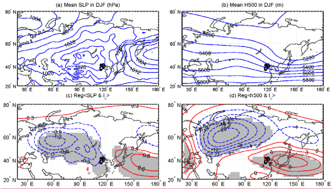
Figure 6 The climatological mean fields of SLP (a) and H500 (b) averaged in winter 1981 to 2010, and the spatial distribution of the regression coefficients of SLP (c) and H500 (d) upon the I_c over the period 1981 to 2015 (Area significant at the 0.05 level are shaded)
