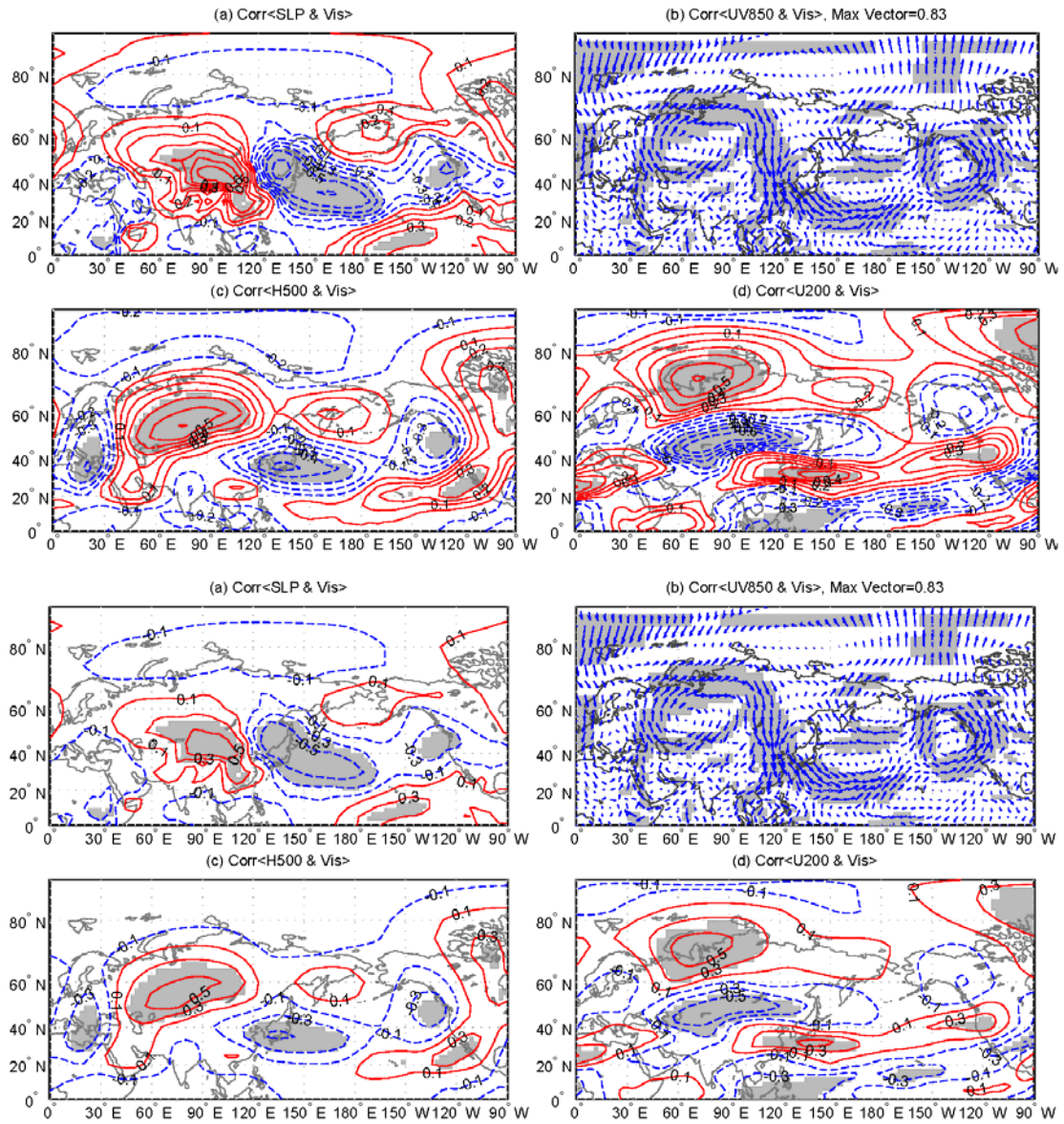
Figure 3, Spatial distribution of correlation coefficients between visibility and SLP (a), UV850 (b), H500 (c) and U200 (d) (Area significant at the 0.05 level are shaded; either U850 or V850 significant at the 0.05 level are shaded in b)
