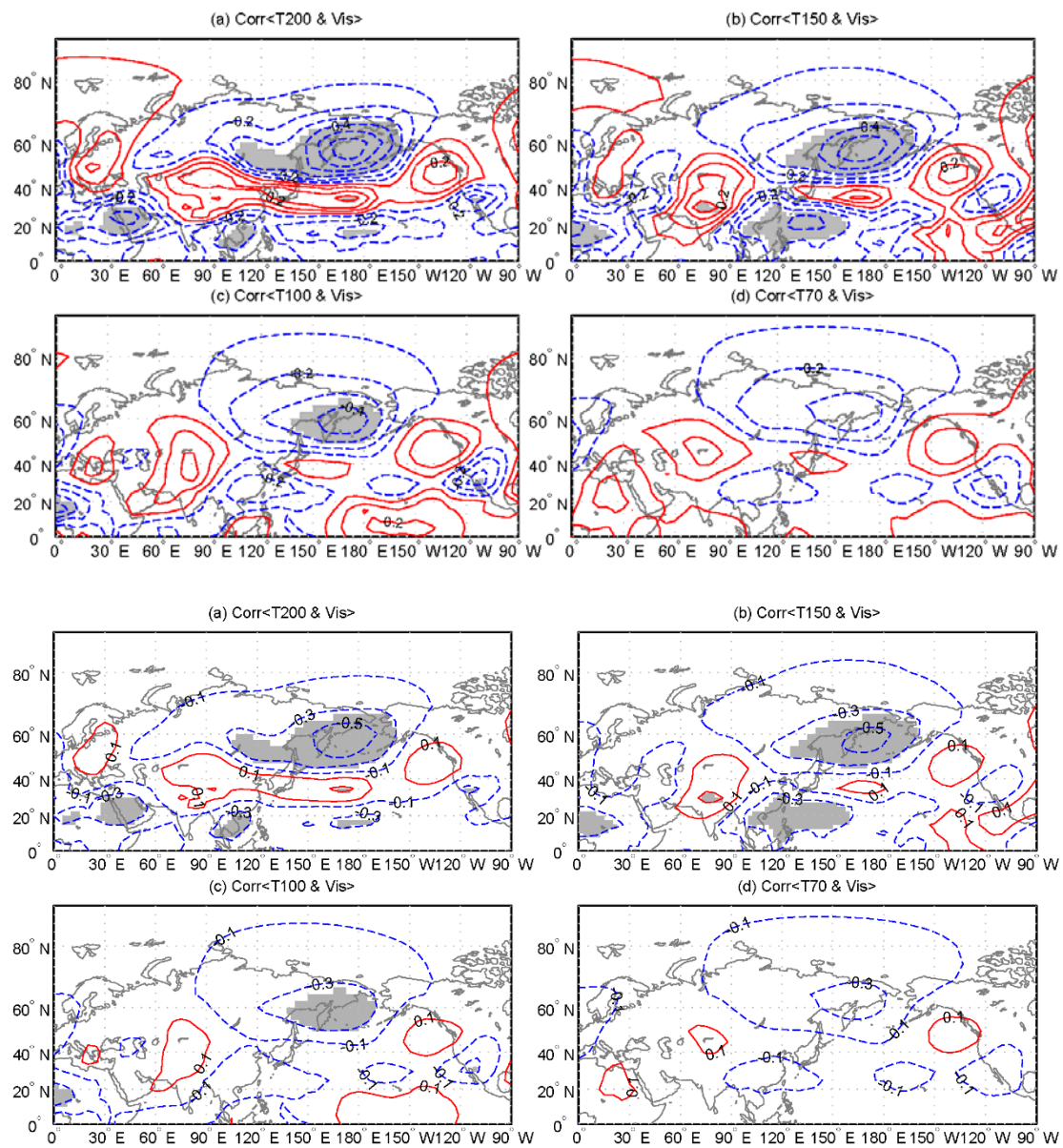
Figure 4 Spatial distribution of correlation coefficients between visibility and T200 (a), T150 (b), T100 (c) and T70 (d) (Area significant at the 0.05 level are shaded)
