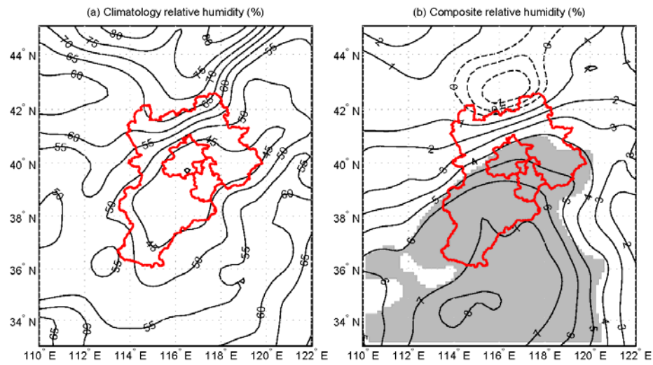
Figure 8 Same as Figure 7, but for relative humidity
