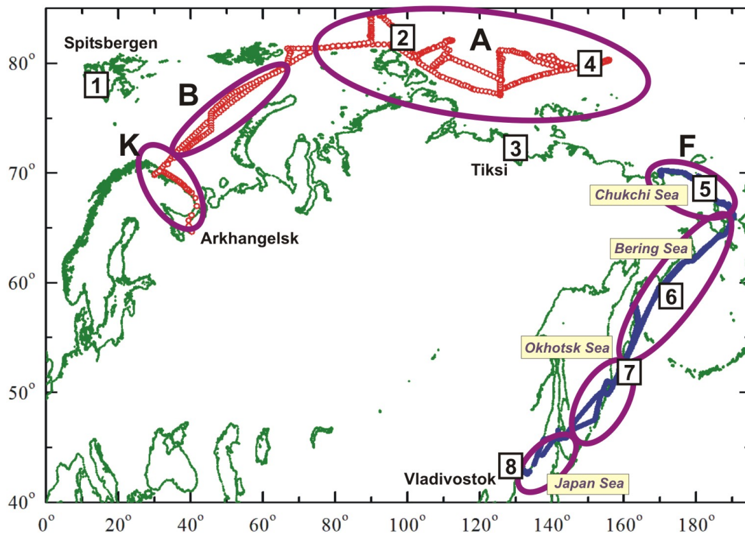
Fig. 1. (The updated Fig1.) Map of the routes of Arctic cruises of RV “Akademik Fedorov” and “Professor Khljustin”: numbers indicate the regions where AOD values were calculated; letters and ovals indicate the
