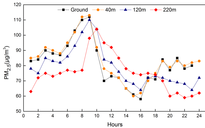
Fig. 7. Fig 5Vertical diurnal variation of PM2.5 mass concentrations during the period from July 1 to September 30, 2009
