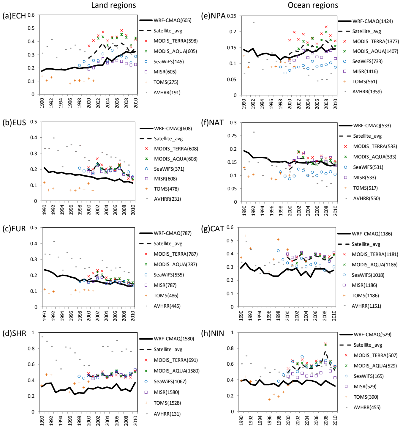
Fig. 3 Temporal series of regional JJA-averaged AOD from satellite retrievals and WRF-CMAQ
