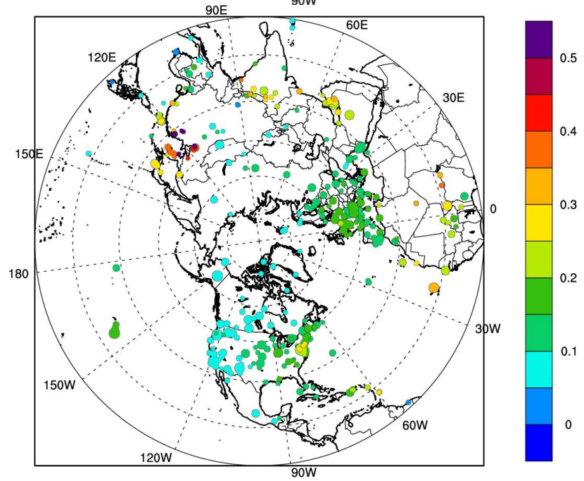
Fig. 4 Comparison of spatial distributions of summer AOD between AERONET and WRF-CMAQ (dot size indicates the extent of data coverage for the period 1990-2010; all converted into 533nm; sites marked by red boxes are selected for trend analysis)
