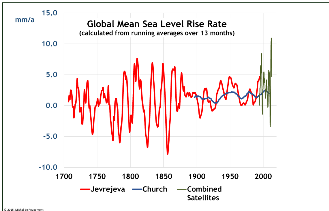
Fig. 2. Global mean sea level annual rise rate
