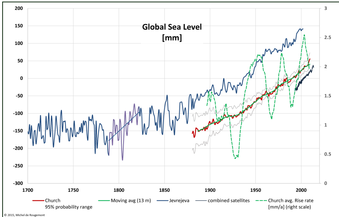
Fig. 1. Global mean sea level, various sources
