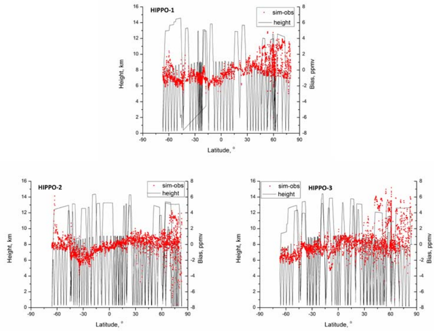
Fig. 1. Figure 3. Change of flight height and difference between simulation and observation of HIPPO-1, 2, 3 with latitude.
