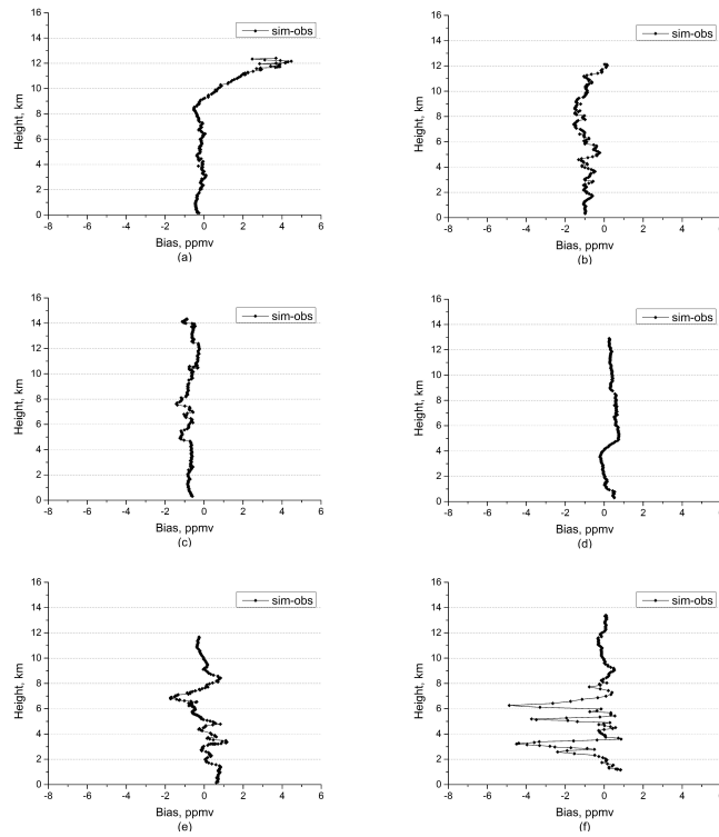
Fig. 3. Figure 7. Biases of simulation minus observation from near-surface to the LS for HIPPO-2, panels are corresponding to Figure 6(a)-6(f) respectively.
