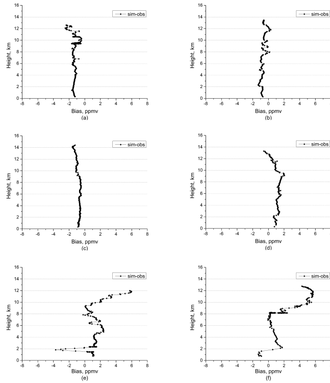
Fig. 4. Figure 9. Biases of simulation minus observation from near-surface to the LS for HIPPO-3, panels are corresponding to Figure 8(a)-8(f) respectively.
