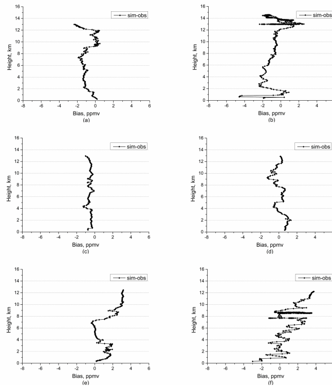
Fig. 2. Figure 5. Biases of simulation minus observation from near-surface to the LS for HIPPO-1, panels are corresponding to Figure 4(a)-4(f) respectively.
