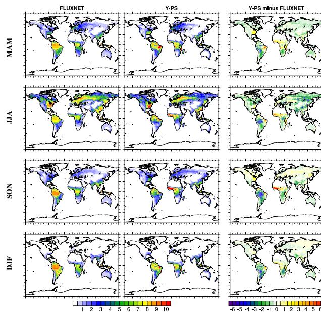
Figure S1. Seasonal averaged FLUXNET-derived GPP (first column), simulated GPP from NASA ModelE2-YIBs (using Y-PS algorithm, second column), and their difference (third column). The units are \text{g[C] m}^{-2} \text{day}^{-1} . GPP in Y-MEGAN and Y-MEGAN-SM are the same as GPP in Y-PS.
