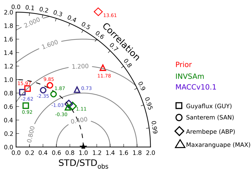
New Fig. 5. Taylor diagram of the statistics of misfits between observations and simulated CO 2 mole fractions between 12:00 and 15:00 LT at Guyaflux (square), Santerem (circle), Arembepe (diamond) and Maxaranguape (triangle), when wind speed > 2 m s -1 , using prior fluxes (red), INVSA m (green) and MACCv10.1 (purple). Radial distance from the origin: ratio of SD of simulated mole fractions and SD of the observations. Angle measured from the y axis: coefficient of correlation. Numbers next to the symbols: bias (in ppm). Gray circles: SD of the misfits (in ppm).
