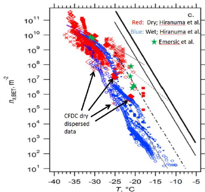
Figure 1. nx-illite n_s data from Hiranuma et al. (2014) split into dry-dispersed (red) and wet-suspended (blue) instruments. Emersic et al.'s data have been superimposed on this plot (green stars). The Emersic et al. chamber data are in disagreement with dry dispersed CFDC (continuous flow diffusion chamber) data from two groups (ETH-PINC and Colorado state). Aggregation as envisaged by the authors is not an issue in these experiments yet the CFDC data is in agreement with the wet-suspension measurements. The CFDC data is therefore inconsistent with Emersic et al.'s aggregation hypothesis.
