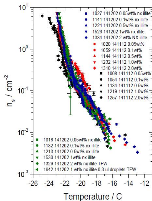
Figure 1. Values of n_s for nx-illite from experiments where the weight fraction of dust in microliter volume droplets was varied from 0.05 to 2 wt %. Aggregation is expected to change over this range of concentrations. The n_s values are independent of dust concentration which shows that the surface area available for nucleation is independent of aggregation.
