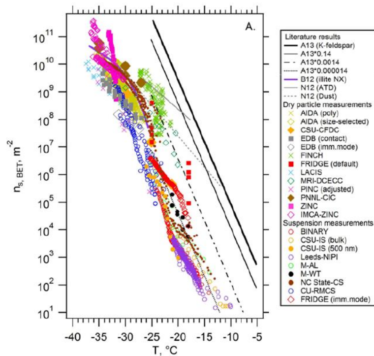
Figure 1. nx-illite \eta_s data from Hiranuma et al. (2014) showing the range of existing nx-illite data.
