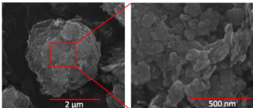
Figure 1. Scanning Electron Microscope (SEM) images of nx-illite. An aggregate of several micrometers in size is shown on the left and a close up (right) reveals that it is composed of many particles on the order of 10–100s of nanometres across. This is consistent with the gas adsorption measurements, which suggested average particles sizes of 20 nm (assuming smooth spheres – see (Broadley et al., 2012) for details).
