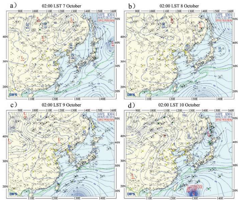
Fig. 9 Surface pressure on the surface at (a) 02:00 LST 7 October, (b) 02:00 LST 8 October, (c) 02:00 LST 9 October, and (d) 02:00 LST 10 October.
