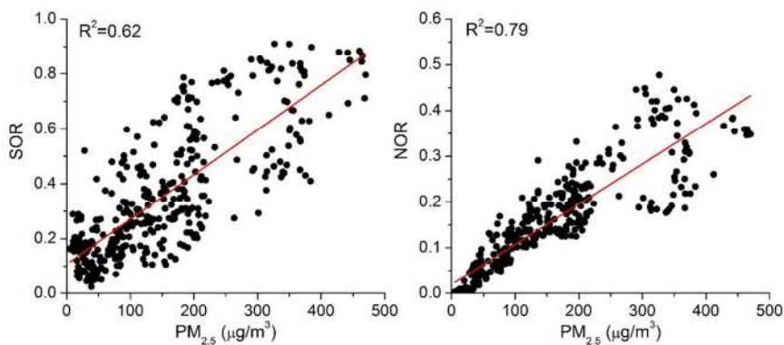
Fig.2 Relationship between \text{PM}_{2.5} and SOR, NOR
