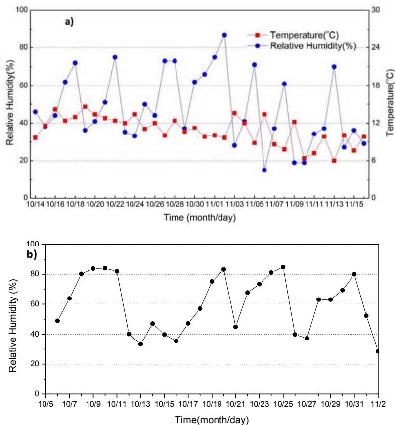
Fig.1 Comparisons of RH in a) October, 2013 (Feng et al. 2014) and b) October, 2014
