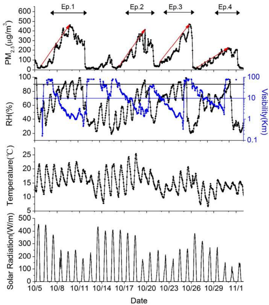
Fig. 2 Time series of observed PM_{2.5} , RH, temperature and solar radiation in Beijing from 5 October to 2 November 2014.
