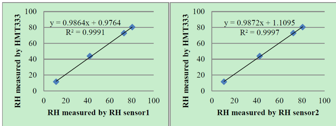
Fig. 2. The calibration of RH sensors
