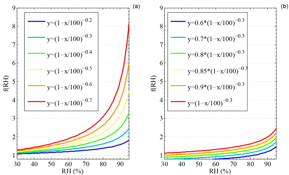
Fig. 2. Sample curves of f(RH)=c*(1-RH)^g with various c and g .
