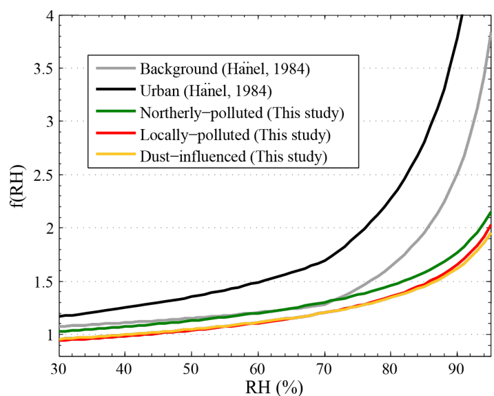
Fig. 3. Fitting curves of humidograms of Hänel and this study.
