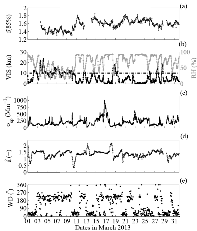
Fig. 4. Time series of measured and derived aerosol variables, as well as the ambient RH and visibility.
