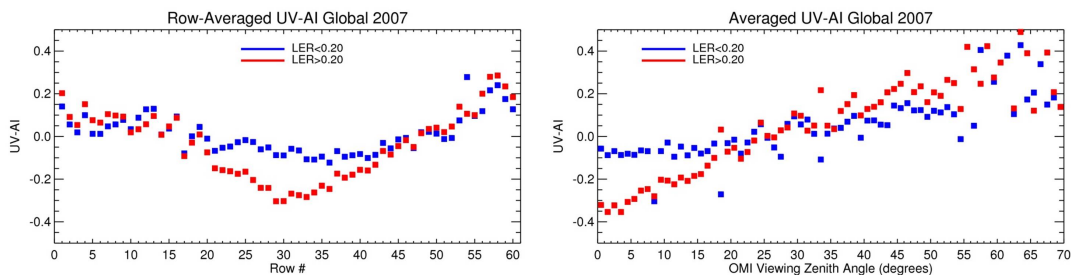
Fig. 2. OMI UV Aerosol Index as a function of Row number (left) and satellite viewing zenith angle (right) for year 2007. All OMI UV-AI data collected by repesctive rows and for a given viewing zenith angle \theta
