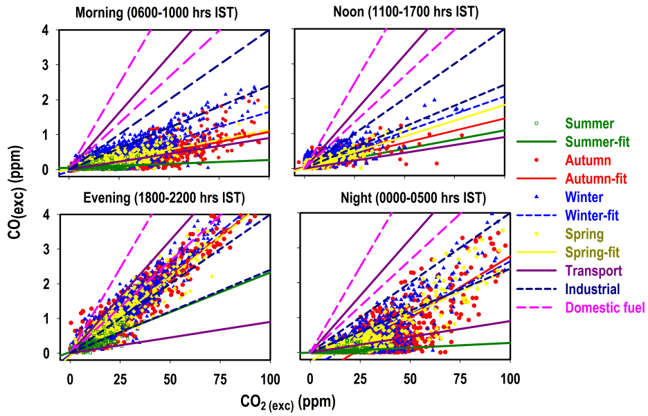
Fig. 1. Scatter plots and regression fits of excess CO (CO(exc)) vs. excess CO 2 (CO 2 (exc)) during morning (0600-1000 hrs), noon (1100-1700 hrs), evening (1800-2200) and night (0000-0500 hrs) hours.
