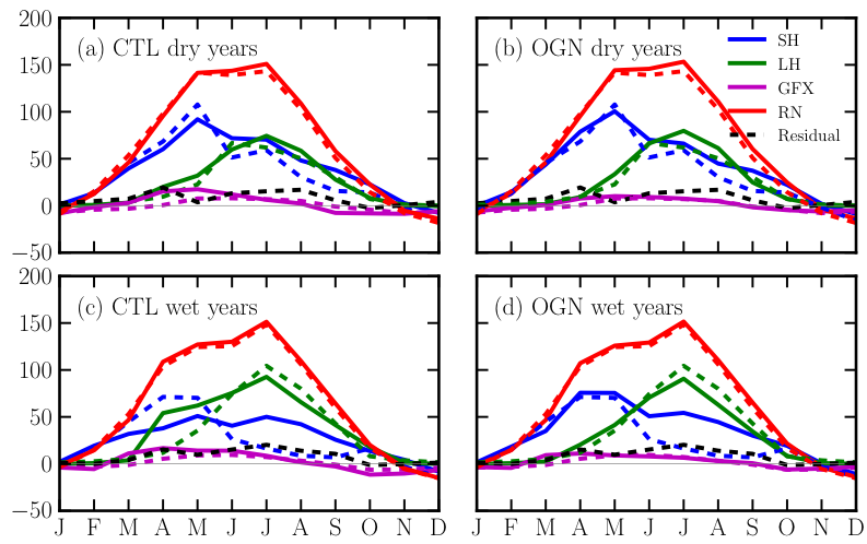
Fig. 1. Annual cycle of selected surface energy cycle fields
