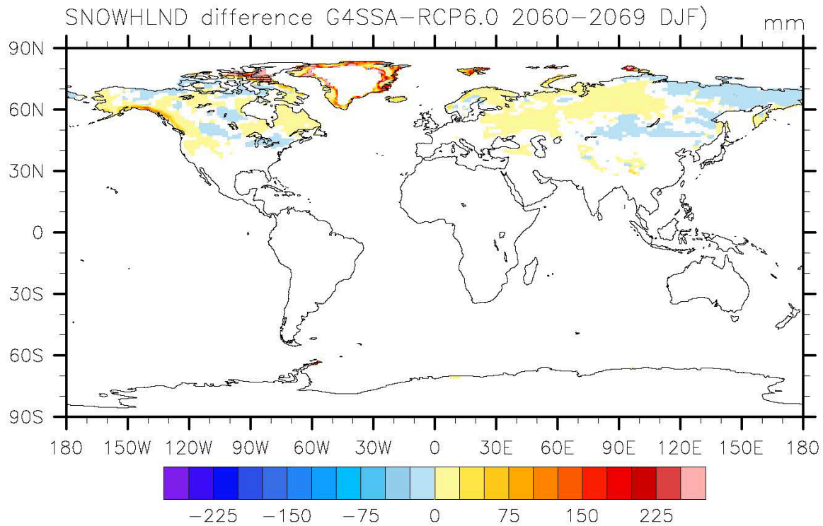
Figure 3. Water equivalent snow depth difference (mm) between G4SSA and RCP6.0 in DJF (average of 2060-2069) (-1 – 1 mm is marked as white).
