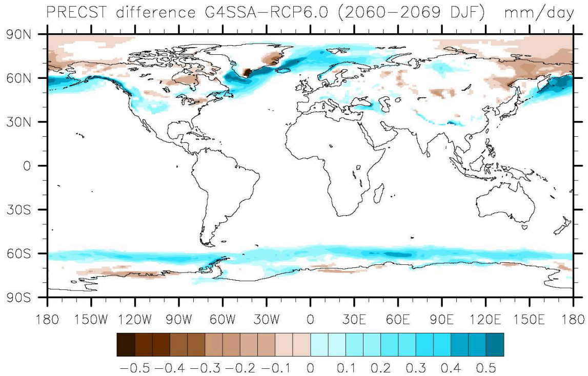
Figure 2. Convective/Large-scale snow rate difference (mm/day) between G4SSA and RCP6.0 in DJF (average of 2060-2069) (-0.05 – 0.05 mm/day is marked as white).
