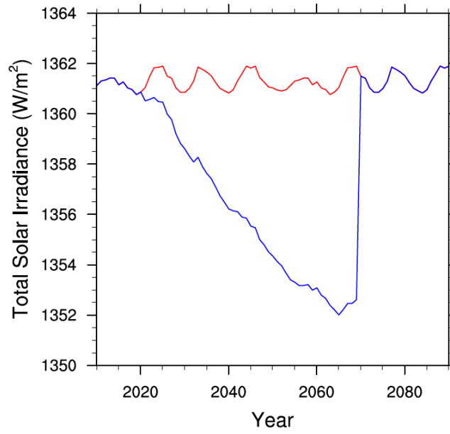
Figure1: Total solar irradiance ( \text{W}/\text{m}^2 ) for G3S, baseline experiment (red), solar dimming experiment (blue).
