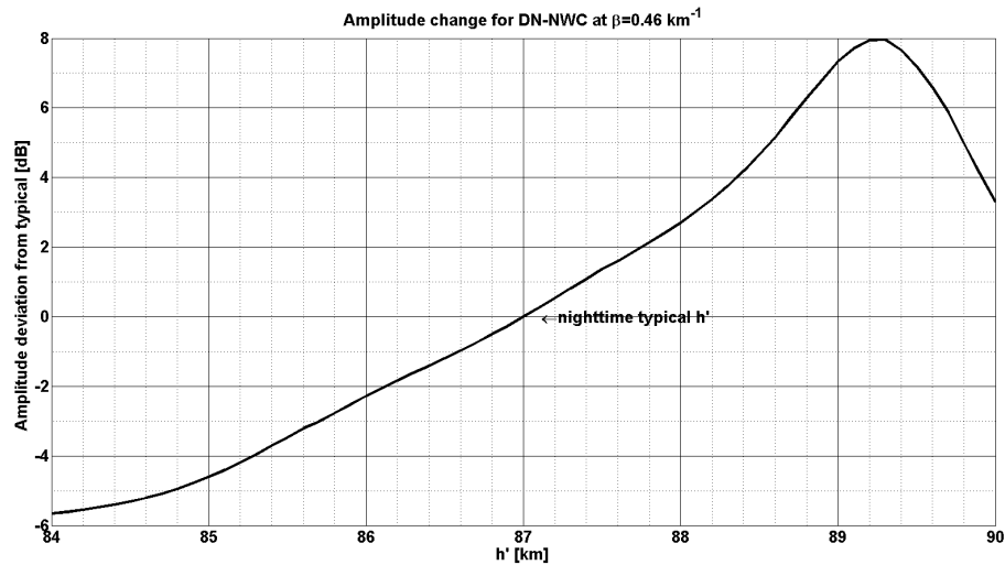
Fig. 1. LWPC model's output for nighttime DN-NWC used in order to find h' change equivalent to the SAO amplitude in VLF measurement.
