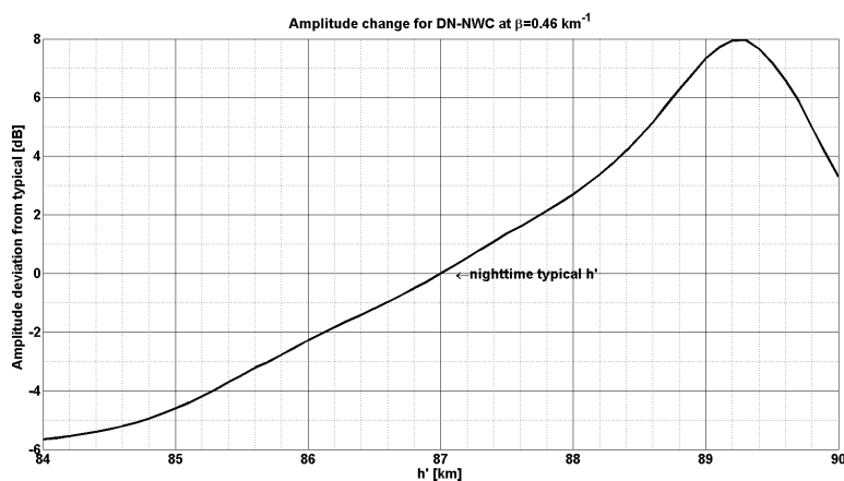
Fig. 1. LWPC model's output for nighttime DN-NWC used in order to find h' change equivalent to the SAO amplitude in VLF measurement.
