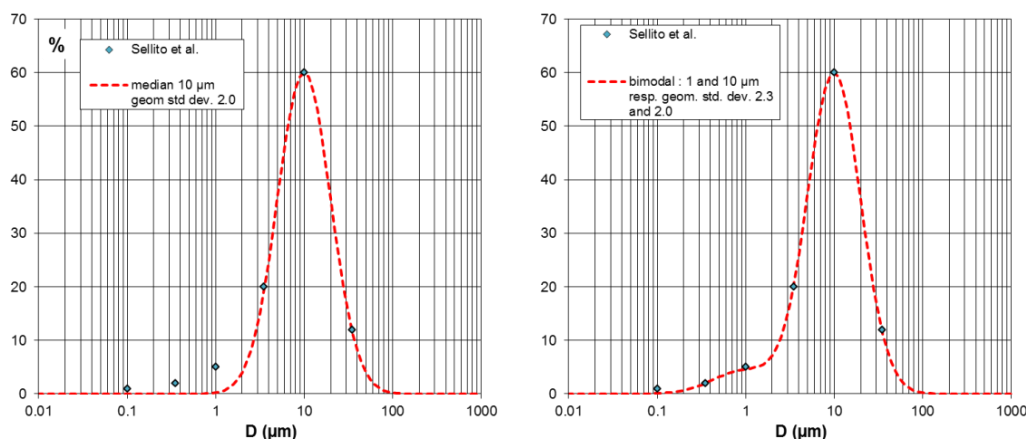
Figure 1: Rough adjustment of the particle size distribution proposed in table 1 of the paper (blue dots), by a monomodal lognormal with a geometric mean diameter of 10 \mu\text{m} (left), and by adding a second mode to fit the tail of the distribution at small sizes (right).
