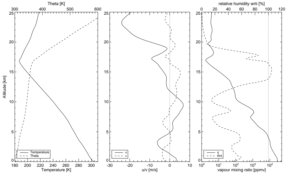
Figure 3. Profile of meteorological parameters prior to Hector development (04:30 UTC). Profiles are averaged over domain 5 and show temperature and potential temperature in the left panel, the u and v wind components in the middle panel, and relative humidity with respect to ice and water vapour mixing ratio in the right panel.
