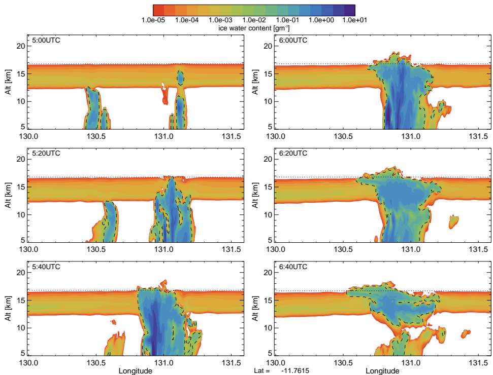
Figure 5. IWC cross sections between 05:00 UTC and 06:40 UTC. The dashed line represents the 0.01 \text{ g kg}^{-1} ice mixing ratio, representing the cloud boundary, and the dotted line indicates the simulated cold point tropopause.
