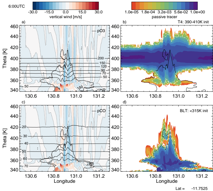
Figure 9. Same as Fig. 8 but for 06:00 UTC.
