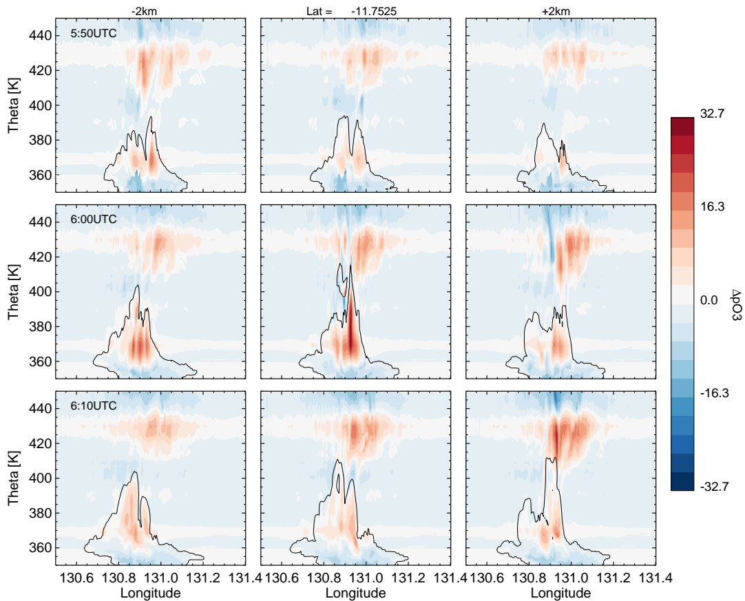
Figure 10. Cross sections of pO 3 difference to the initialisation profile ( \Delta pO_3 ). By shifting the cross section 2 km to the South/North (right/left) and 10 minutes prior/after (upper/lower panels) the variability of the cloud and the \Delta pO_3 field become visible.
