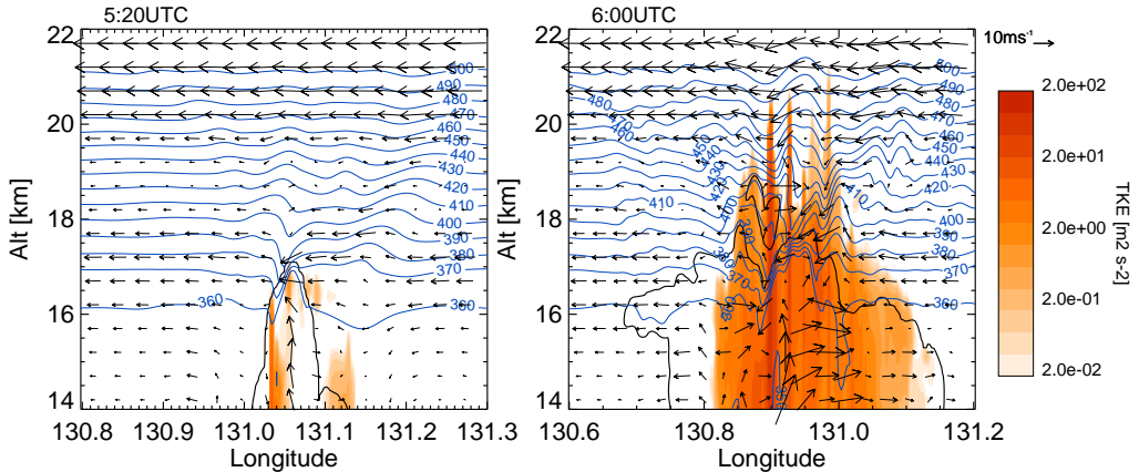
Figure 12. Vertical cross sections of parameterised TKE at 05:20 UTC (left) and 06:00 UTC (right). The thick black line denotes the 0.01 \text{g kg}^{-1} ice mixing ratio and the thinner blue lines depict isentropes. Also superimposed are the u-w wind vectors.
