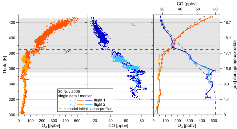
Figure 1. Observed ozone and carbon monoxide mixing ratio profiles (left and middle panel) during the double flight on 30 Nov 2005. On the right, the median observed profiles with the 33 and 67 percentiles (error bars) are shown together with the model initialisation profiles (see Sect. 5). The shading indicates the TTL as defined by Fueglistaler et al. (2009) and the dashed line indicates the cold point tropopause (CPT) .
