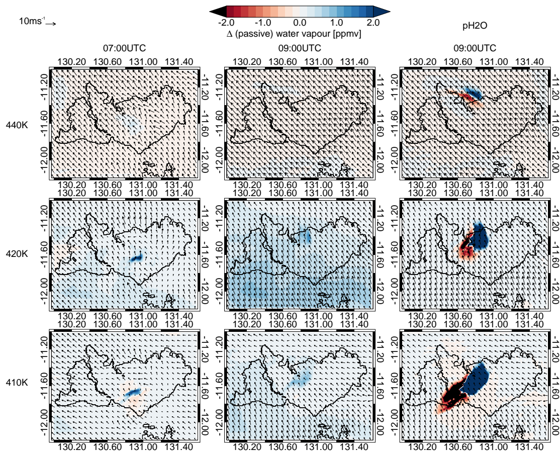
Figure 15. Change in humidity at 07:00 UTC (left column) and 09:00 UTC (middle column) on different potential temperature levels. The right column shows the change of pH 2 O at 09:00 UTC for comparison. Superimposed are the horizontal wind vectors on the respective level.
