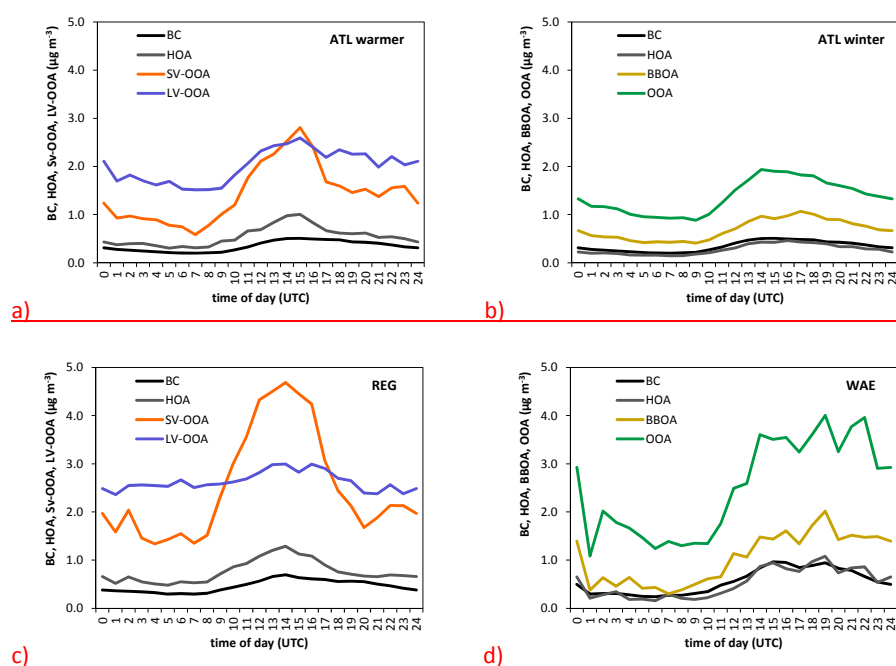
Figure S12. Average daily pattern for Atlantic advections (ATL), for the warmer and the colder periods, regional episodes (REG) (only warmer period), and Winter Anticyclonic episodes (WAE) (only colder period).
