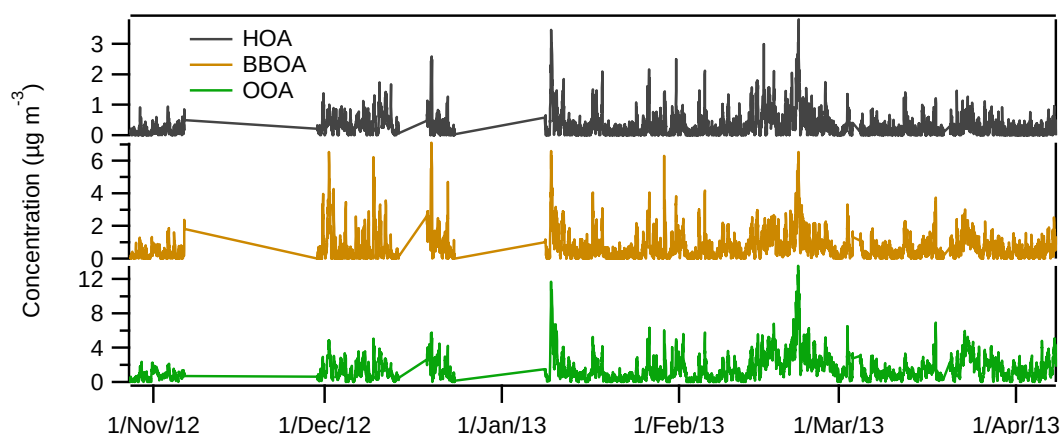
Figure S11. Time series of the OA sources in the warmer (top) and the colder (bottom) periods.
