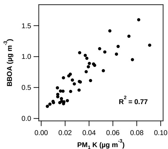
Figure S13. Contribution of BBOA in winter (averaged to 24-h periods matching the filter sampling) vs potassium concentrations in PM 1 .
