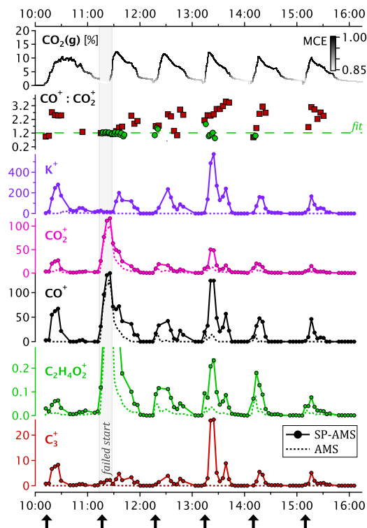
Figure 2. Time series for the aged beech-wood-combustion experiment. All traces are analogous to Fig. 1 but are scaled differently. Note especially the change of scale for C_2H_4O_2^+ . In this experiment, the second batch of wood failed to start (grey shading), causing OM concentrations tenfold greater than normal. This especially increased the signal at C_2H_4O_2^+ (a tracer ion for holocellulose pyrolysis), which has been plotted off-scale during that period to allow features at other times to be visible. The MCE during this period was also off-scale, with mean 0.82.
