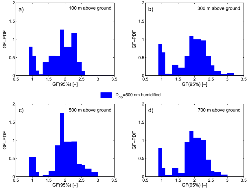
Figure 11. GF-PDFs recorded near Cabauw on 24 May 2012 at four different altitudes: approximately 100, 300, 500 and 700 m AGL seen in panels (a–d), respectively. Every curve is the mean over the two flown profiles NHP1 and NHP2.
