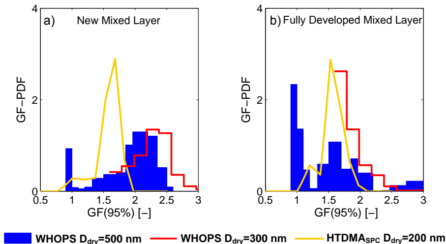
Figure 5. GF-PDF comparison between WHOPS (at 100 m AGL) and HTDMA in the Po Valley on 20 June 2012. The WHOPS results were averaged from 8:30 - 10:00 LT for the new ML and 12:30 - 14:00 LT for the fully developed ML, equivalent to results in Fig. 3a and b. The HTDMA data was averaged over the same time interval which corresponds to the mean over 3 full measurements per layer. Note that the WHOPS cannot reliably detect particles with GF < 1.5 and D_{dry} = 300 nm, as described in Rosati et al. (2015a). Thus, no information is available from the WHOPS measurements on the number fraction and properties of the 300 nm particles with GF < 1.5 .
