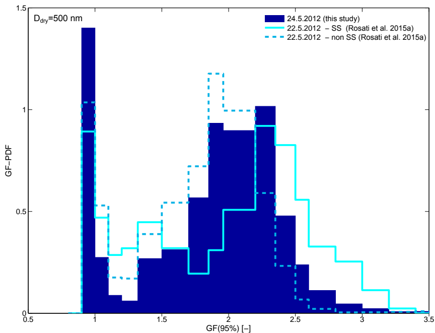
Figure 14. Comparison of GF-PDFs recorded with the WHOPS on board of the Zeppelin for two different flight days: 24 May 2012 (this study) and on 22 May 2012 (Rosati et al., 2015a). Both flights were located close to Cabauw and results are representative for particles with D_{\text{dry}} = 500 \text{ nm} .
