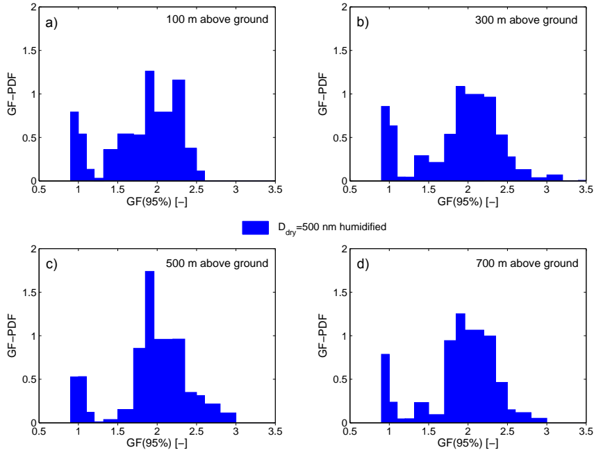
Figure 11. GF-PDFs recorded near Cabauw on 24 May 2012 at four different altitudes: approximately 100, 300, 500 and 700 m AGL seen in panels (a–d), respectively. Every curve is the mean over the two flown profiles NHP1 and NHP2.
