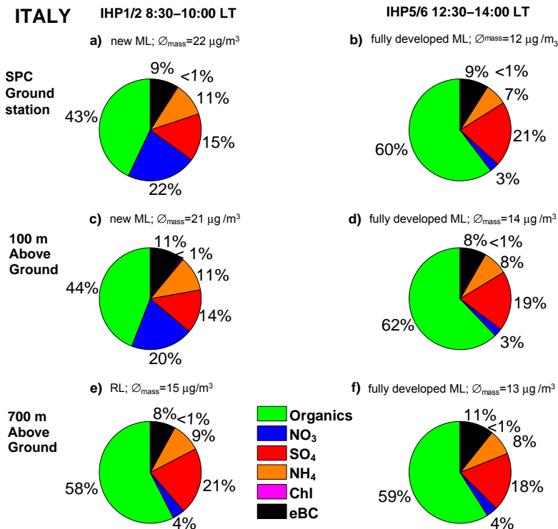
Figure 6. \text{PM}_{10} chemical composition results from the flight on 20 June 2012 in Italy. (a and b) show the mass fractions measured by the HR-ToF-AMS and MAAp at San Pietro Capofiume ground station; (a) was recorded during IHP1/2 whereas (b) was measured during IHP5/6. (c–f) depict the mass fractions measured by the HR-ToF-AMS and aethalometer on the Zeppelin. (c and e) illustrate the results for the first height profiles, (c) at 100 and (e) at 700 m AGL, while (d and f) show the results for IHP5/6 for 100 and 700 m AGL, respectively.
