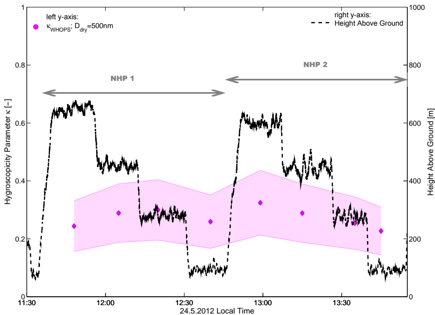
Figure 13. Time series of \kappa values retrieved during the flight on 24 May 2012. WHOPS results for a dry diameter of 500 nm are presented. The measurement accuracy is shown as the shaded area. Additionally, the flight altitude is indicated.
