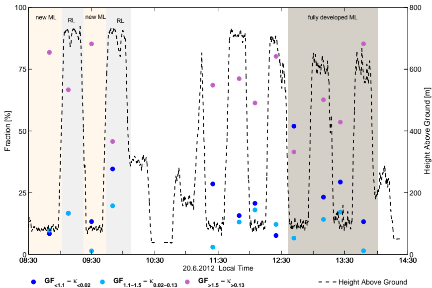
Figure 4. Time series of the mixing state of the aerosol particles (with D_{\text{dry}} = 500 nm) for the height profiles in Italy on 20 June 2012. Particles are classified into three hygroscopicity categories according to their GF: \text{GF} < 1.1 , 1.1 < \text{GF} < 1.5 , \text{GF} > 1.5 , in blue, light blue and pink respectively; these are equivalent to \kappa < 0.02 , 0.02 < \kappa < 0.13 and \kappa > 0.13 . The black, dashed line denotes the flight altitude. The labelled, coloured areas refer to the layer which was probed at the certain altitude.
