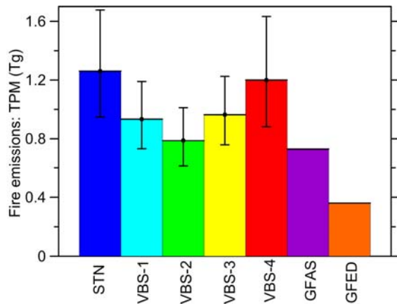
Figure 11. (a) Top-down estimates (in Tg) of total BB aerosol emissions from the study region in the period from 1 July to 31 August 2010 according to different simulation scenarios and in comparison with total particulate matter (TPM) emission data from the GFASv1.0 and GFED3.1 inventories. The estimates are derived from the MODIS AOD measurements. (b) The corresponding optimal estimates of F_\alpha derived from MODIS (boxes with solid filling) measurements in comparison with corresponding estimates (boxes with dashed filling) obtained from ground-based measurements in the Moscow region. Note that the estimates for the “unrealistic” scenario “VBS-5”, which would exceed the axis limits (see Sect. 3.4), are not shown.
