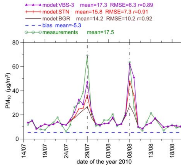
Figure 4. The same as in Fig. 3 but for PM_{10} concentrations, except that in addition to results for the STN and BGR runs, this figure also shows (by a purple line) results for the VBS-3 run.
