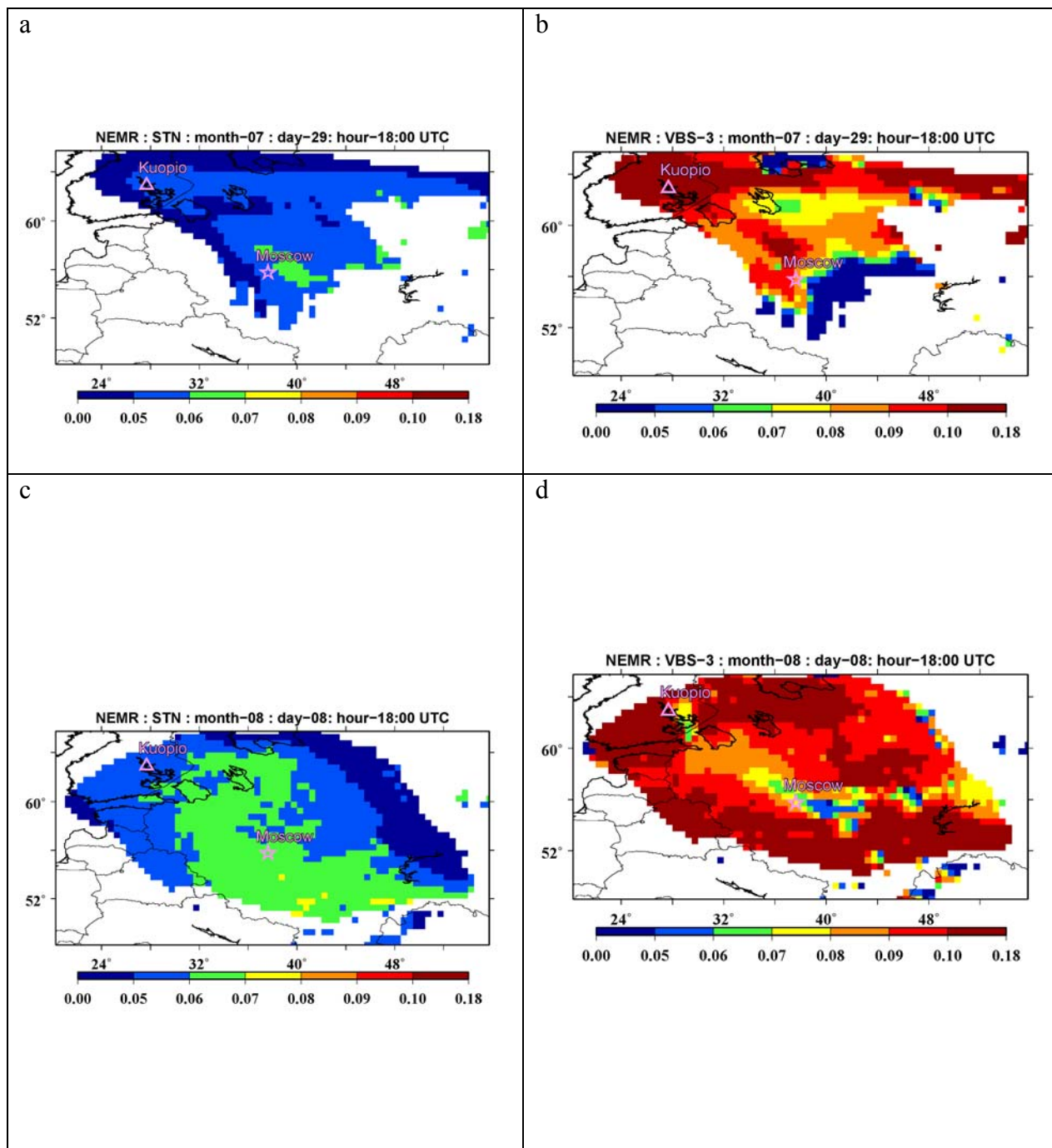
Figure 6. Normalized excess mixing ratio (NEMR) calculated as the ratio of near-surface mass concentrations of PM 10 and CO ( \text{g g}^{-1} ) originating from the fires. The NEMR values are shown only in the grid cells with CO concentrations exceeding 100 \mu\text{g m}^{-3} for 29 July (a,b) and 8 August (c,d) 2010 according to the STN (a,c) and VBS-3 (b,d) scenarios.
