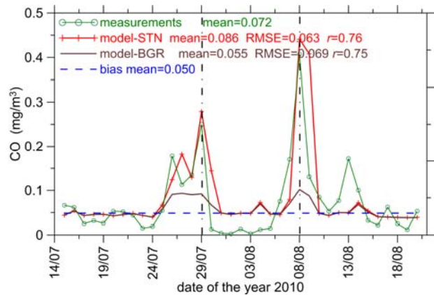
Figure 3. Time series of daily CO concentrations in Moscow (a) and in Kuopio (b). The CO concentrations for the simulation scenario "STN" (see the red lines with crosses) are obtained by taking into account both anthropogenic and fire emissions (as explained in Section 2.8), while that for the "BGR" run (see the solid brown lines) reflects only anthropogenic CO emissions (along with other sources contributing to the boundary conditions for CO). The dashed blue lines depict the model bias (representing the systematic difference between the simulations and measurements on days not affected by fires); note that a negative bias (specifically, in the plot "a") is shown with the opposite sign. The measurement data (from Mosecomonitoring stations and the Maaherrankatu site in Kuopio) are shown by green lines. The vertical dashed lines indicate the CO concentrations observed (a) in Moscow on 28 July and 7 August and (b) in Kuopio on 29 July and 8 August.
