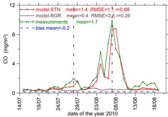
Figure 3. Time series of daily CO concentrations in Moscow (a) and in Kuopio (b). The CO concentrations for the simulation scenario "STN" (see the red lines with crosses) are obtained by taking into account both anthropogenic and fire emissions (as explained in Section 2.8), while that for the "BGR" run (see the solid brown lines) reflects only anthropogenic CO emissions (along with other sources contributing to the boundary conditions for CO). The dashed blue lines depict the model bias (representing the systematic difference between the simulations and measurements on days not affected by fires); note that a negative bias (specifically, in the plot "a") is shown with the opposite sign. The measurement data (from Mosecomonitoring stations and the Maaherrankatu site in Kuopio) are shown by green lines. The vertical dashed lines indicate the CO concentrations observed (a) in Moscow on 28 July and 7 August and (b) in Kuopio on 29 July and 8 August.
