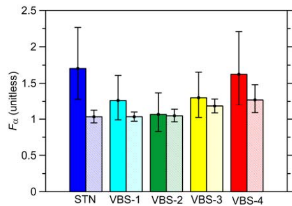
Figure 11. (a) Top-down estimates (in Tg) of total BB aerosol emissions from the study region in the period from 1 July to 31 August 2010 according to different simulation scenarios and in comparison with total particulate matter (TPM) emission data from the GFASv1.0 and GFED3.1 inventories. The estimates are derived from the MODIS AOD measurements. (b) The corresponding optimal estimates of F_\alpha derived from MODIS (boxes with solid filling) measurements in comparison with corresponding estimates (boxes with dashed filling) obtained from ground-based measurements in the Moscow region. Note that the estimates for the “unrealistic” scenario “VBS-5”, which would exceed the axis limits (see Sect. 3.4), are not shown.
