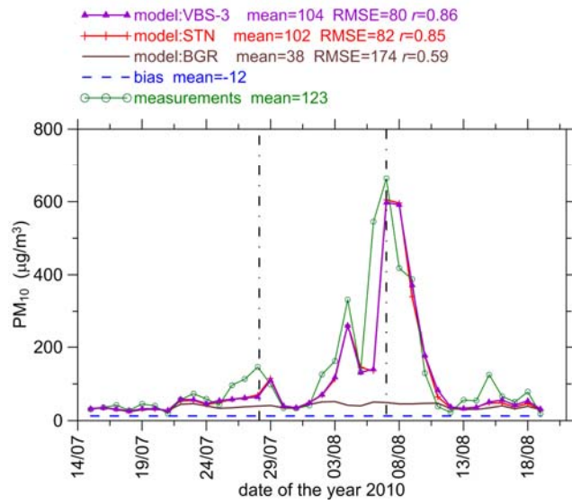
Figure 4. The same as in Fig. 3 but for PM_{10} concentrations, except that in addition to results for the STN and BGR runs, this figure also shows (by a purple line) results for the VBS-3 run.
