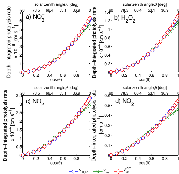
Figure 7. Depth-integrated photolysis rate coefficient at various solar zenith angle for different species within snowpack BaseC, ( \rho = 0.4 \text{ g cm}^{-3} , [\text{BC}] = 4 \text{ ng(C) g}^{-1} and \sigma_{\text{scatt}} = 25 \text{ m}^2 \text{ kg}^{-1} ). a) depth-integrated photolysis rate coefficient of the \text{NO}_3^- anion; b) depth-integrated photolysis rate coefficient of \text{H}_2\text{O}_2 ; c) depth-integrated photolysis rate coefficient of the \text{NO}_2^- anion; d) depth-integrated photolysis rate coefficient of \text{NO}_2 ; blue circle – v_{\text{TUV}} , computed by TUV; green cross – v_{z_e} , calculated by e -folding depth method; pink diamond – v_{z_e}^{\text{Corr}} , corrected v_{z_e} by coefficients listed in Table 4.
