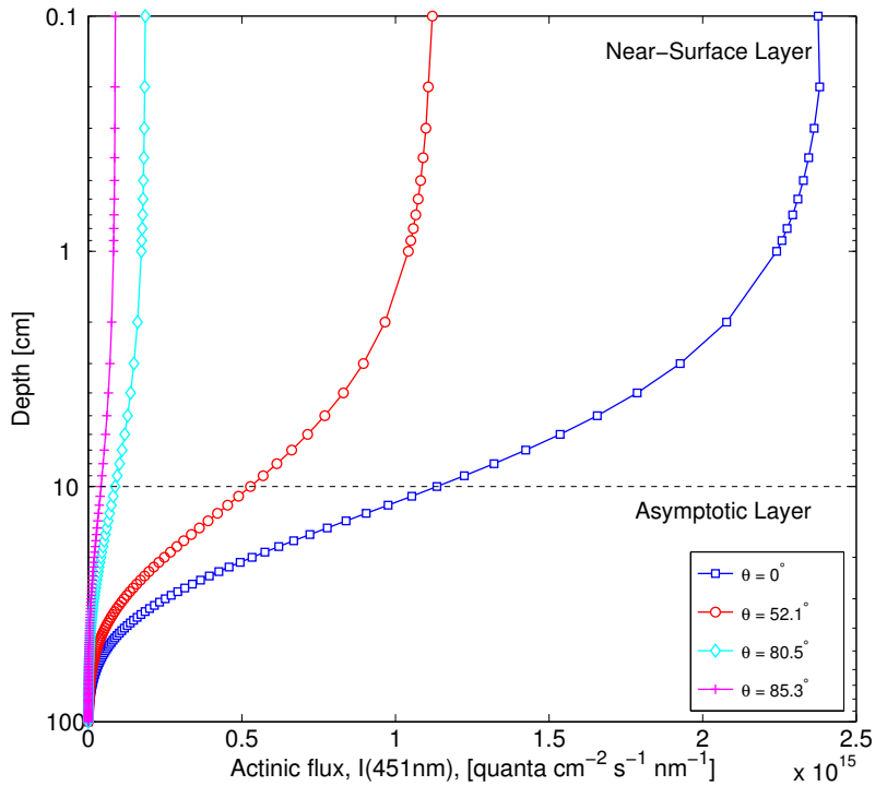
Figure 1. Depth profile within ‘cold polar snow’ (Base Case: \rho=0.4 \text{ g cm}^{-3} , [\text{BC}]=4 \text{ ng(C) g}^{-1} and \sigma_{\text{scatt}}=25 \text{ m}^2 \text{ kg}^{-1} ) of actinic flux, I , at \lambda=451 \text{ nm} at different solar zenith angles \theta .
