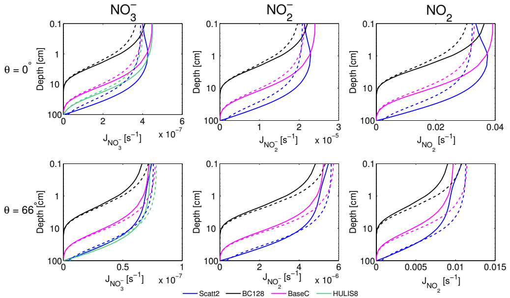
Figure 6. Photolysis rate coefficient for the \text{NO}_3^- anion (a & d), the \text{NO}_2^- anion (b & e) and \text{NO}_2 (c & f) computed by TUV (solid line) and z_e method (dashed line) at two different solar zenith angles, \theta , at 0^\circ (top row) and 66^\circ (bottom row). Maximum and minimum depth-integrated photolysis rate coefficient ratio occurred at \theta = 0^\circ and \theta \sim 66^\circ respectively. Blue is the “melting snow”, Scatt2, ( \rho = 0.4 \text{ g cm}^{-3} , [\text{BC}] = 4 \text{ ng(C) g}^{-1} and \sigma_{\text{scatt}} = 2 \text{ m}^2 \text{ kg}^{-1} ); Black is the “heavily black carbon polluted snow”, BC128, ( \rho = 0.4 \text{ g cm}^{-3} , [\text{BC}] = 128 \text{ ng(C) g}^{-1} and \sigma_{\text{scatt}} = 25 \text{ m}^2 \text{ kg}^{-1} ); Magenta is the “BaseC snow”, BaseC, ( \rho = 0.4 \text{ g cm}^{-3} , [\text{BC}] = 4 \text{ ng(C) g}^{-1} and \sigma_{\text{scatt}} = 25 \text{ m}^2 \text{ kg}^{-1} ); and Green is the “HULIS polluted snow” HULIS8 ( \rho = 0.4 \text{ g cm}^{-3} , [\text{HULIS}] = 8 \text{ ng g}^{-1} and \sigma_{\text{scatt}} = 25 \text{ m}^2 \text{ kg}^{-1} ). Surface (depth = 0 cm) values of photolysis rate coefficient from “RT method” and “ z_e method” are the same (see Eq. 8 for calculation of J_{\text{TUV}} ).
