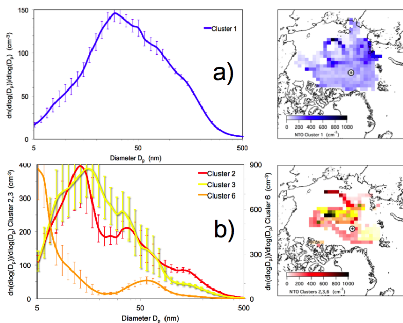
Fig. 8 Left: Average particle number size distributions of the four clusters of horizontal trajectory coordinates, combined with particle size distributions in the subpopulation “Open water”. The clusters are separated into a) Pack ice low, b) Pack ice high. Error bars give one standard deviation about the group average. Blue= Cluster 1; Yellow= Cluster 3. Right: Corresponding regional distributions of median total number concentrations, (NTO, \text{cm}^{-3} ). The color saturation indicates the total number associated with the respective trajectory. Only geocells with at least 25 trajectory hits are shown. The symbol indicates the North Pole.
