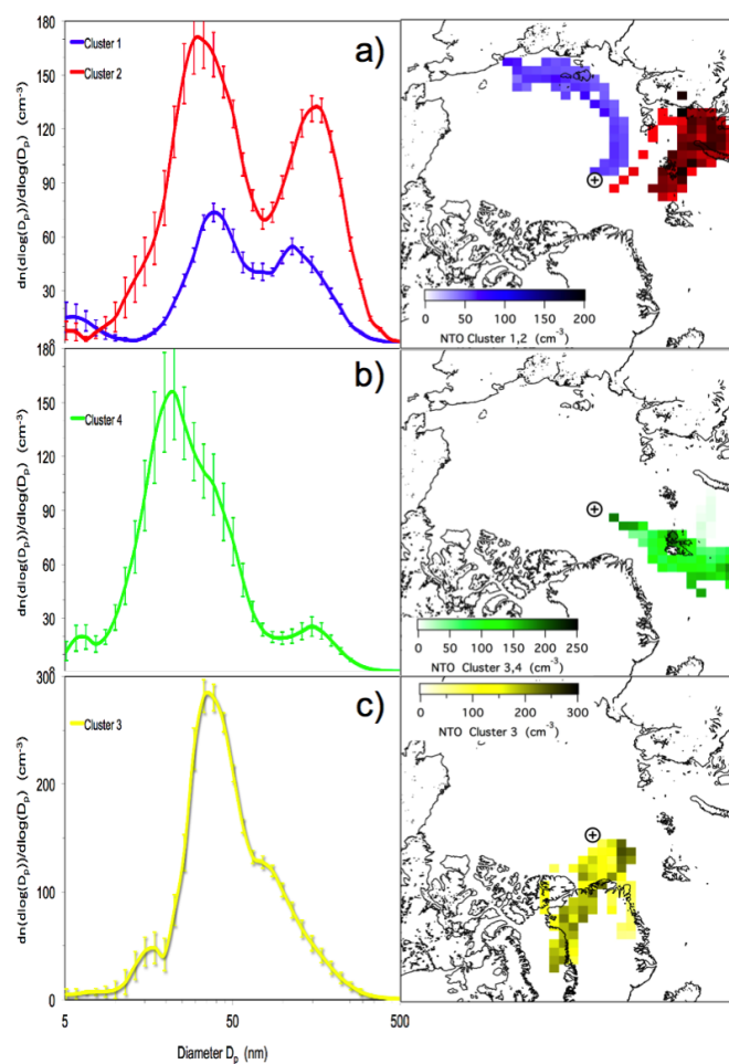
Fig. 7 Left: Average particle number size distributions of the four clusters of horizontal trajectory coordinates, combined with particle size distributions in the subpopulation “Marginal ice”. The clusters are separated into a) marine, b) Spitsbergen and c) Greenland. Error bars give one standard deviation about the group average. Blue= Cluster 1; Yellow= Cluster 3; Green = Cluster 4. Right: Corresponding regional distributions of median total number concentrations, (NTO, \text{cm}^{-3} ). The color saturation indicates the total number associated with the respective trajectory. Only geocells with at least 25 trajectory hits are shown. The symbol indicates the North Pole.
