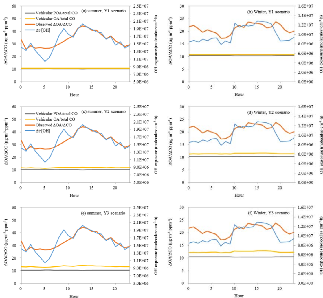
Fig. 7. Diurnal variations of observed \Delta OA/\Delta CO in the atmosphere (red line), OH exposures (blue line), and the ratios of vehicular POA emission (grey line) and OA formation (orange line) to total CO emissions with the SOA yields in three scenarios (Y1, Y2 and Y3) in summer and winter in the urban area of Shanghai for the year of 2013.
