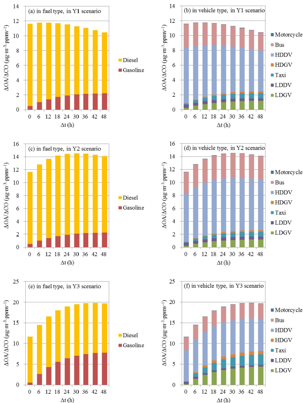
Fig. 8. Contributions of vehicle emissions to OA formation ratios in different vehicle and fuel types in Y1, Y2 and Y3 scenarios with the changes of photochemical ages.
