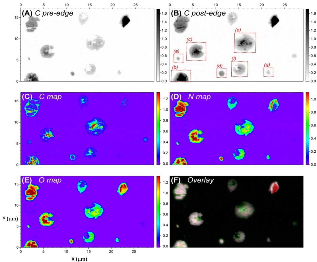
Figure 6. STXM images and elemental maps of representative particles in the coarse mode range with some smaller accumulation mode particles. The particles shown here represent a volume equivalent diameter range of 0.6 -1.9 \mu\text{m} . (A and B) carbon pre- and post-edge images, (C) carbon elemental map, (D) nitrogen map, (E) oxygen map, and (F) overlay of C (green), N (blue), and O (red) maps. Axes in A-E display image dimensions in \mu\text{m} . Optical density (color code) is displayed for individual maps. Red boxes and labels in (B) highlight internally mixed particles with ammoniated sulfate and variable amounts of organics.
