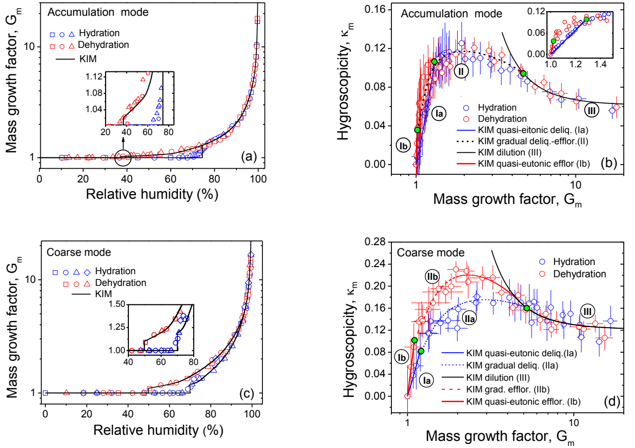
Figure 8. Hygroscopic properties of accumulation (a,b), and coarse (c,d) modes of ZOTTO aerosol samples: (a, c) mass growth factors ( G_m ) observed as a function of relative humidity compared to KIM; (b, d) mass-based hygroscopicity parameters ( \kappa_m ) calculated as a function of mass growth factor. The data points and error bars are from FDHA experiments of hydration (blue symbols) and dehydration (red symbols). The labels I (Ia,Ib), II (IIa,IIb) and III indicate different regimes of hygroscopicity (Eqs.(6)-(8)); the borders of the corresponding fit intervals are indicated by green circles (b, d). Varied symbols in panels (a) and (c) represent different experimental runs on the same sample.
