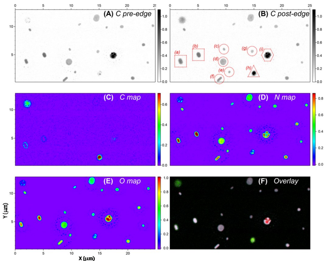
Figure 5. STXM images and elemental maps of representative accumulation mode particles in the ZOTTO aerosol samples. The particles shown here represent a volume equivalent diameter range of 0.3 - 0.6 \mu\text{m} . (A and B) carbon pre- and post-edge images, (C) carbon elemental map, (D) nitrogen map, (E) oxygen map, and (F) overlay of C (green), N (blue), and O (red) maps. Axes in A-E display image dimensions in \mu\text{m} . Optical density (color code) is displayed for individual maps. Red boxes and labels in (B) exemplify the most common particle types in STXM samples: a and b show internally mixed particles with ammoniated sulfate core and organic coating; c - g show mostly purely inorganic ammoniated sulfate particles; i shows ammoniated sulfate with potassium; h shows a C-rich particle with small inorganic content.
