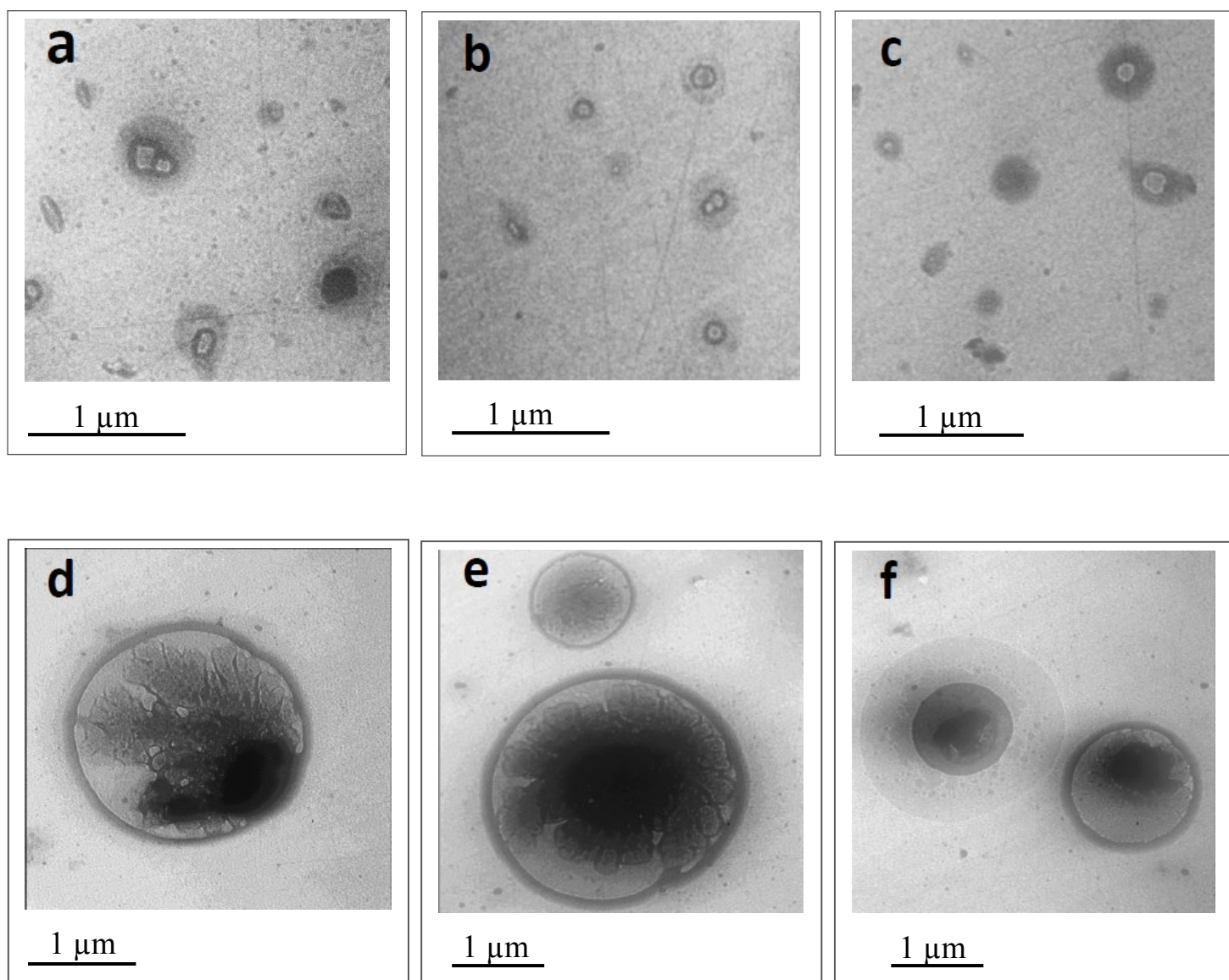
Figure 7. TEM micrographs of submicron (a, b, c) and supermicron (d, e, f) particles.
