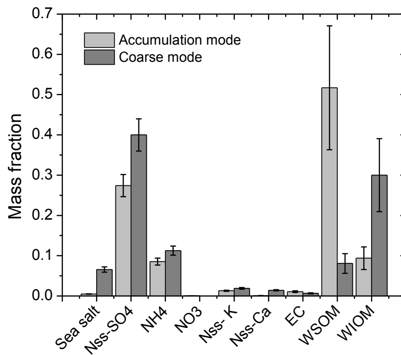
Figure 4. Average mass fraction of organic and inorganic species in the accumulation and coarse modes of the ZOTTO samples.
