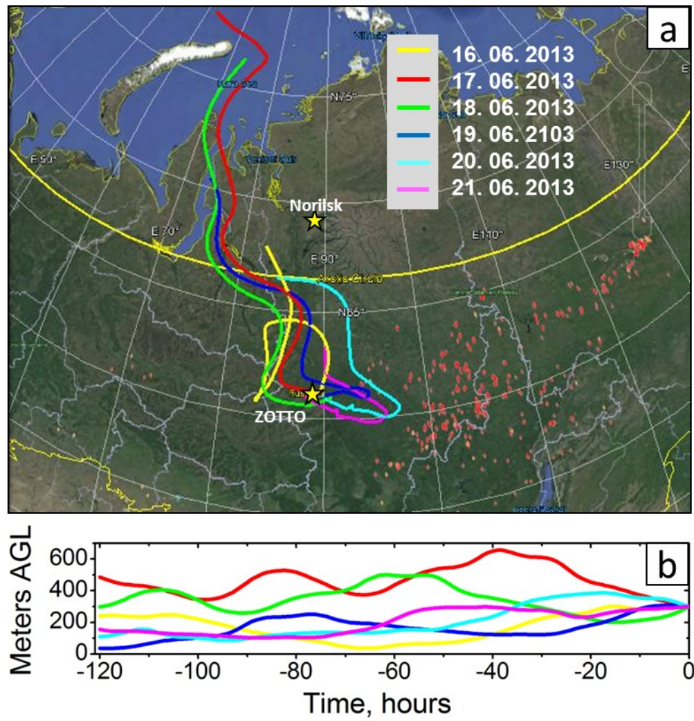
Figure 1. (a) 120-hour HYSPLIT airmass backward trajectories during the sampling period at ZOTTO at 300 m from 16 to 21 June 2013 and (b) their height above ground level (AGL). Red dots indicate the fire locations within the sampling period.
