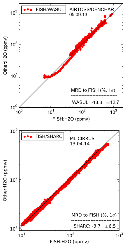
Figure 10. Scatterplot of FISH–WVMR vs.: WASUL (red) during Airtoss/DENCHAR 2013 (top panel) and SHARC during ML-Cirrus 2014 (bottom panel). The mean relative deviation (MRD) with SD to FISH is given for each individual instrument.
