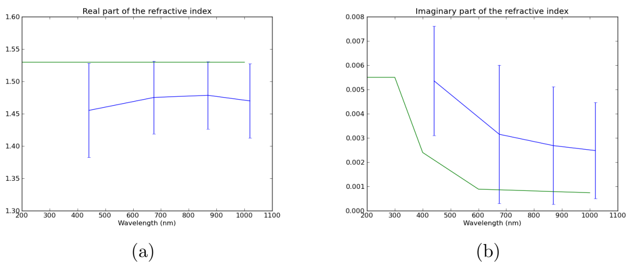
Fig. 8. (a) Real part of the refractive index inverted from the AERONET measurements averaged for June 22-24 and July 2-4 (blue line: average and extreme of the 29 available hourly AERONET values) and value used by CHIMERE (green line). The blue error bars indicate the extreme values measured by AERONET during these six days. (b) Same as (a) but for the imaginary part of the refractive index.
