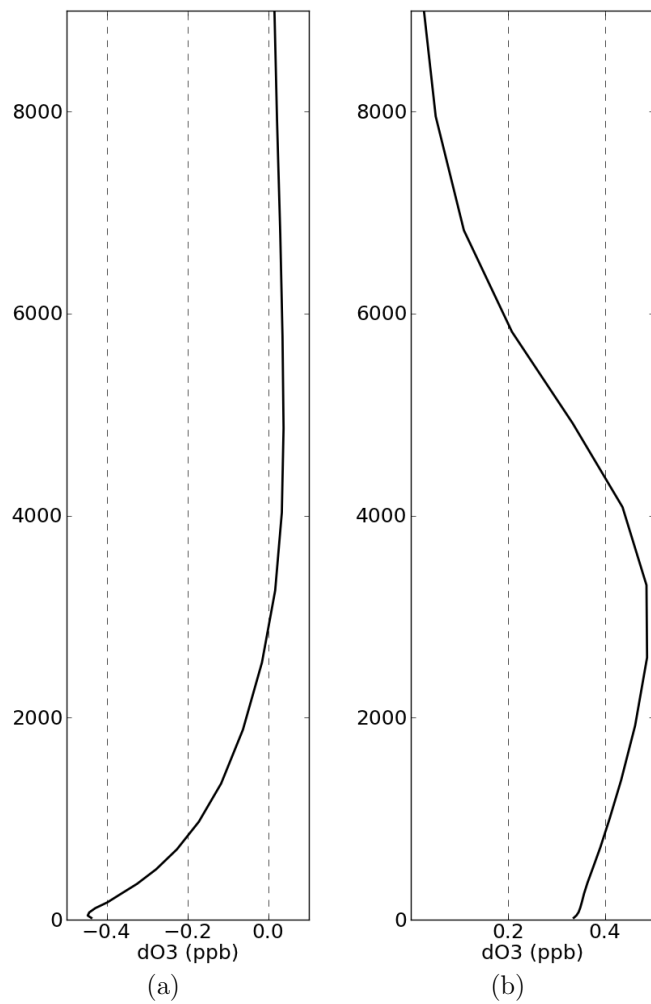
Fig. 19. (a) [O_3]_{REF} - [O_3]_{NA} as a function of the height in meters above the ground level (m.a.g.l.), averaged for the Mediterranean basin ( 35N-45N \times 5W-35E ) for all the simulation period (June 6 - July 15); and (b) same as (a) but for the Saharan area ( 5N-30N \times 10W-30E ).
