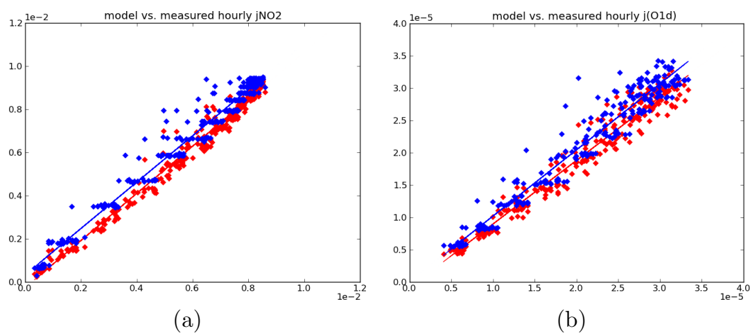
Fig. 15. (a) Scatter plot of hourly modelled J(\text{NO}_2) versus measured J(\text{NO}_2) at Lampedusa for 698 points with valid daytime measurements of J(\text{NO}_2) . Red diamonds represent the J(\text{NO}_2) values in the REF simulation, blue diamonds the J(\text{NO}_2) values in the NA simulation, with the respective regression lines; (b) same as (a) for J(\text{O}^1\text{D}) , with 610 valid data points.
