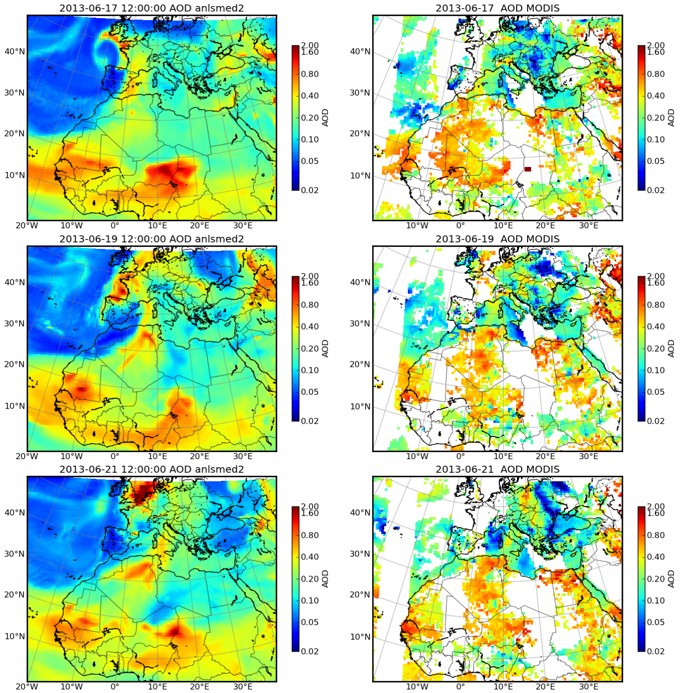
Fig. 6. AOD at 550 nm in the CHIMERE model (left column) and as observed by MODIS AQUA and TERRA, for June 17, 19 and 21, 2013.
