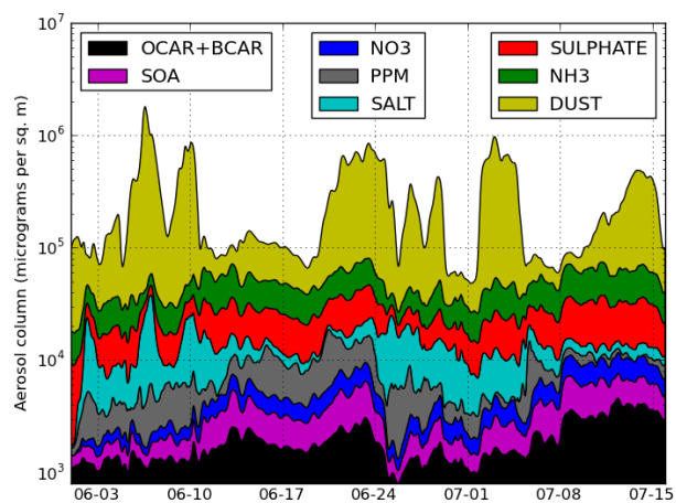
Fig. 11. Cumulative plot of the total aerosol mass load ( \mu g m^{-2} ) for the following groups of species : Organic and black carbon (OCAR+BCAR), secondary organic aerosols (SOA), nitrates (NO3), primary anthropogenic particulate matter (PPM), sea-salt (SALT), sulphate, ammonium (NH3) and mineral dust (DUST).
