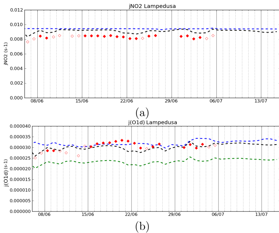
Fig. 13. (a) Daily maximal values of modelled J(\text{NO}_2) in \text{s}^{-1} for the REF simulation (black dashed line) and the NA simulation (blue dashed line), and measured values of the daily maxima (red diamonds). The days when significant effect of clouds was visible on the spectrometer measurements are signalled on the plot by an empty red diamond. (b) same as (a) for J(\text{O}^1\text{D}) . The green dashed line represents the J(\text{O}^1\text{D}) values in the O3+ simulation.
