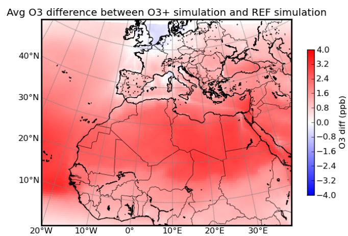
Fig. 20. Difference (ppb) in the concentration of ozone in the lowest model layer between the O3+ simulation and the REF simulation.
