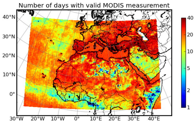
Fig. 5. Number of days with available MODIS measurements between Jun. 6 and July 15
