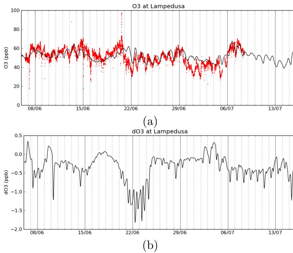
Fig. 17. (a) Time series for ozone concentration (ppb) in the reference simulation in Lampedusa (black line) along with measured values (red dots); and (b), effect of the optical screening by the aerosols on the ozone concentration, computed as dO_3 = [O_3]_{ref} - [O_3]_{NA} .
