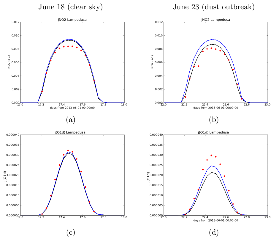
Fig. 14. (a) Hourly modelled values of J(\text{NO}_2) in the REF simulation (black line) and in the NA simulation (blue line), and hourly measured values of J(\text{NO}_2) (red diamonds), for June 18, 2013. (b) same as (a) but for June 23; (c): Hourly modelled values of J(\text{O}^1\text{D}) in the REF simulation (black line) and in the NA simulation (blue line), and hourly measured values of J(\text{O}^1\text{D}) (red diamonds), for June 18, 2013; and (d): same as (c) but for June 23.
