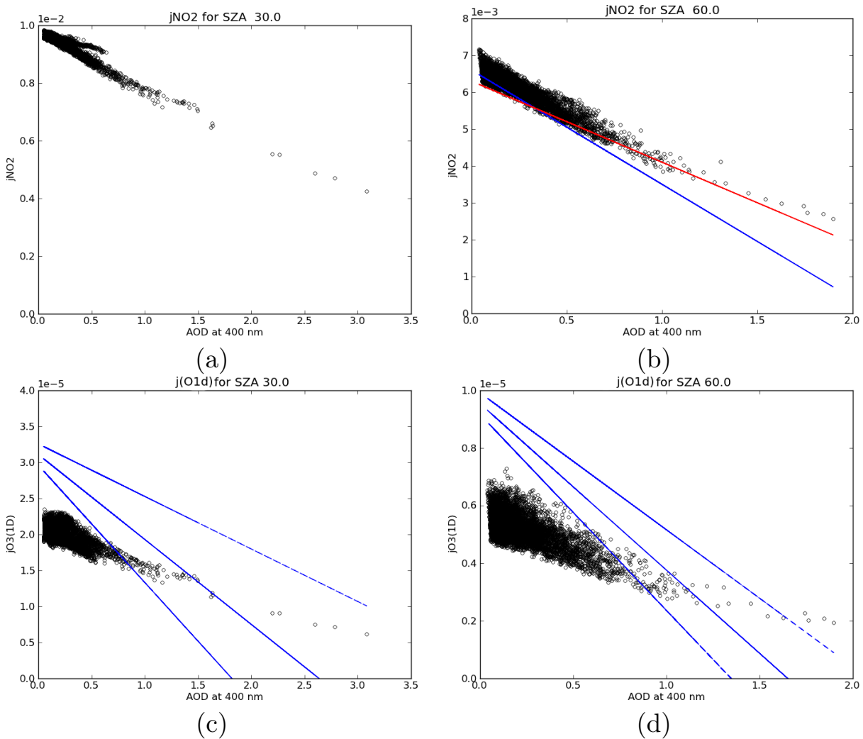
Fig. 16. Scatter plots of J(\text{NO}_2) (a,b) and j\text{O}_3(1\text{D}) (c,d) at the lowest model level versus the AOD, for clear-sky conditions and latitudes comprised between 32.5^\circ\text{N} and 38.5^\circ\text{N} . For the purpose of comparison, on panel (b), the regression relationships found by Gerasopoulos et al. (2012) with field data are reported in blue (non-dust aerosols) and red (dust aerosols). On panels (c) and (d) the regression lines by Casasanta et al. (2011) are indicated along with their uncertainty margin.
