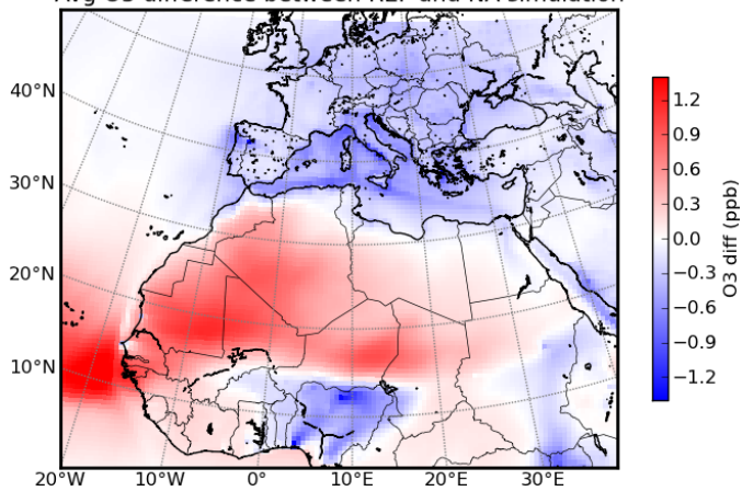
Fig. 18. (a) Average difference of J(\text{O}^1\text{D}) between REF and NA (%) for all the simulation period (June 6 - July 15) ; (b) Average difference of J(\text{NO}_2) between REF and NA (%) for all the simulation period ; and (c) Average difference of ozone concentration between REF and NA for all the simulation period (ppb).
