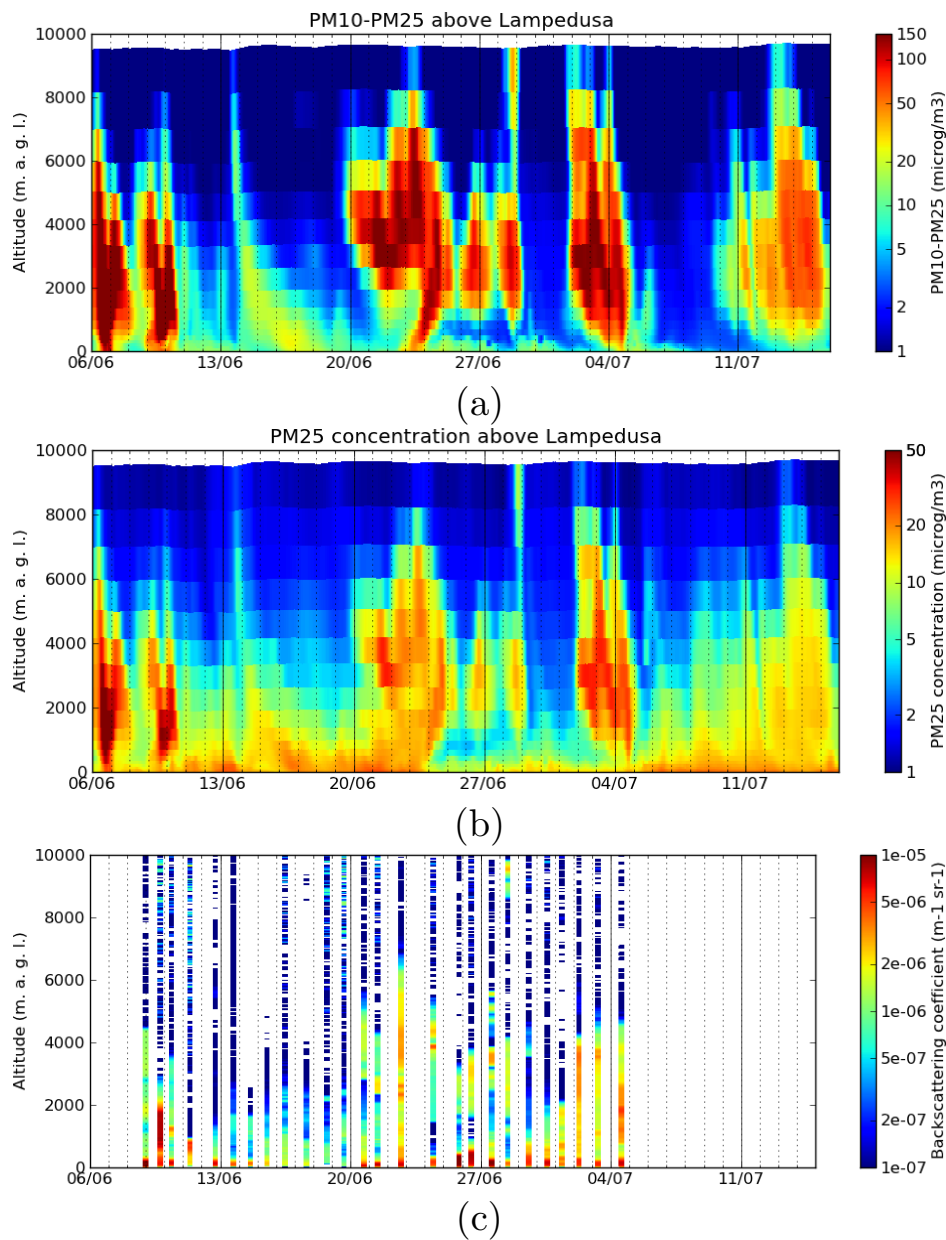
Fig. 9. (a) Evolution of modelled coarse particles concentrations ( PM_{10} - PM_{2.5} ) above Lampedusa ; (b) same as (a) but for the fine particles ( PM_{2.5} ) ; and (c) : LIDAR backscatter coefficient above Lampedusa. Each selected LIDAR profile is represented by a column of fixed width centered on the instant of the measurement, representing the backscatter coefficient (color levels).
