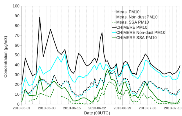
Fig. 10. Modelled speciation of PM 10 aerosols in the first model layer compared to measurements for total PM 10 (black lines), non-dust PM 10 (blue lines) and sea-salt aerosols (green lines).
