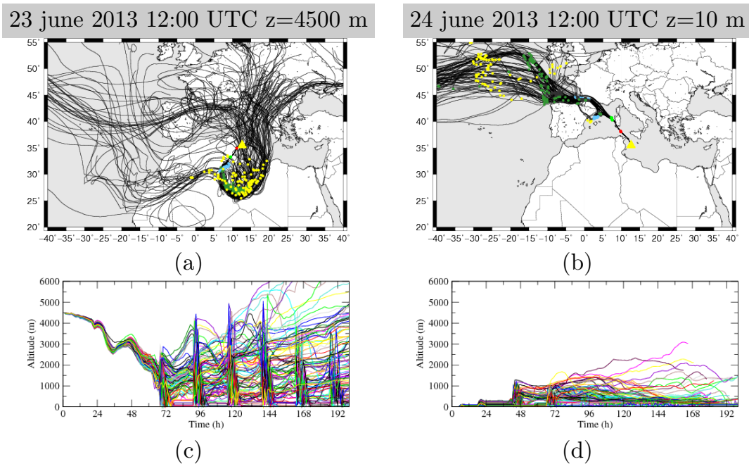
Fig. 12. (a) Backplume starting above Lampedusa for June 23, 12UTC at 4500 m altitude. The yellow triangle represents Lampedusa, the starting location of the backplume. The colored dots correspond to the number of hours before the starting time: red=12, green=24, blue=48, dark green=72, yellow=96 (b) same as (a) but for June 24, 12 UTC at 10 m altitude. (c) altitude of the backplume starting above Lampedusa for June 23, 12UTC at 4500 m altitude, and (d), altitude of the backplume starting above Lampedusa for June 24, 12UTC at 10 m altitude.
