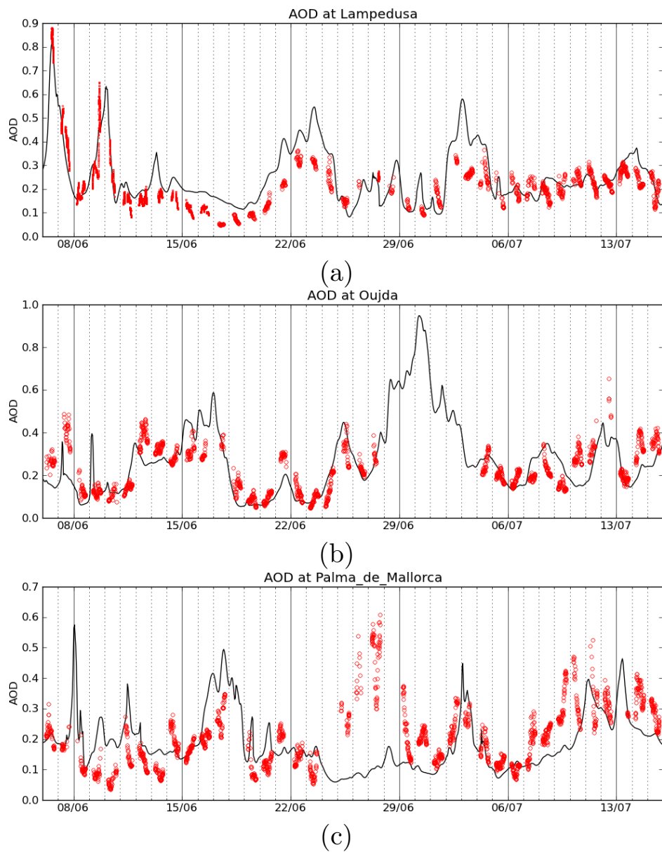
Fig. 7. Evolution of modeled AOD (black lines) at 400 nm above Lampedusa, Oujda and Palma de Mallorca, compared to the AERONET AOD interpolated at 400 nm (red circles). For Lampedusa, AERONET data is completed with MFRSR data (red dots) when the AERONET data was not available.
