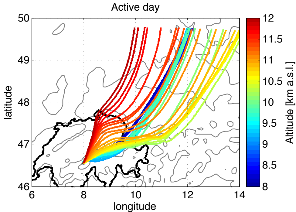
Figure 11. Path of the trajectories arriving at Jungfraujoch on 12 March 2012 3 UTC.
