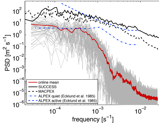
Figure 4. Power spectral density (PSD) of the vertical wind calculated from online trajectories (grey) passing above Jungfraujoch at 09 UTC between 10.0 km and 11.5 km. Red curve: average of online trajectories. Solid and dashed black lines: PSDs of vertical velocities measured during SUCCESS (Toon et al., 1998) and MACPEX (Rollins et al., 2014), respectively. Blue dashed and dashed-dotted lines: data from the ALPEX campaign for active and quiet days, respectively (Kuettner, 1981).
