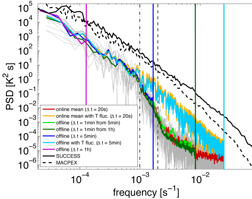
Figure 3. Power spectral densities (PSDs) of the temperature calculated for trajectories arriving above Jungfraujoch at 09 UTC at 10.0-11.5 km, where the cirrus cloud was observed by the Lidar. (a): Grey lines: PSDs of individual 20-s online trajectories. Red line: average of the online trajectories. Orange: online trajectory with superimposed temperature fluctuations. Light green: offline trajectories based on 5-min model output, interpolated to 1 min resolution. Dark green: based on 1-h model output, interpolated to 1 min. Dark blue: offline trajectories based on 5-min COSMO-2 model output. Light blue: offline trajectories based on 5-min COSMO-2 model output with superimposed small scale temperature fluctuations. Cyan: based on 5-min model output, interpolated to 1 min resolution. Purple: offline trajectories based on 1-h model output. Colored vertical lines: Nyquist frequency for each specific temporal resolution. Black solid curve: PSD derived from aircraft data sampled during the SUCCESS campaign. Black dashed curve: same for the MACPEX campaign. Dashed vertical line: maximum frequency that can be resolved on the COSMO-grid given the finite horizontal resolution and the mean horizontal velocity along the trajectories ( f_{max} = 17.4 \text{ m/s} / (4 \times 2.2 \text{ km}) \approx 2 \cdot 10^{-3} \text{ s}^{-1} ). Dashed-dotted vertical line: Cut-off frequency using 8\Delta x as effective model resolution.
