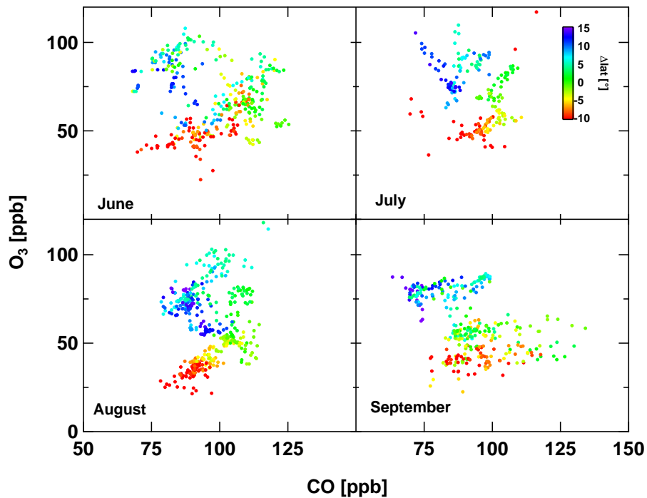
Figure 6. Monthly distributions of O_3 vs. CO during the summer monsoon season 2008. Points are colour-coded by relative position within the UTAC, as determined by \Delta lat (see also Sect. S6).
