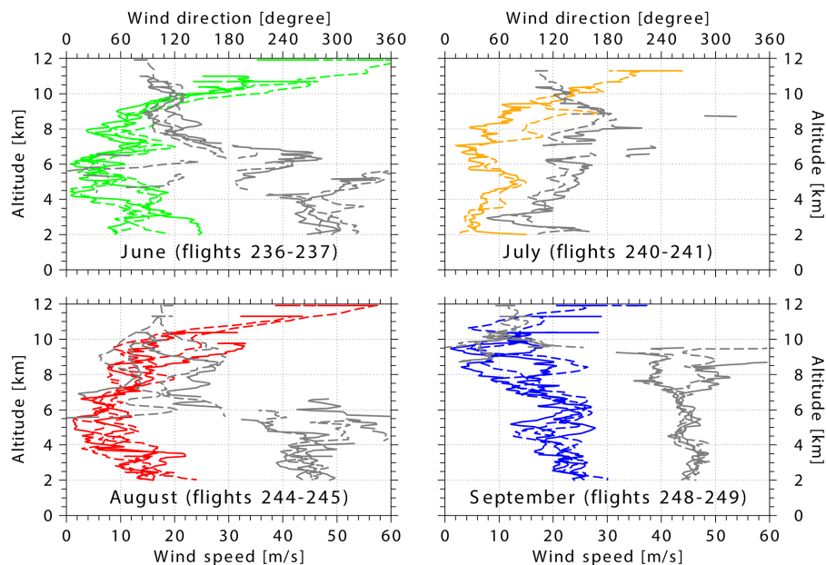
Figure 7. Wind speed (coloured lines, lower x axis) and wind direction (grey lines, upper x axis, 90^\circ means wind from the east, 180^\circ from the south, 270^\circ from the west) from the measurements onboard the CARIBIC aircraft for the descent into (solid lines) and ascent from (dashed lines) Chennai. Only data south of 16^\circ N and above 2 km altitude is plotted. Chennai is at 12.99^\circ N, 80.18^\circ E.
