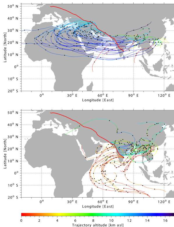
Figure 9. 10 day backward trajectories for CARIBIC flight 244 to Chennai on 13 August 2008. Upper panel: trajectories north of the wind reversal at 26.6^{\circ} N. Lower panel: trajectories south of the wind reversal. Every second trajectory is plotted for clarity. The colour indicates the trajectory altitude and the black dots mark 24 h time steps along the trajectories. The CARIBIC flight track is shown by the thick red line (see also Figs. S29–S31).
