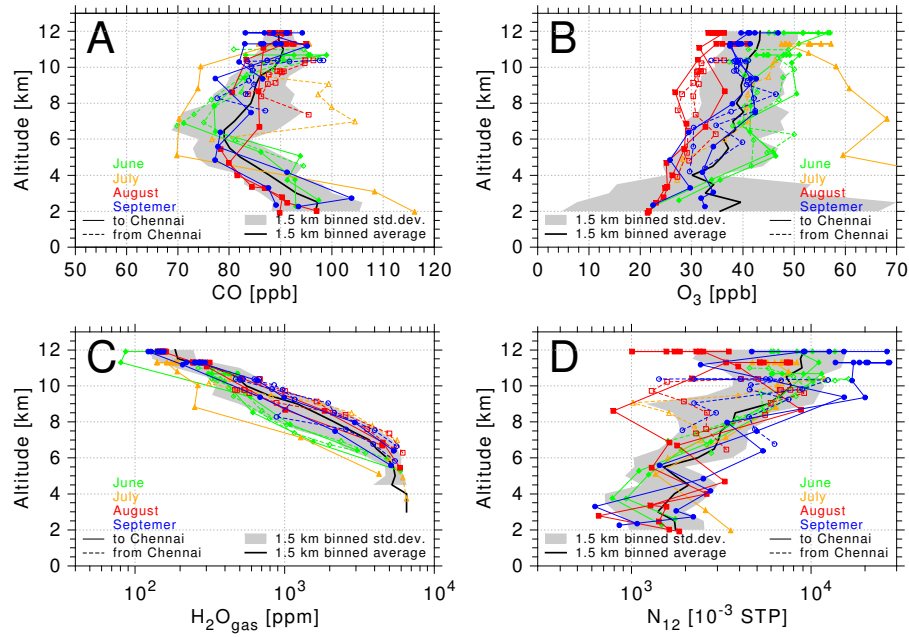
Figure 9. Vertical profiles of CO ( A ), O_3 ( B ), water vapour ( C ) and number concentration of Aitken mode aerosol particles N_{12} at STP (273.15 K, 1013.25 hPa; D ) between 2 km and 12 km during descent into (solid lines and filled symbols) and ascent from (dashed lines and open symbols) Chennai. The colours indicate the flight month, the black line is the mean over all flights and the grey shading indicates the 1- \sigma standard deviation around the mean (both calculated over moving 1.5 km altitude bins). Note the logarithmic x axis for water vapour ( C ) and aerosol particles ( D ).
