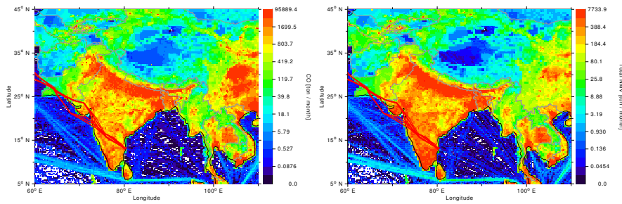
Figure 2. Emissions of CO (left panel) and non-methane volatile organic compounds (right panel) for August 2008 from the Regional Emission inventory in ASia (REAS) v2.1 (Kurokawa et al., 2013) including the update from 14 November 2013. The red lines mark the CARIBIC flight tracks for June to September 2008.
