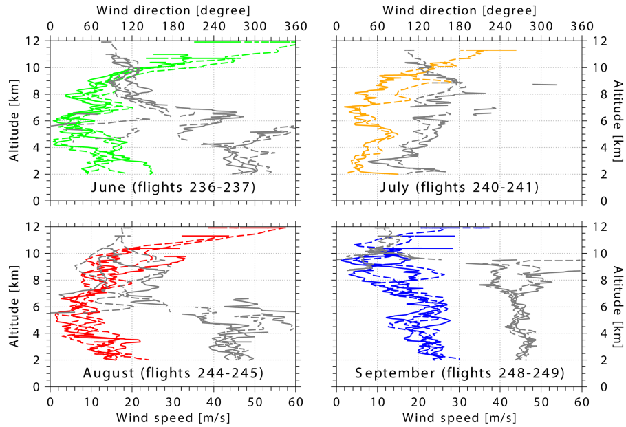
Figure 8. Wind speed (coloured lines, lower x axis) and wind direction (grey lines, upper x axis, 90^\circ means wind from the east, 180^\circ from the south, 270^\circ from the west) as recorded by the CARIBIC aircraft for the descent into (solid lines) and ascent from (dashed lines) Chennai. Only data south of 16^\circ N and above 2 km altitude is plotted. Chennai is at 12.99^\circ N, 80.18^\circ E.
