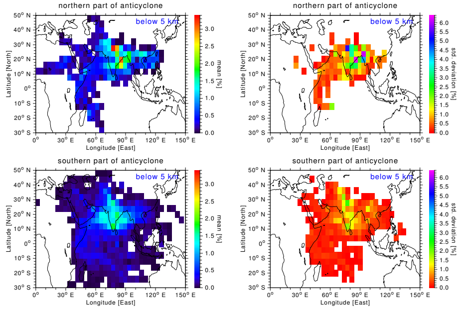
Figure 11. Distribution of source regions for all the CARIBIC flights. The colour code shows the percentage of trajectory points that were below 5 km altitude in the preceeding 10 days per 4^\circ \times 4^\circ grid box. Upper left panel: source regions for trajectories starting north of the wind reversal. Lower left panel: source regions for trajectories starting south of the wind reversal. Right panels show the corresponding standard deviation of the percentages in the monsoon months June to September per grid box for all grid boxes reached by trajectories from at least two months (see also Figs. S26–S29).
