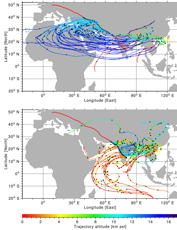
Figure 10. 10 day backward trajectories for CARIBIC flight 244 to Chennai on 13 August 2008. Upper panel: trajectories north of the wind reversal at 26.6^{\circ} N. Lower panel: trajectories south of the wind reversal. Every second trajectory is plotted for clarity. The colour indicates the trajectory altitude (in km above sea-level) and the black dots mark 24 h time steps along the trajectories. The CARIBIC flight track is shown by the thick red line.
