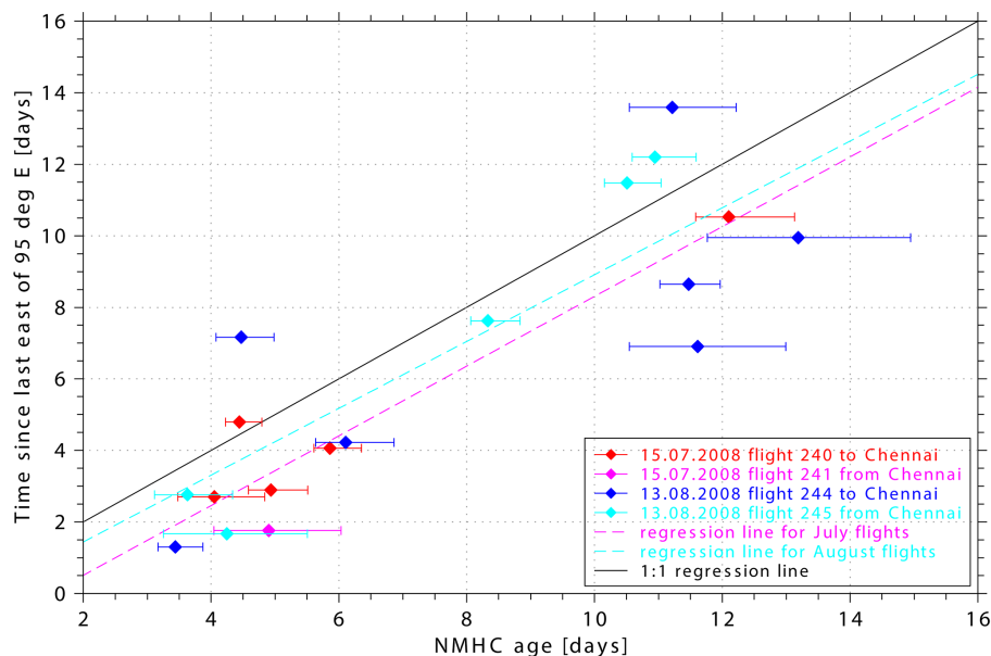
Figure 15. Comparison of the photochemical age of air estimated from NMHC ratios and the time the air had last been east of 95° E according to the FLEXPART trajectory calculations. Shown are the mean chemical age together with the minimum and maximum age determined from the propane/ethane, n-butane/ethane and n-butane/propane ratios. The colours indicate different flights (see legend). The black line indicates perfect agreement of both age estimates while the dashed lines indicate linear least-square regression lines of transport time and chemical ages derived from the different NMHC ratios (magenta regression lines for July, light blue for August flights).
