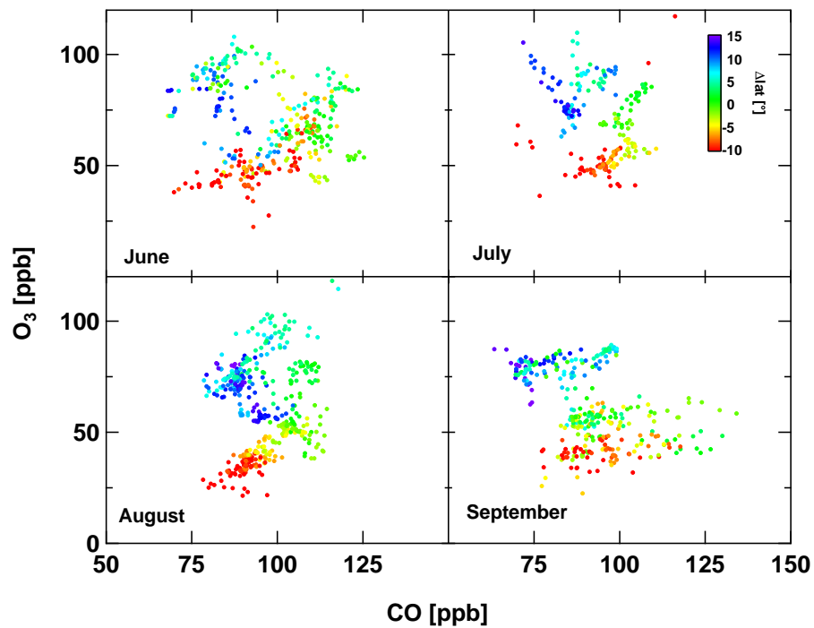
Figure 7. Monthly distributions of O_3 vs. CO during the summer monsoon season 2008. Points are colour-coded by relative position within the UTAC, as determined by \Delta lat (see also Sect. S6).
