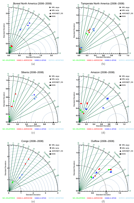
Figure 7. Taylor diagrams for comparison of simulations HAM2.2-AEROCOM, HAM2.2-GFAS and SOFIEV-MODIFIED to satellite observations (MODIS NRL Aqua, MODIS NRL Terra) and ground-based observations (AERONET_DS, MAN), see text for more detailed description of simulation set-ups and observational data sets. The NO-WILDFIRES scenario excludes all wildfire emissions.
