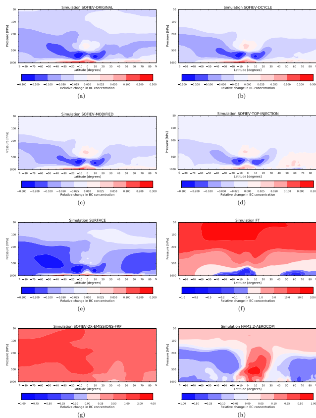
Figure 3. Mean relative changes in zonal mean BC concentrations for 2005–2011. All relative changes refer to the standard implementation of prescribed emission heights combined with GFASv1.1 emissions (simulation HAM2.2-GFAS). A more detailed description of the simulation set-ups is provided in Table 1.
