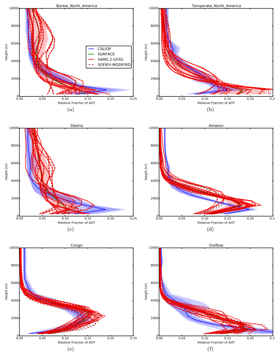
Figure 8. Regional AOT profiles averaged for 2006–2011 for CALIOP observations (solid blue line), simulation HAM2.2-GFAS (bold solid red line), simulation SOFIEV-MODIFIED (bold dashed dark red line) and simulation SURFACE (solid green line). Thin red lines indicate individual multi-year monthly means; red shading represents one SD of monthly variations for model simulation HAM2.2-MODIFIED. Dark blue shading indicates one SD of CALIOP monthly means; light blue shadings indicate minimum and maximum monthly means for CALIOP observations. All vertical lines represent relative AOT fractions at 532 nm (CALIOP) respectively at 550 nm (model simulations) of monthly averages for 2006–2011. Relative AOT fractions describe the integrated AOT of individual height layers (500 m intervals for 0–5 km, 1 km intervals for 5–10 km).
