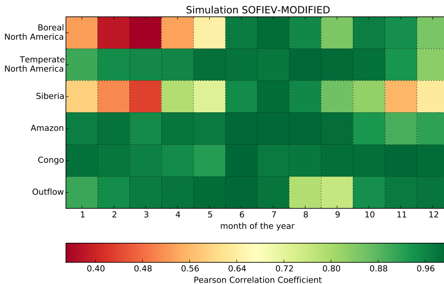
Figure 9. Pearson correlation coefficients of multi-year monthly means for CALIOP vs. SOFIEV-MODIFIED. Correlation coefficients greater than 0.48 are significant on a 95 % confidence interval, while correlations smaller than 0.48 are not significant.
