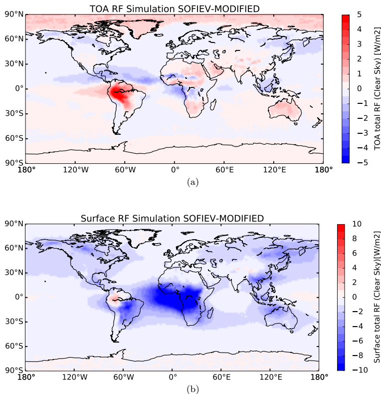
Figure 11. Clear sky Top of Atmosphere radiative forcing (top plot) and clear sky surface radiative forcing introduced by wildfire emissions (lower plot). Both figures show absolute differences of SOFIEV-MODIFIED (applying the plume height parametrization which matches best to observations) and the NO-WILDFIRES scenario for which all wildfire emissions were turned off.
