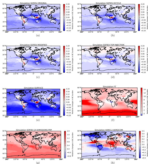
Figure 2. Mean relative changes in BC burden introduced by various implementations of fire emission heights. All relative changes refer to the standard implementation of prescribed emission heights combined with GFASv1.1 emissions (simulation HAM2.2-GFAS). Simulations SOFIEV-ORIGINAL (a), SOFIEV-DCYCLE (b), SOFIEV-MODIFIED (c) and SOFIEV-TOP-INJECTION (d) show different versions of the Sofiev plume height parametrization. Simulation SURFACE (e) represents near surface emissions, simulation FT (f) is based on purely free-tropospheric emissions. SOFIEV-2X-EMISSIONS-FRP (g) assumes a doubling in emissions and FRP. HAM2.2-AEROCOM (h) illustrates the influence of changes in the emission inventory. For a description of settings for simulations (a) to (h), see Table 1.
