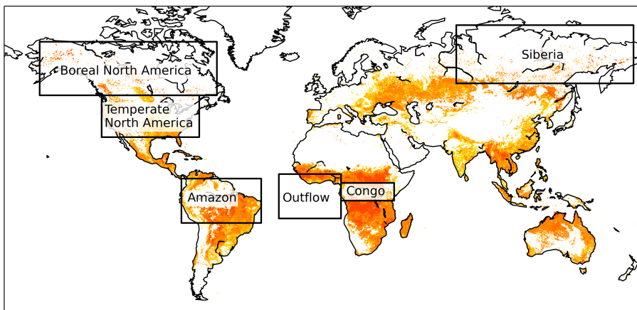
Figure 1. Region specification of major biomass burning areas for comparison of modeled AOT to observations. Color shading represents mean annual assimilated FRP values of GFASv1.1 for 2005–2011. Yellow colors indicate low FRP values, dark red colors indicate high FRP values.
