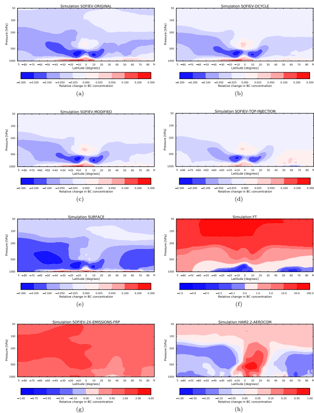
Figure 3. Mean relative changes in zonal mean BC concentrations for 2005–2011. All relative changes refer to the standard implementation of prescribed emission heights combined with GFASv1.1 emissions (simulation HAM2.2-GFAS). A more detailed description of the simulation set-ups is provided in Table 1.
