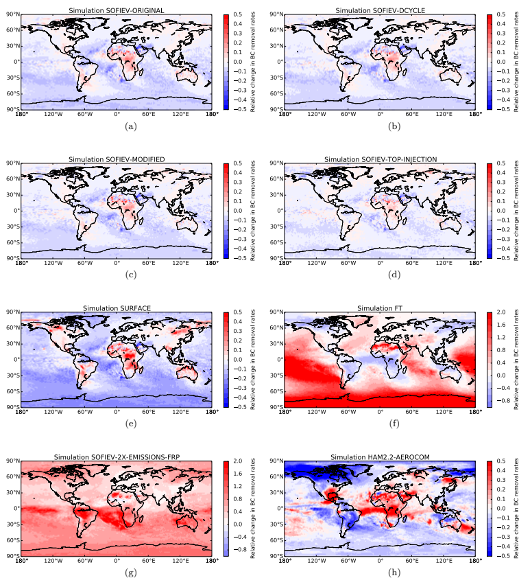
Figure 4. Simulated mean total deposition rates from 2005 to 2011. All relative changes refer to the standard implementation of prescribed emission heights combined with GFASv1.1 emissions (simulation HAM2.2-GFAS). A more detailed description of the simulation set-ups is provided in Table 1.
