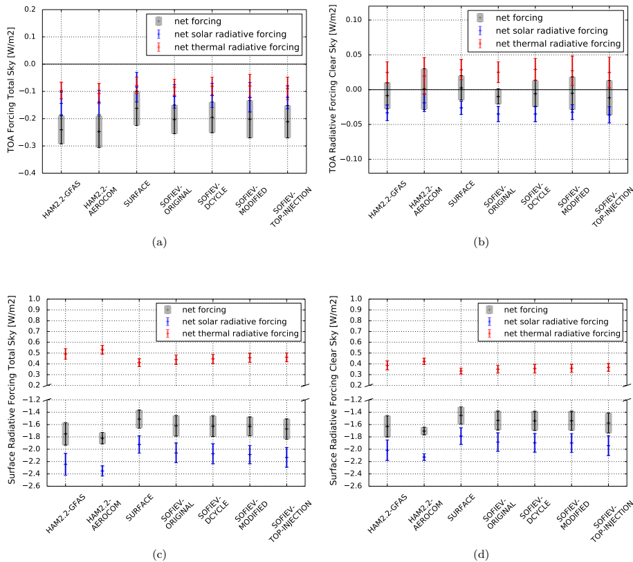
Figure 10. Simulated global mean net Radiative Forcing (RF) for Top Of Atmosphere (TOA) total sky (a), TOA clear sky (b), surface total sky (c) and surface clear sky (d). The RF of all simulations refers to the NO-WILDFIRES scenario. Error bars indicate one SD of monthly mean RF values for 2005–2011. For a detailed description of the simulation set-ups, see Table 1.
