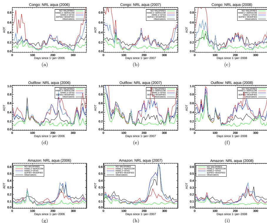
Figure 5. Temporal evolution of regional AOT for standard HAM2.2 plume heights based on GFAS emissions (HAM2.2-GFAS) respectively AEROCOM emissions (HAM2.2-AEROCOM) and a modified plume height parametrization of Sofiev et al. (2012) including a diurnal cycle of fire emissions and fire intensity (simulation SOFIEV-MODIFIED). The NO-WILDFIRES scenario is shown to distinguish wildfire-related biases from others. Observations are MODIS Aqua satellite measurements of AOT. All model data were collocated with the observations prior to averaging.
