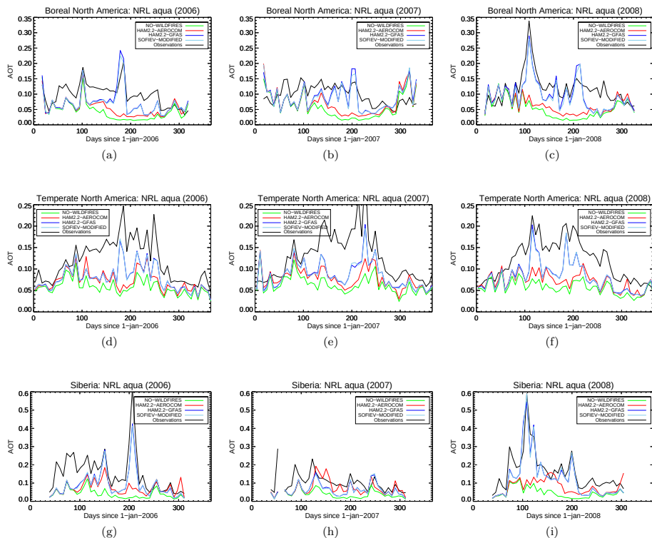
Figure 6. Temporal evolution of regional AOT for standard HAM2.2 plume heights based on GFAS emissions (HAM2.2-GFAS) respectively AEROCOM emissions (HAM2.2-AEROCOM) and a modified plume height parametrization of Sofiev et al. (2012) including a diurnal cycle of fire emissions and fire intensity (simulation SOFIEV-MODIFIED). The NO-WILDFIRES scenario is shown to distinguish wildfire-related biases from others. Observations are MODIS Aqua satellite measurements of AOT. All model data were collocated with the observations prior to averaging.
