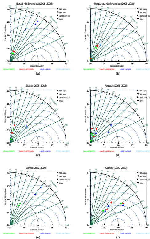
Figure 7. Taylor diagrams for comparison of simulations HAM2.2-AEROCOM, HAM2.2-GFAS and SOFIEV-MODIFIED to satellite observations (MODIS NRL Aqua, MODIS NRL Terra) and ground-based observations (AERONET_DS, MAN), see text for more detailed description of simulation set-ups and observational data sets. The NO-WILDFIRES scenario excludes all wildfire emissions.
