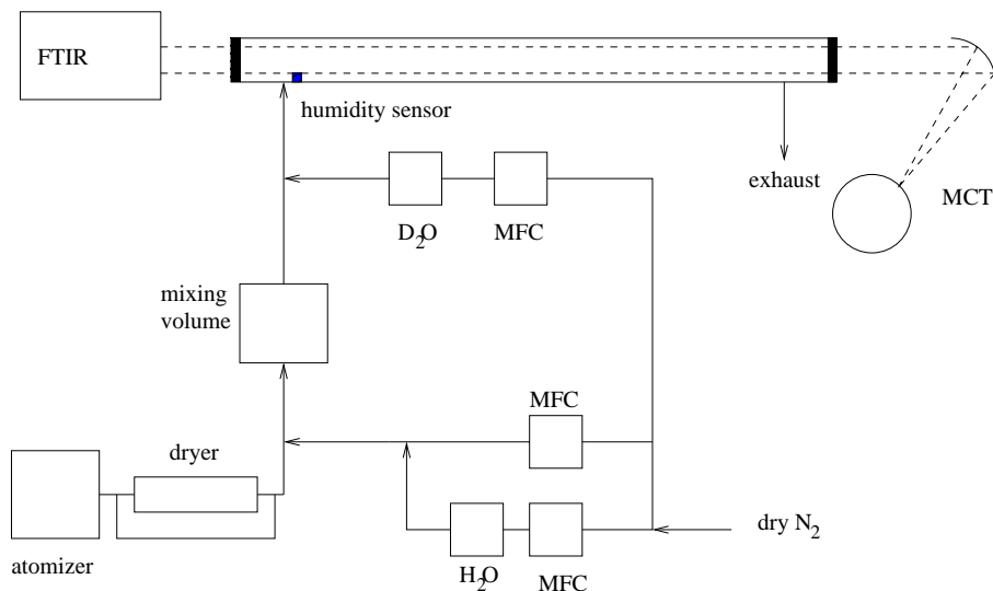
Figure 1. Experimental setup. An atomizer was used to produce particles in an aqueous state or crystalline after removal of condensed phase water in a dryer. H 2 O or D 2 O vapor could then be added to the system from two bubblers coupled to mass flow controllers. The IR spectrum of the aerosol was then determined in a FTIR-coupled flow tube.
