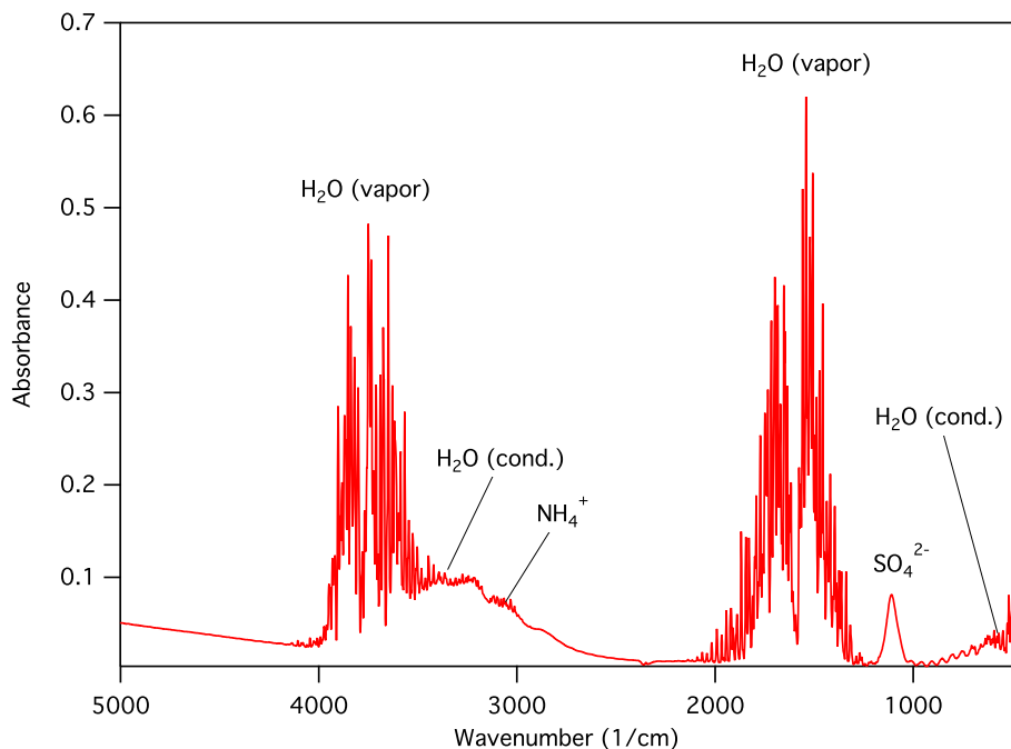
Figure 2. A typical FTIR spectrum of ammonium sulfate at high relative humidity obtained in this experiment. Note the condensed and gas-phase features. The slope at higher wave number corresponds to aerosol scattering.
