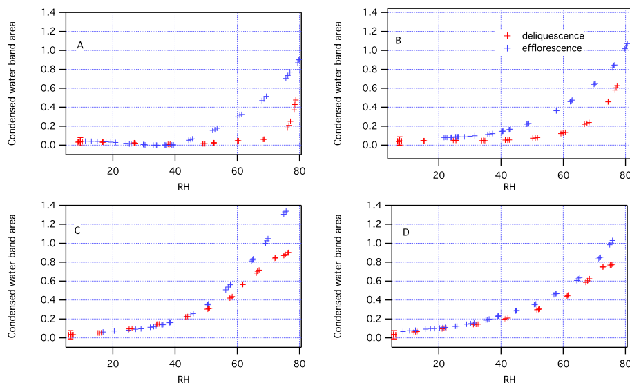
Figure 6. Deliquescence and efflorescence experiments on (\text{NH}_4)_2\text{SO}_4 /glycerol/water ternary mixtures of variable concentrations. (a): pure ammonium sulfate. Note, efflorescence at \sim 35\% RH, deliquescence at \sim 80\% RH. (b): 1 : 3 glycerol/ (\text{NH}_4)_2\text{SO}_4 . Note, no clear efflorescence or deliquescence points. (c): 1 : 2 glycerol/ (\text{NH}_4)_2\text{SO}_4 . Note, no clear efflorescence or deliquescence points. (d): 1 : 1 glycerol/ (\text{NH}_4)_2\text{SO}_4 . Note, no clear efflorescence or deliquescence points.
