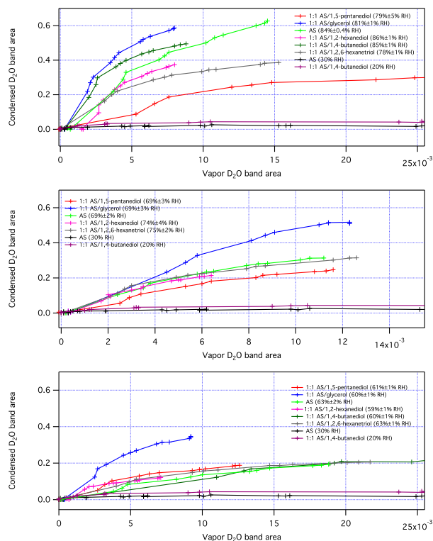
Figure 8. Gas-phase exchange experiments for organic/ (\text{NH}_4)_2\text{SO}_4 mixtures in three RH ranges. Data for pure ammonium sulfate at 30% RH, a crystalline solid, is plotted for reference. No change in the condensed \text{D}_2\text{O} band area is seen in only the two control cases: ammonium sulfate at 30% RH and a 1 : 1 (\text{NH}_4)_2\text{SO}_4 /1,4-butanediol mixture at 20% RH, both of which are below their efflorescence point (i.e., they contain no condensed-phase water). For all particles containing condensed water, an exchange of \text{D}_2\text{O} vapor is apparent. Liquid–liquid phase separation does not exclude water diffusion into the aqueous core.
