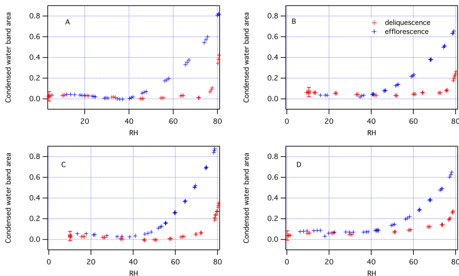
Figure 5. Deliquescence and efflorescence experiments on (\text{NH}_4)_2\text{SO}_4 /1,4-butanediol/water ternary mixtures of variable concentrations. (a): pure ammonium sulfate. Note, efflorescence at \sim 35\% RH and deliquescence at \sim 80\% RH. (b): 1 : 3 1,4-butanediol/ (\text{NH}_4)_2\text{SO}_4 . Note, efflorescence at 35–40 % RH and deliquescence at 80 % RH. (c): 1 : 2 1,4-butanediol/ (\text{NH}_4)_2\text{SO}_4 . Note, efflorescence at 35–40 % RH and deliquescence at 80 % RH. (d): 1 : 1 1,4-butanediol/ (\text{NH}_4)_2\text{SO}_4 . Note, efflorescence at 35–40 % RH and deliquescence at 80 % RH.
