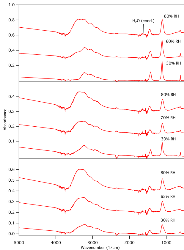
Figure 3. Spectra obtained after subtraction of gas-phase water features. Top panel: ammonium sulfate, middle panel: 1 : 1 (\text{NH}_4)_2\text{SO}_4 /1,2,6-hexanetriol (mixture by mass), bottom panel: 1 : 1 (\text{NH}_4)_2\text{SO}_4 /glycerol. Note the presence of a condensed-phase water feature at 1640\text{ cm}^{-1} (the HOH bend). This was used to quantify liquid water in the aerosol phase.
