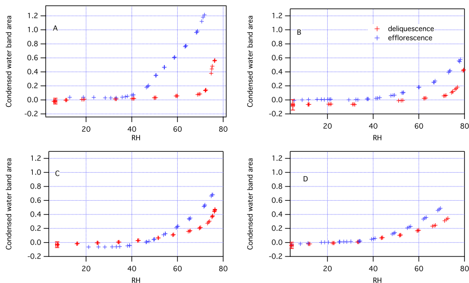
Figure 7. Deliquescence and efflorescence experiments on (\text{NH}_4)_2\text{SO}_4 /1,2,6-hexanetriol/water ternary mixtures of variable concentrations. (a): pure ammonium sulfate. Note, efflorescence at \sim 35\% RH, deliquescence at \sim 80\% RH. (b): 1 : 3 1,2,6-hexanetriol/ (\text{NH}_4)_2\text{SO}_4 . Note, efflorescence at 40% RH, deliquescence at 70–80% RH. (c): 1 : 2 1,2,6-hexanetriol/ (\text{NH}_4)_2\text{SO}_4 . Note, efflorescence at 40–50% RH, no clear deliquescence point. (d): 1 : 1 1,2,6-hexanetriol/ (\text{NH}_4)_2\text{SO}_4 . Note, no clear efflorescence or deliquescence points.
