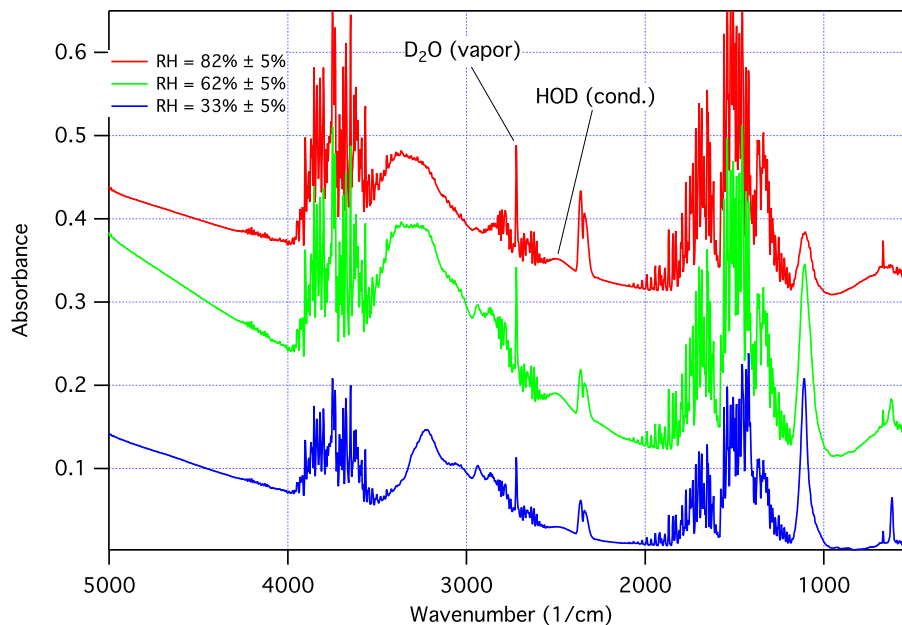
Figure 4. (\text{NH}_4)_2\text{SO}_4/1,2,6\text{-hexanetriol} solution exposed to \text{D}_2\text{O} at three different RH values. Note the presence of features related to \text{D}_2\text{O} : the \text{D}_2\text{O} vapor features at 2600\text{--}2800\text{ cm}^{-1} and the condensed HOD feature at 2500\text{ cm}^{-1} . HOD is present in all three spectra, indicating that gas-phase diffusion occurred despite phase separation. Note that the green spectrum, taken at 62% RH, has a higher aerosol concentration than the other cases, resulting in the enhanced scattering slope at higher wavenumbers.
