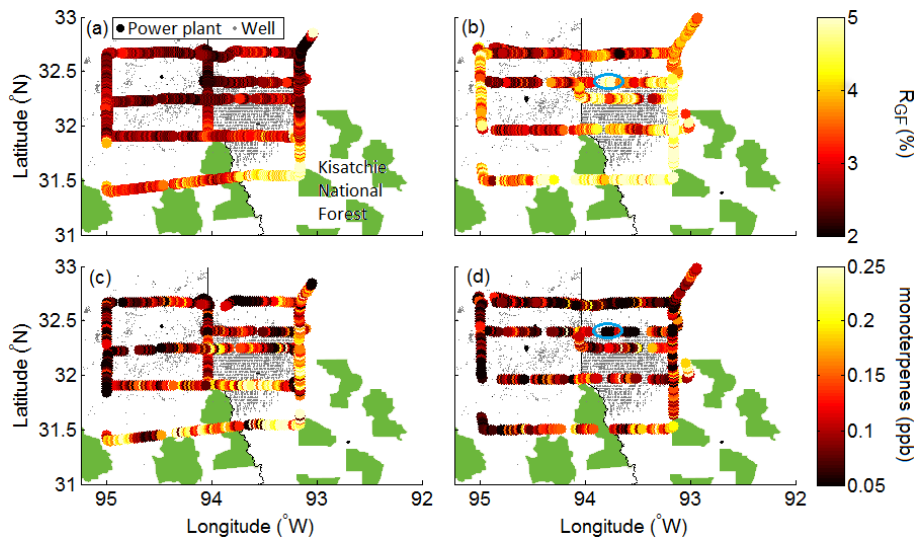
Figure 3. Flight tracks for 10 June ( a, c ) 25 June ( b, d ) over the Haynesville shale, colored by R_{GF} and the measured monoterpene mixing ratio. The southeast corner highlights high R_{GF} in a region with high monoterpene concentrations. The blue circle indicates the location of high R_{GF} discussed further in the text. Figure 5 shows meteorological and trace gas measurements acquired at this location. National parks are shown in green, and the Kisatchie National Forest is labeled in ( a ).
