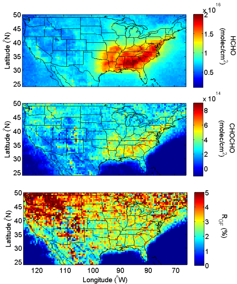
Figure 9. OMI Satellite retrievals of HCHO and CHOCHO vertical density during June through August of 2007. The ratio to CHOCHO to HCHO is shown in the bottom panel.
