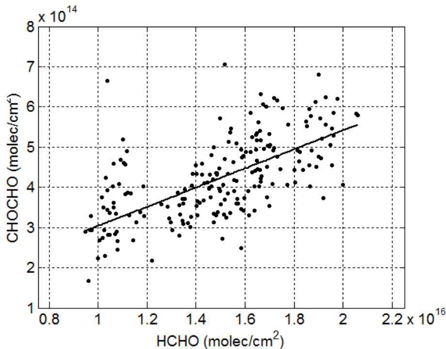
Figure 10. Satellite retrieval of CHOCHO v HCHOs corresponding to grid coordinates of SENEX boundary layer measurements. Statistics for the linear fits are shown in Table 4.
