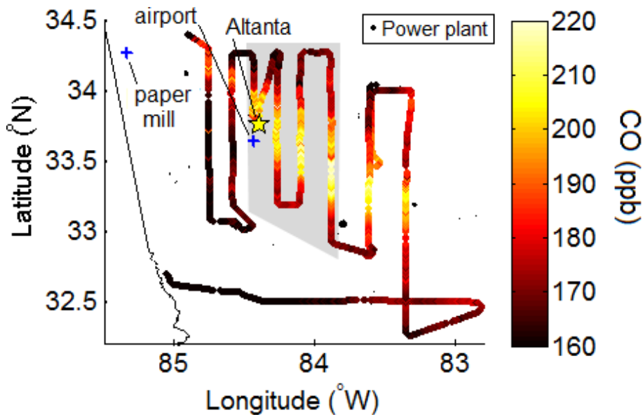
Figure 6. Flight track for 12 June colored by CO, which shows the combined outflow of Atlanta, the airport, and a paper mill on the surrounding background. Measurements acquired in the shaded area are shown in Fig. 7.
