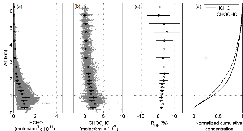
Figure 8. Average vertical profile of (a) HCHO and (b) CHOCHO measurements acquired during the flights specified in Fig. 1. Gray dots represent all measurements, black circles are averages in a given altitude bin, and error bars are SD within that bin. Bins are 200 m in height from 200 to 2500 m, and 500 m thereafter. (c) R_{GF} calculated from average OVOC profiles. Error bars are calculated from the SDs of HCHO and CHOCHO observations. (d) Cumulative concentration of HCHO and CHOCHO with altitude from 0–6 km, normalized to total column concentration.
