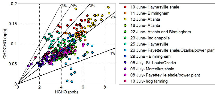
Figure 2. The relationship of CHOCHO and HCHO for each flight, gridded to OMI satellite resolution. Flights with extreme values of R_{GF} include those to the Haynesville shale (6/10 and 6/25) and the Ozarks (6/26).
