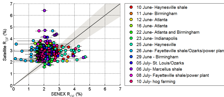
Figure 11. Satellite and SENEX R GF . The line represents a 1–1 relationship, error bars represent SDs of SENEX measurements within the given pixel, and the shaded area represents the accuracy of the SENEX measurements.
