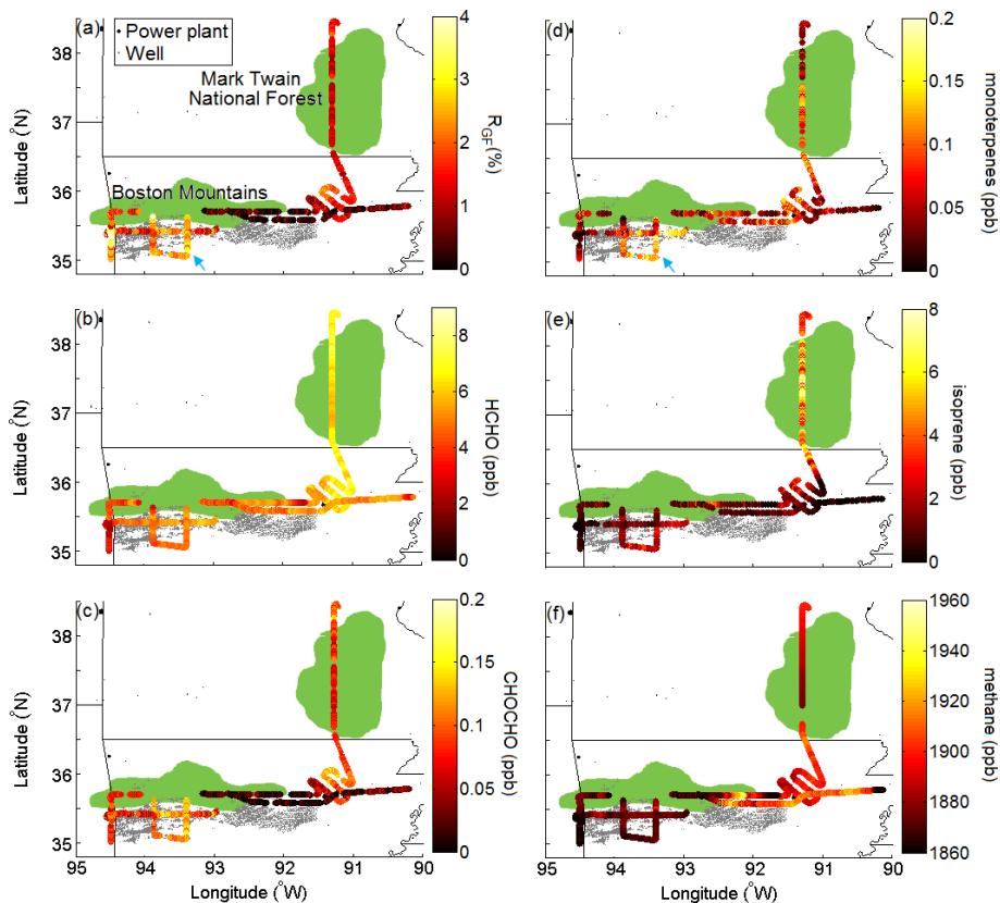
Figure 4. Flight track for the 26 June over the Fayetteville shale, the independence power plant, and the Ozarks, colored by the specified trace gas mixing ratio and R_{GF} . The blue arrow highlights the region of elevated monoterpene mixing ratios. National forests are shown in green.
